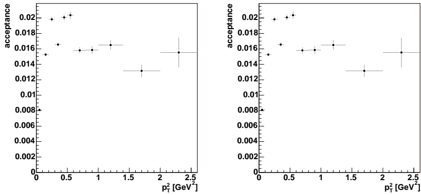
(a) \Xi acceptance.
