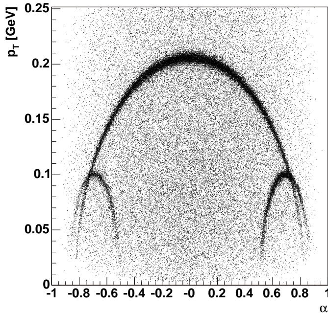
Figure 4.7: Armenteros-Podolansky plot for K_S^0 and \Lambda [ T^+53 ]. The transverse momentum is plotted against the longitudinal momentum asymmetry \alpha = (p_l^+ - p_l^-)/(p_l^+ + p_l^-) of the daughter tracks, both quantities were measured with respect to the mother particle track.
