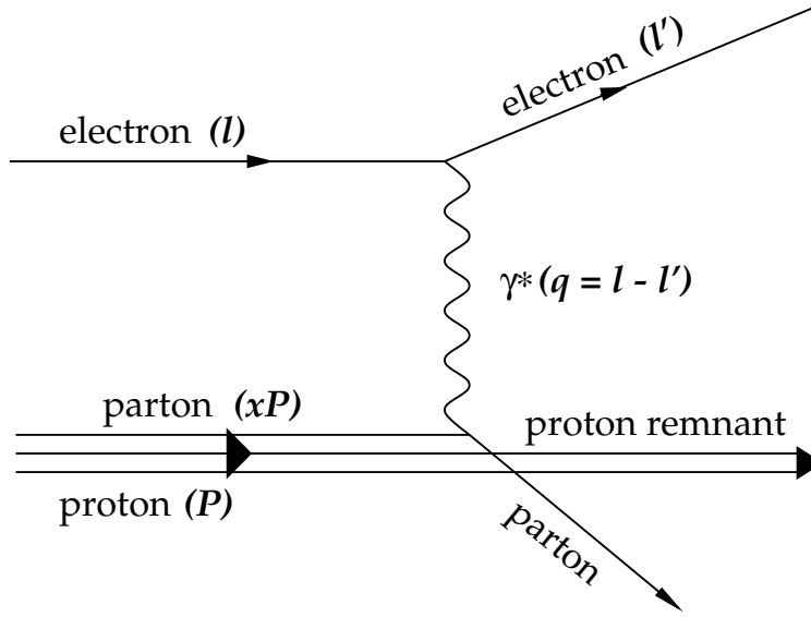
Figure 1.2: Deep inelastic ep scattering in the Quark Parton Model. Letters in braces denote particle four-momenta.
