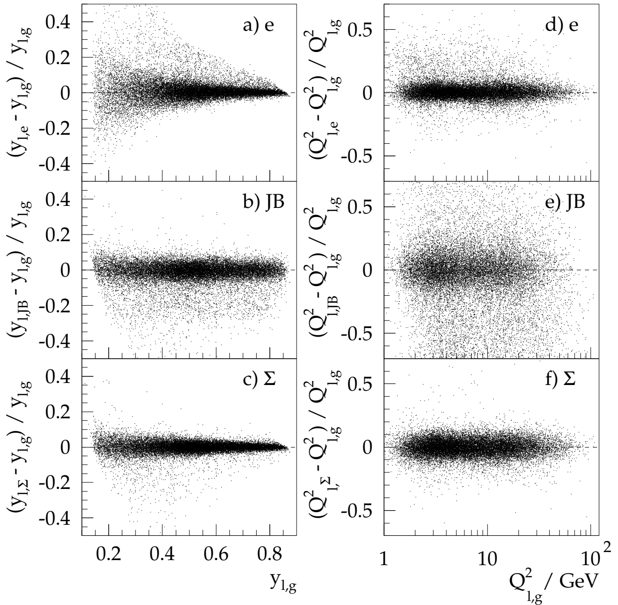
Figure 3.13: Resolution of leptonic variables y_l and Q_l^2 in simulated COMPTON events. The dots in the scatter plots show the relative deviation of the reconstructed quantity from its generated value as a function of the corresponding generated variable. The left plots demonstrate y_l resolution of a) electron, b) Jaquet – Blondel and c) Sigma method. The right plots show Q_l^2 resolution of these reconstruction methods: d) electron, e) Jaquet – Blondel and f) Sigma method. Only such events are displayed, in which a correct electron/photon identification on the basis of the simulated central tracker response has been performed.
