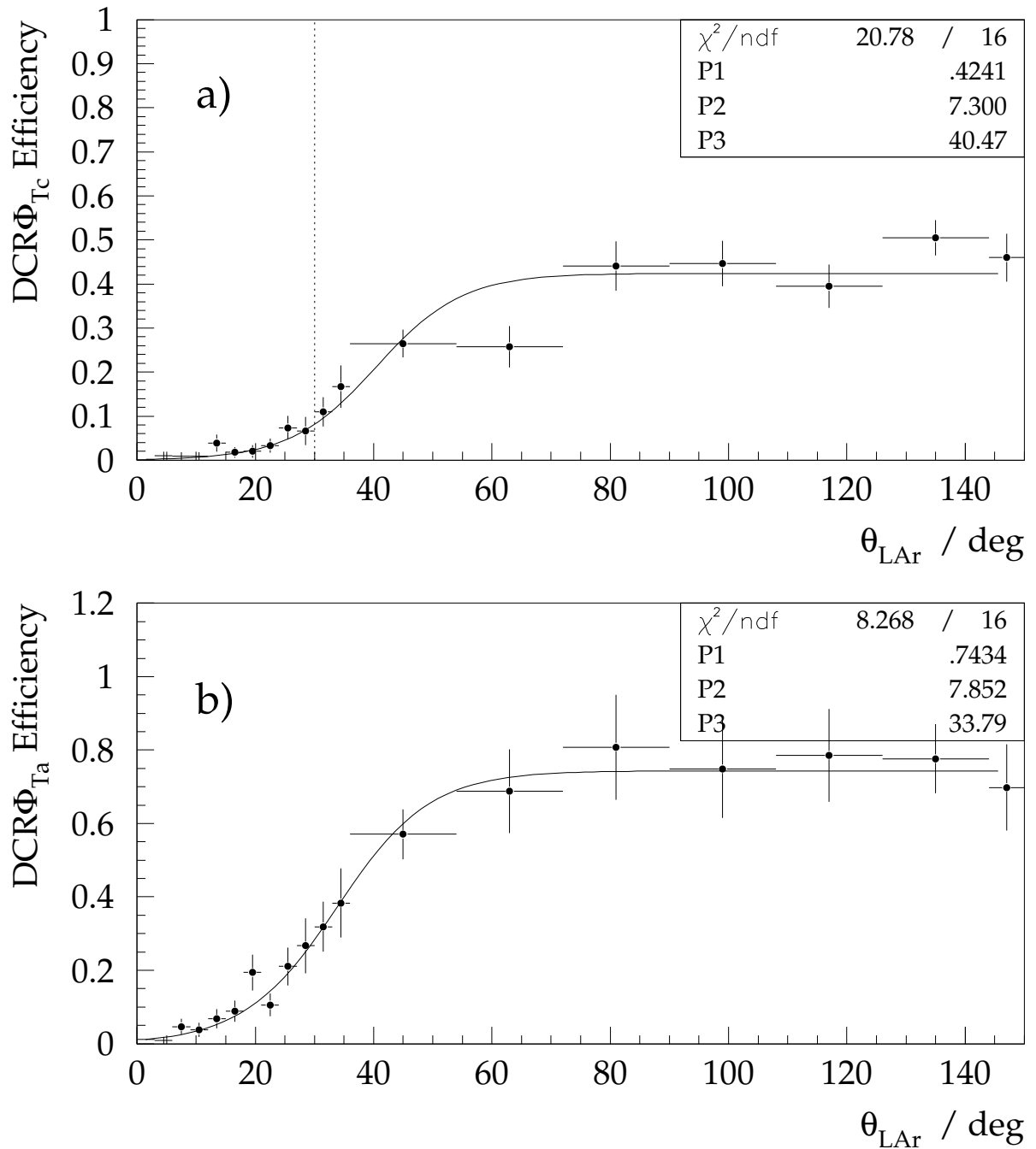
Figure 4.10: Efficiency of the DCRΦ trigger as a function of the LAr cluster maximum polar angle: a) DCRΦ Tc element, b) DCRΦ Ta element. The solid lines illustrate the fit functions given by eq. 4.16. The dashed line demonstrates the \theta_{\text{LAr}} cut applied in the analysis chain.
