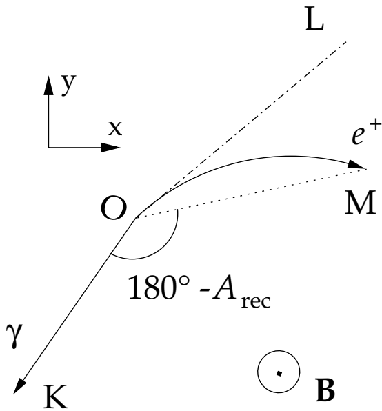
Figure 4.3: Influence of the magnetic field on the azimuthal angle of the scattered positron, which leads to a wrong acoplanarity reconstruction. The measured value is determined from the angle KOM, while the true value is given by the angle KOL. Here, K and M indicate the SpaCal clusters and O denotes the vertex position in the xy plane.
