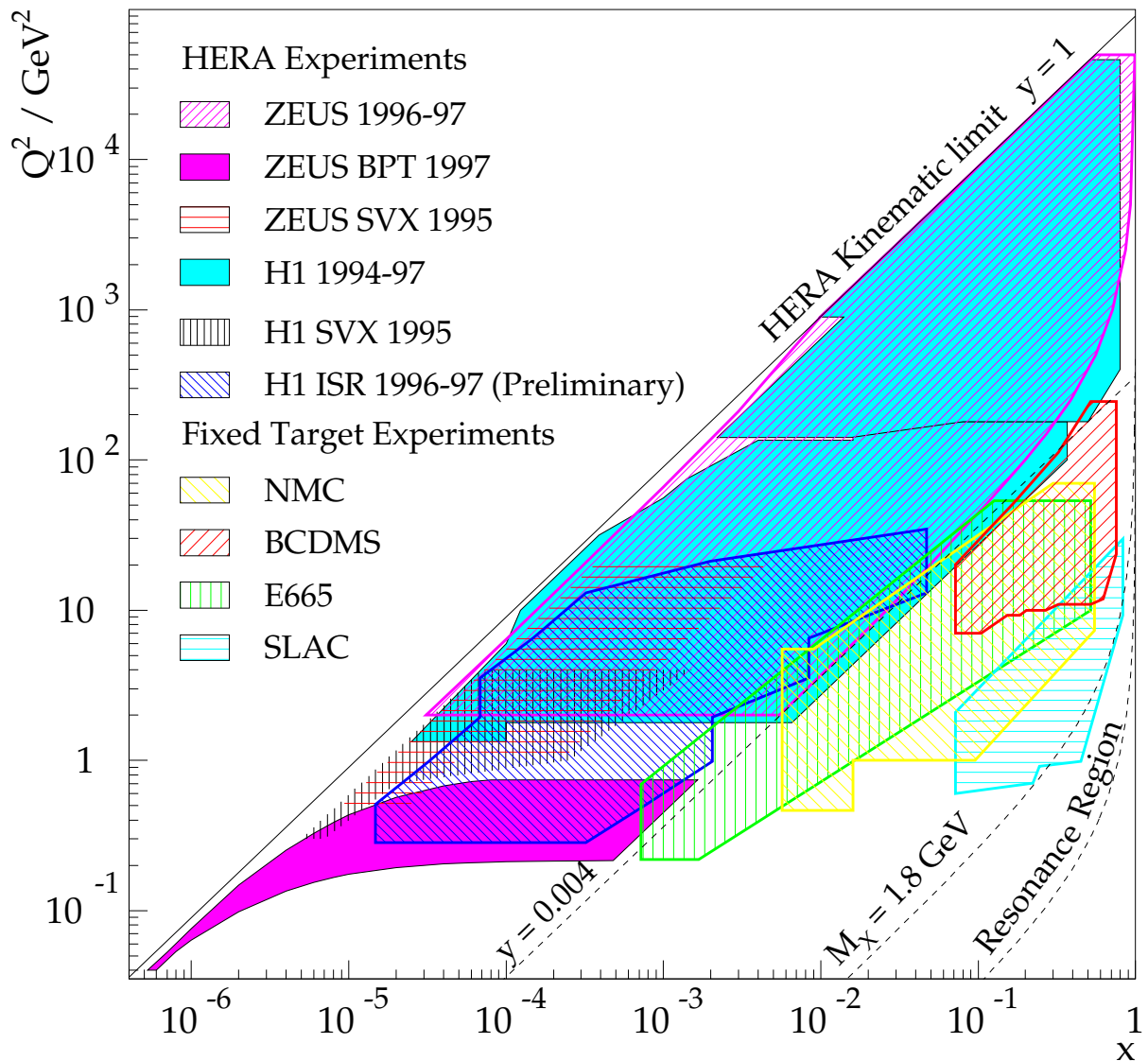
Figure 1.9: Kinematic regions of F_2 measurement in lepton-hadron experiments. Out of HERA results, the domains of H1 low [h100] and high Q^2 [h101], ZEUS standard [zeus01] and BPT [zbpt00], H1 [h197] and ZEUS [zeus96] shifted vertex, and H1 ISR [iiss01] measurements are drawn. The fixed target experiments shown are SLAC electron beam experiments [whi92], and CERN BCDMS [bcdms], NMC [nmc97] and FNAL E665 [e665] experiments on muon-nucleon scattering.
