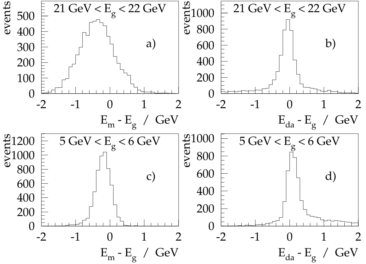
Figure 4.26: Figures a) and c) display the difference between the cluster energy and the generated energy in MC in two chosen bins of the generated energy. In figures b) and d) the double angle energy is used instead of the cluster energy.
