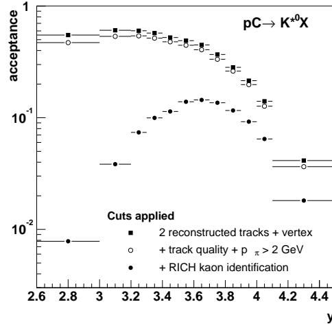
Figure 5.16: y acceptance as a function of the different analysis cuts. Again, this plot was made using the Monte-Carlo track matching method.
