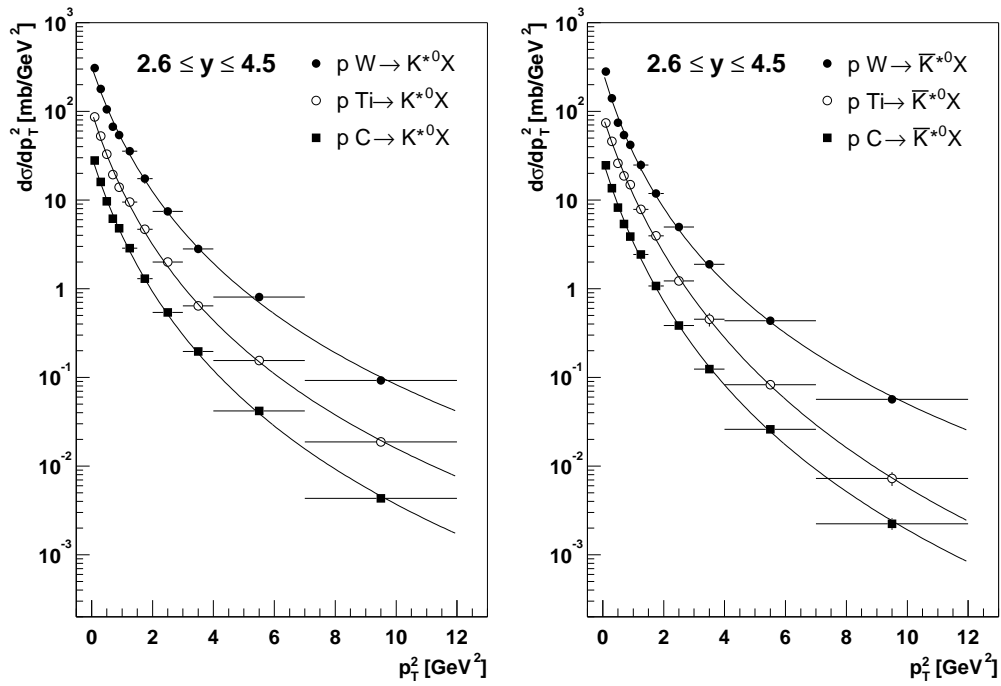
Figure 6.3: Transverse differential cross sections d\sigma/dp_T^2 for K^{*0} and \bar{K}^{*0} production at mid-rapidity. The cross sections are evaluated for 2.6 \leq y \leq 4.5 . Fits to the parameterization (6.5) are superimposed.
