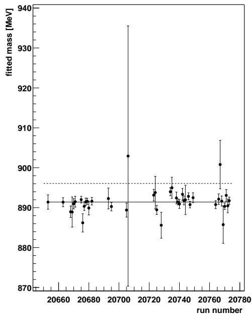
Figure 4.1: Fitted K^{*0} mass for each run. With respect to the nominal value (indicated by the dashed line) the mass is systematically shifted by about 5 MeV to lower values.
