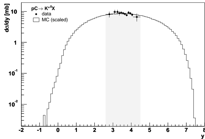
Figure 6.5: Illustration of the full phase space extrapolation of the K^{*0} production cross section. For the differential distribution shown the the experimental data cover 45 % of the total phase space.
