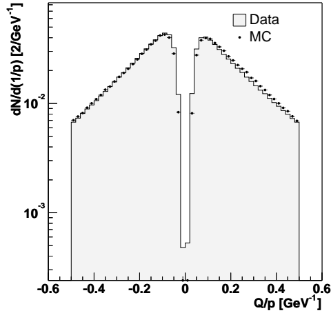
Figure 4.11: Q/p distribution for single tracks normalized to the same number of entries. The momentum cut at 2\text{ GeV} is clearly seen.
