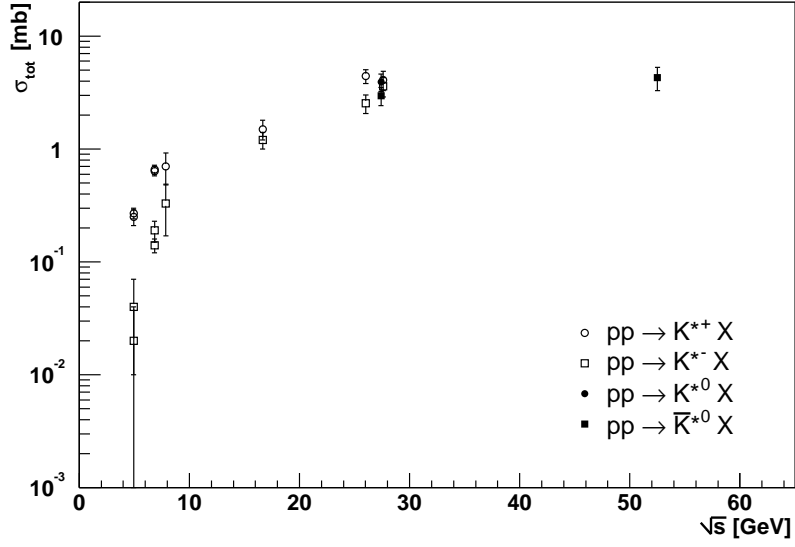
Figure 1.2: Measurements of the total K^* production cross sections in pp -collisions as a function of the center-of-mass energy \sqrt{s} [blo74, boc79, kic79, dri81, bri82, azi86, bog88, agu91]. The numbers are summarized in table 1.2.
