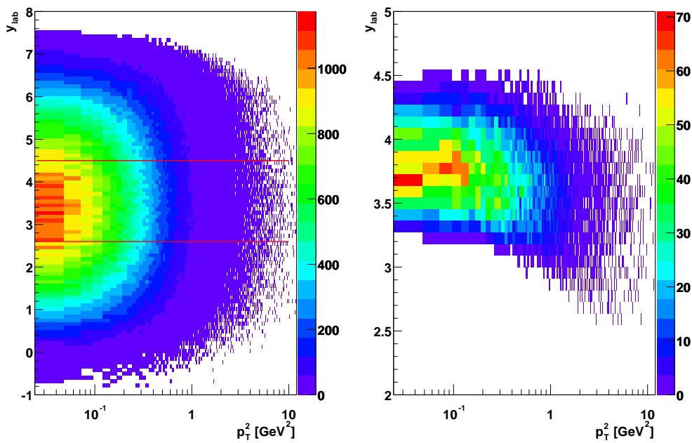
Figure 5.10: Monte-Carlo distributions of K^0 production in the p_T^2 - y plane. Left: Generator distribution showing the full phase space of the decay. The y -range accessible by HERA-B is indicated by the horizontal lines. Right: Distribution of reconstructed K^0 after application of all selection cuts. Clearly, rapidity and transverse momentum are not independent of each other any more.
