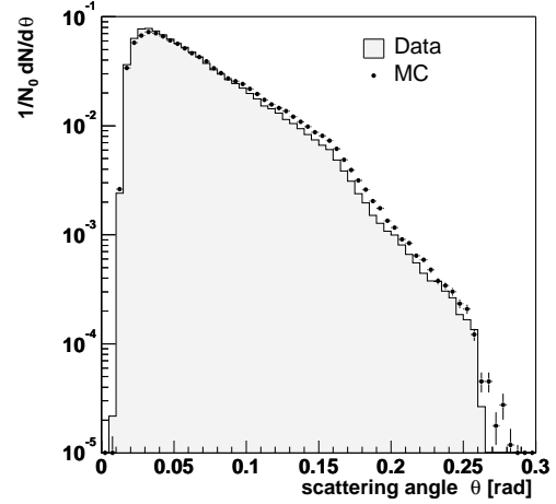
Figure 4.12: Comparison of the scattering angle \theta of single tracks measured in the laboratory system. The kink at \theta = 160\text{ mrad} is a result of the different acceptance limits in the horizontal and vertical plane.
