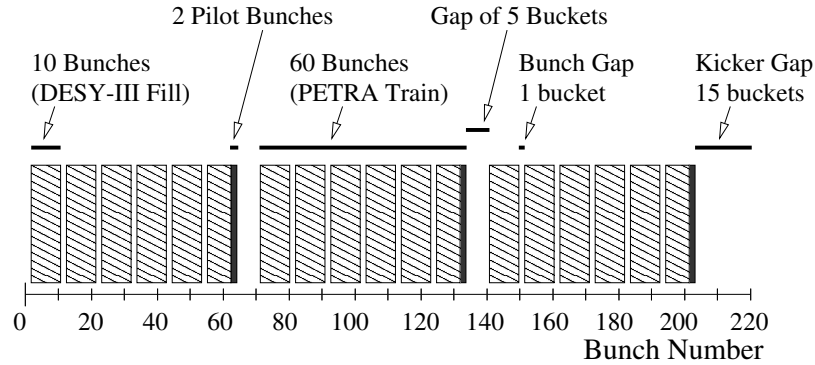
Figure 3.4: Filling scheme of the HERA proton beam, subdivided into three PETRA trains consisting of 6 DESY III trains of 10 bunches each. The pilot bunches at the end of each PETRA train do not have a colliding electron partner.
