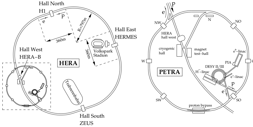
Figure 3.3: Schematic view of the HERA accelerator facility (left) and its pre-accelerator chain (right). The HERA-B experiment is located at Hall West on the DESY site.
