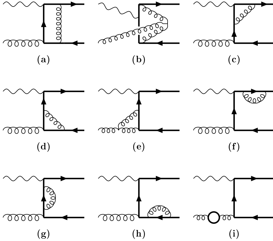
Figure 7.3: The NLO virtual corrections to \vec{\gamma}\vec{g} \rightarrow Q\bar{Q} . Reversing the heavy quark lines, except for the non-planar graph (b), yields the remaining graphs. Massless particle loops similar to graph (i) vanish, similarly to (3.3).
