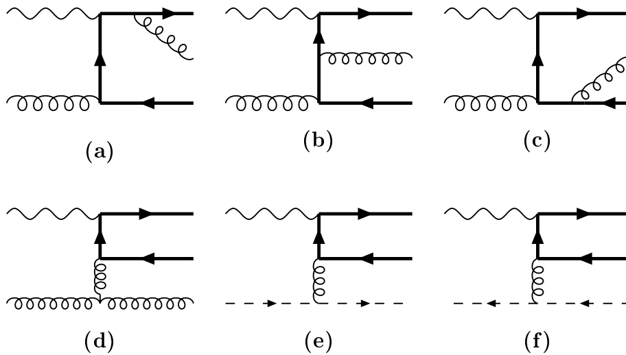
Figure 7.4: Feynman diagrams for the NLO gluon bremsstrahlung process \vec{\gamma}\vec{g} \rightarrow Q\bar{Q}g . Reversing the heavy quark lines yields the remaining graphs. In the unpolarized calculation the ghost contributions (e) and (f) have to be subtracted to cancel unphysical polarization contributions, see Fig. 2.1 and App. B.4.
