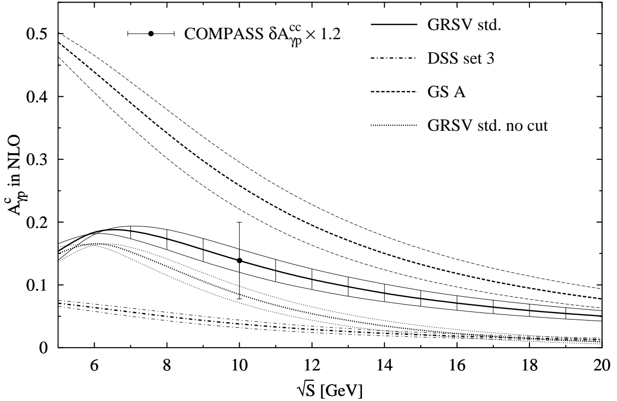
Figure 8.5: NLO anticharm photoproduction spin asymmetry A_{\gamma p}^{\bar{c}} with a cut p_T \leq 1.2 GeV using the GRSV standard, DSS set 3, and GS A polarized parton densities [15, 17, 18]. For the unpolarized cross section GRV'94 parton densities [62] were used. The thick lines have m_c = 1.5 GeV, the upper thin lines have m_c = 1.4 GeV, and the lower ones have m_c = 1.6 GeV (order reverses at \sqrt{S} \lesssim 6 GeV for GRSV standard). The GRSV standard curves are connected to form a band. We have set \mu_r^2 = \mu_f^2 = 2.25(m_c^2 + p_T^2) . GRSV standard curves without p_T -cut and the expected error at COMPASS [31], see text, are also shown.
