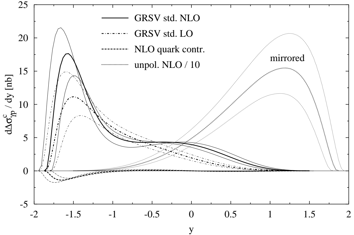
Figure 8.8: y -differential polarized anticharm photoproduction cross section d\Delta\sigma_{\gamma p}^c/dy in LO and NLO at \sqrt{S} = 10 \text{ GeV} with the GRSV standard densities [15] as measured in the hCMS. The thick lines have m_c = 1.5 \text{ GeV} , the thin lines with largest positive peak have m_c = 1.4 \text{ GeV} , and the ones with smallest positive peak have m_c = 1.6 \text{ GeV} . We have set \mu_r = \mu_f = 1.5m_c . The initial light quark contributions to the NLO curves are shown separately, for them the m_c = 1.4 \text{ GeV} curve has the largest negative peak and so on. For comparison analogous unpolarized curves with NLO GRV'94 densities [62] are shown divided by 10. They are also mirrored, i.e., we plot d\sigma(-y) .
