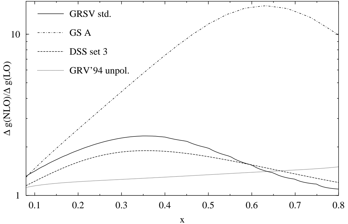
Figure 8.6: Ratios of NLO to LO polarized gluon distributions in the large x region. Shown is \Delta g(NLO)/\Delta g(LO) for the GRSV standard [15], DSS set 3 [17], and GS A [18] polarized parton densities. For comparison the ratio NLO to LO for the unpolarized GRV'94 [62] parton densities is also shown.
