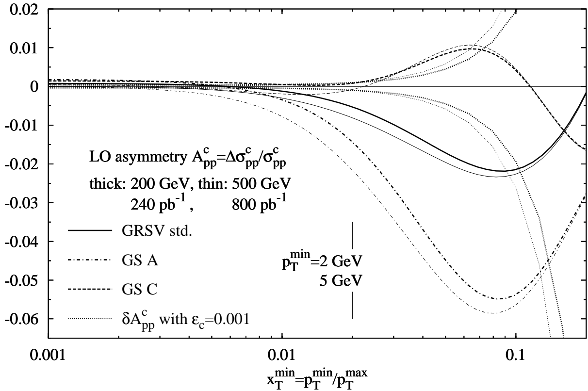
Figure 2.5: Total LO charm spin asymmetry at RHIC [32] for \sqrt{S} = 200, 500 GeV (thick, thin lines) for different polarized parton sets [15, 18] and the unpolarized GRV'94 densities [62], plotted as function of x_T^{\min} . This means varying the p_T -cut p_T \geq p_T^{\min} , where x_T^{\min} = p_T^{\min}/p_T^{\max} . For illustration the two p_T^{\min} values corresponding to x_T^{\min} = 0.02 and \sqrt{S} = 200 and 500 GeV, respectively, are inserted. An estimate of \pm \delta A_{pp}^c according to (2.31) is also shown.
