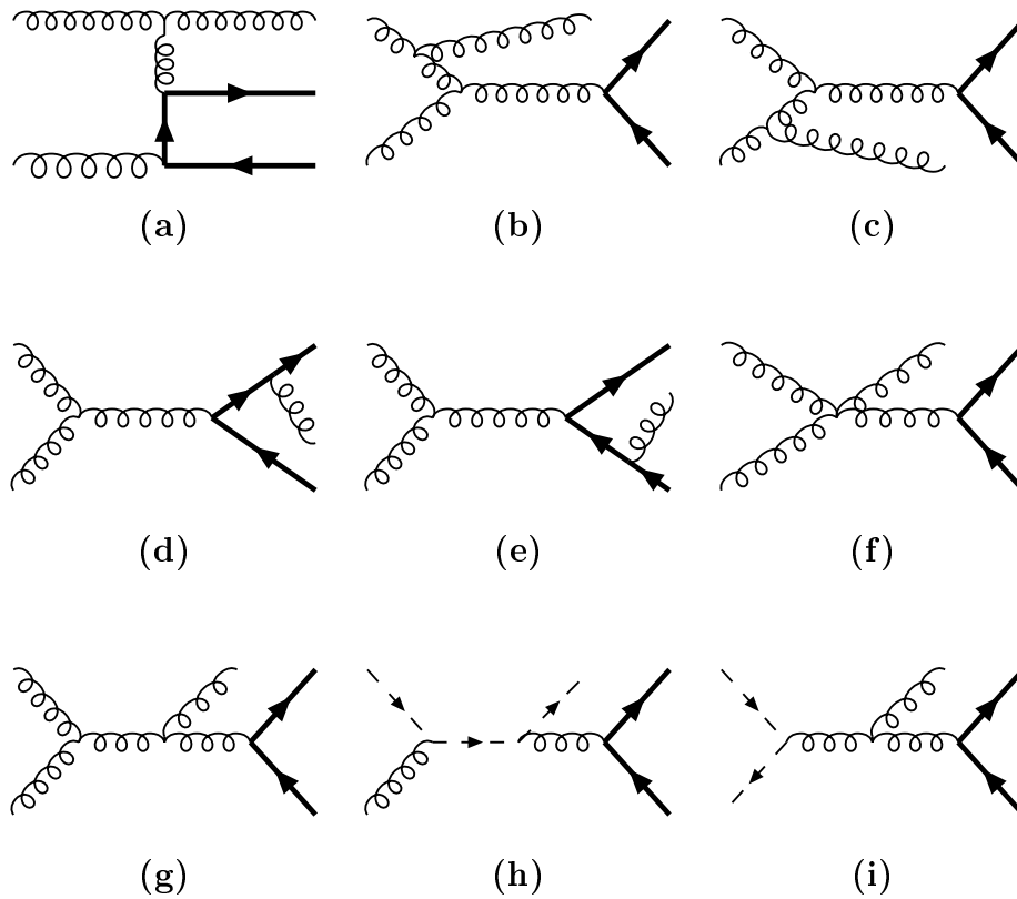
Figure 7.17: Feynman diagrams for the NLO gluon bremsstrahlung process \vec{g}\vec{g} \rightarrow Q\bar{Q}g . Replacing the photon by a gluon in Fig. 7.4 and reversing the heavy quark lines of (a) yields the remaining graphs. Many initial to final or initial to initial ghost contributions, for example (h) and (i), have to be subtracted in the unpolarized case to cancel unphysical polarization contributions, compare Fig. 2.1 and App. B.4.
