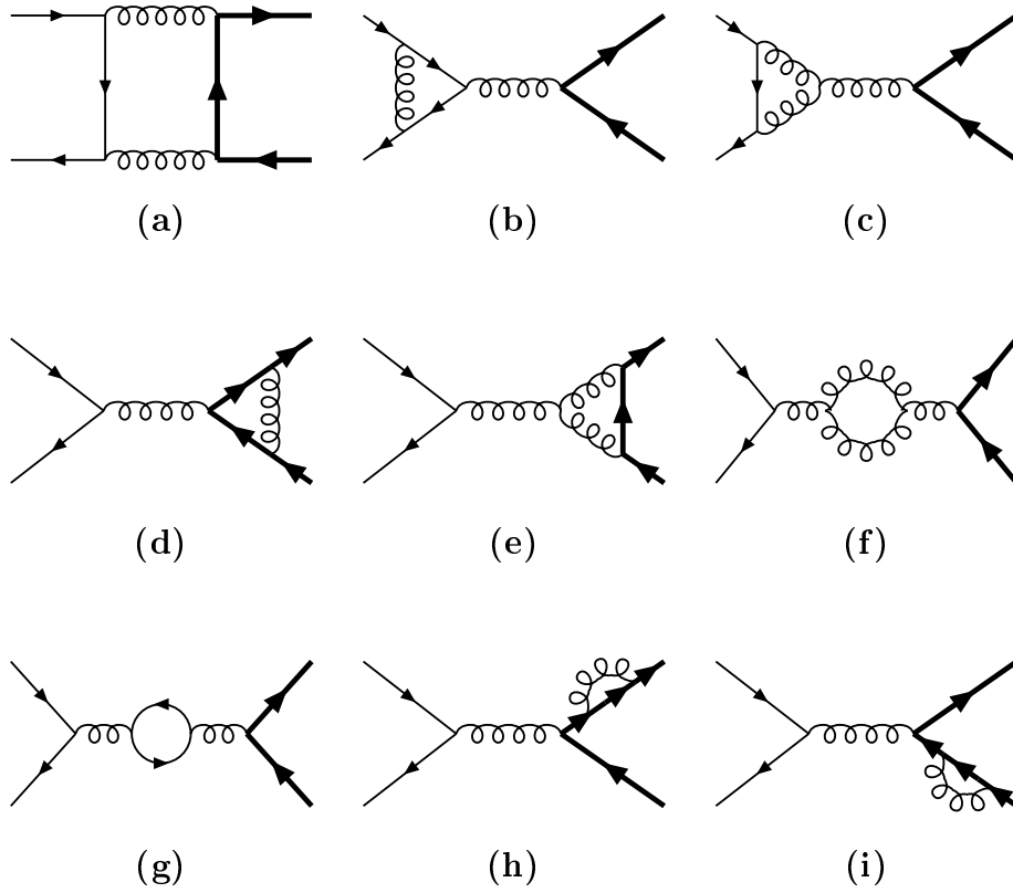
Figure 7.12: The NLO virtual corrections to \vec{q} \vec{q} \rightarrow Q \bar{Q} . There are two additional diagrams, one is obtained from reversing the heavy quark lines of graph (a), the other from replacing the gluon loop of graph (f) by a ghost loop. The quark loop of graph (g) has to be computed for massless and massive quarks. Vanishing light quark self-energy loops on the incoming lines, see (3.3), are not shown.
