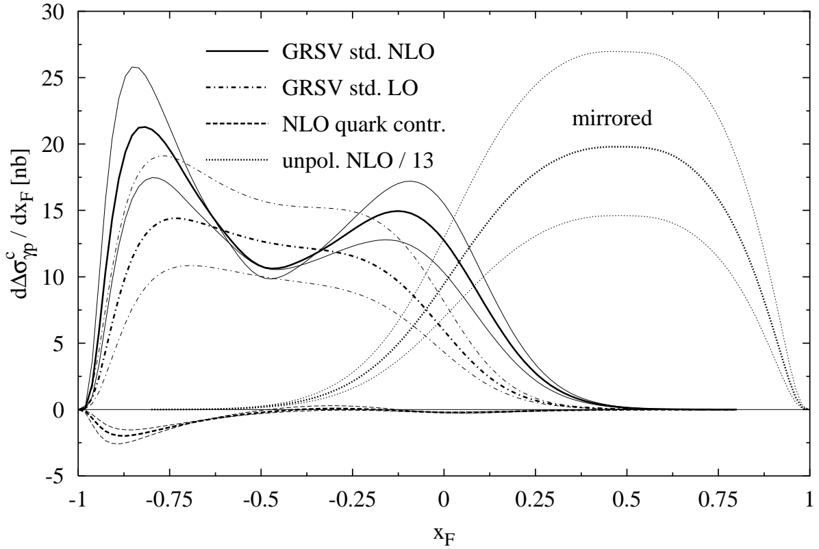
Figure 8.9: x_F -differential polarized anticharm photoproduction cross section d\Delta\sigma_{\gamma p}^c/dx_F in LO and NLO at \sqrt{S} = 10 GeV with the GRSV standard densities [15] as measured in the hCMS. The thick lines have m_c = 1.5 GeV, the thin lines with largest positive peak have m_c = 1.4 GeV, and the ones with smallest positive peak have m_c = 1.6 GeV. We have set \mu_r = \mu_f = 1.5m_c . The initial light quark contributions to the NLO curves are shown separately, for them the m_c = 1.4 GeV curve has the largest negative peak and so on. For comparison analogous unpolarized curves with NLO GRV'94 densities [62] are shown divided by 13. They are also mirrored, i.e., we plot d\sigma(-x_F) .
