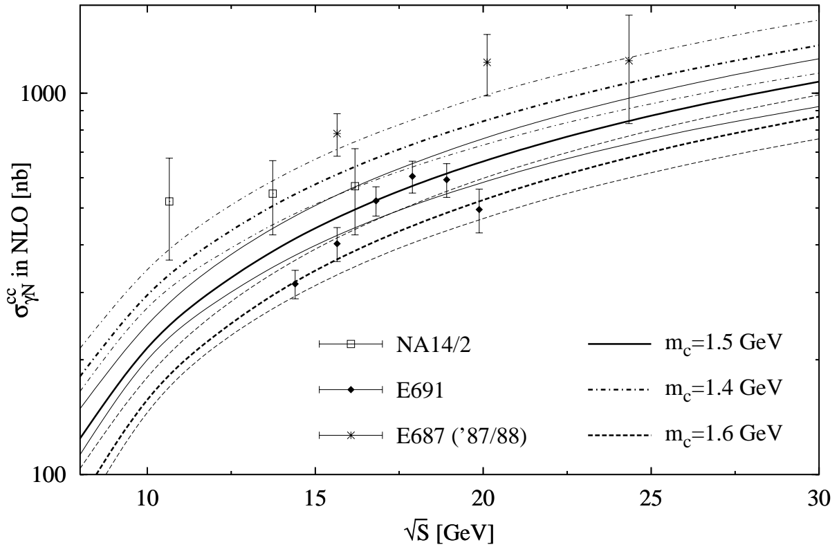
Figure 8.10: Unpolarized total charm-pair photoproduction cross section \sigma_{\gamma N}^{c\bar{c}} \simeq \sigma_{\gamma p}^{\bar{c}} compared with experimental data [105]. Predictions for the charm masses 1.4 GeV (dot-dashed lines), 1.5 GeV (solid lines), and 1.6 GeV (dashed lines) are shown, where the thick lines have \mu_r^2 = \mu_f^2 = 2.25m_c^2 and the thin lines are obtained by independent variations of \mu_{r,f}^2 by \pm 1.25m_c^2 . The GRV'94 unpolarized parton densities [62] were used.
