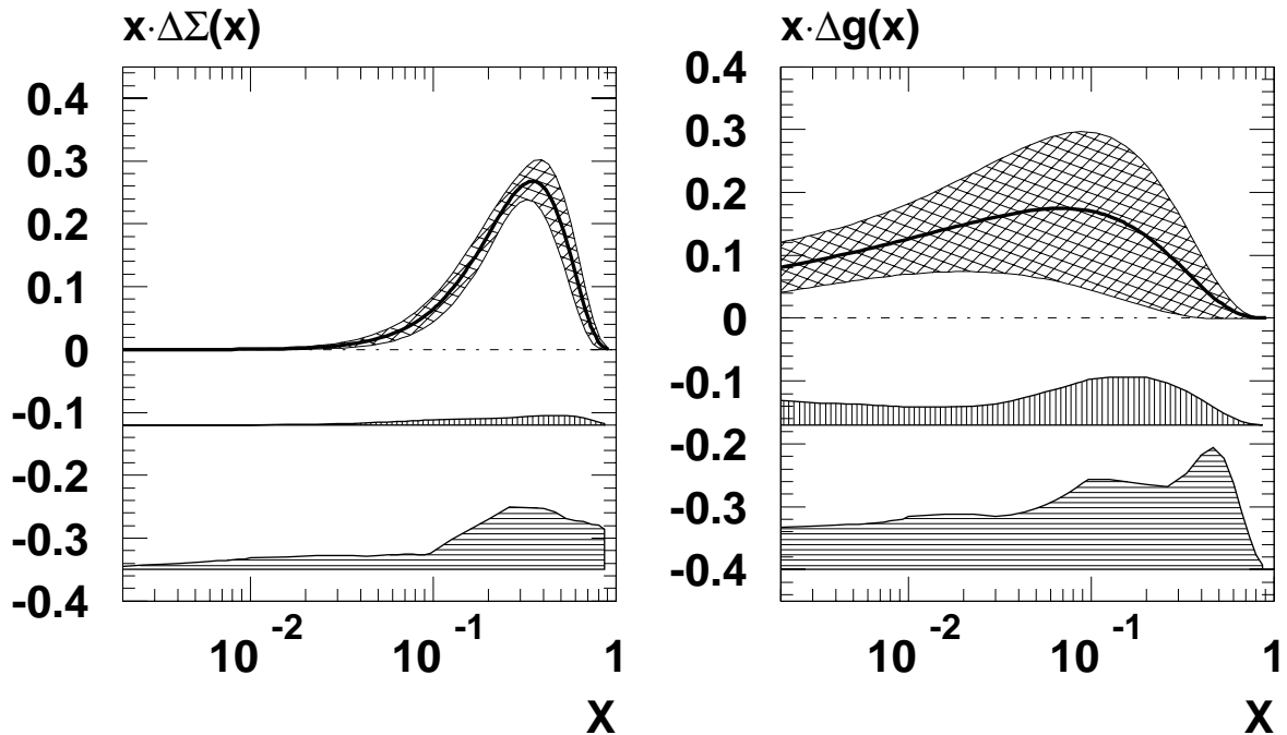
Figure 1.1: \Delta \Sigma and \Delta g uncertainties as obtained in the SMC fit [19]. Shown are the best fits (solid line) and the statistical (crossed hatch band), experimental systematic (vertically hatched), and theoretical (horizontally hatched) uncertainties as a function of x at the evolution starting scale \mu_{f0}^2 = 1\text{GeV}^2 . Note that the densities are obtained in the AB scheme [20], but \Delta g(x, \mu_f^2) remains unchanged by a scheme transformation to \overline{\text{MS}} . The figure shown here is part of Fig. 5 in [19].
