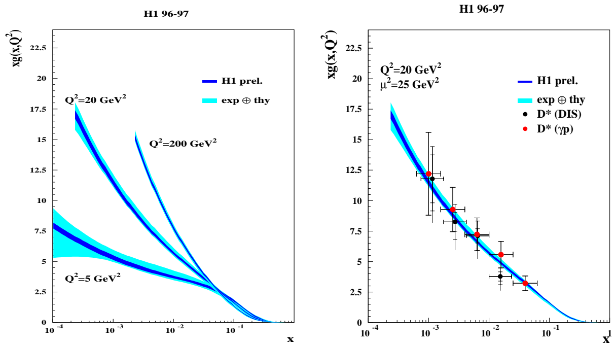
Figure 1.2: Uncertainty of the unpolarized gluon density g(x, \mu_f^2 = Q^2) from the H1 fit to scaling violations [21] (left) and comparison of this fit to the gluon unfolded from charm structure function DIS and photoproduction data for D^* [22] (right). The inner dark band of the gluon density shows experimental, the outer light band theoretical uncertainties. The figure shown here is Fig. 14 of [21].
