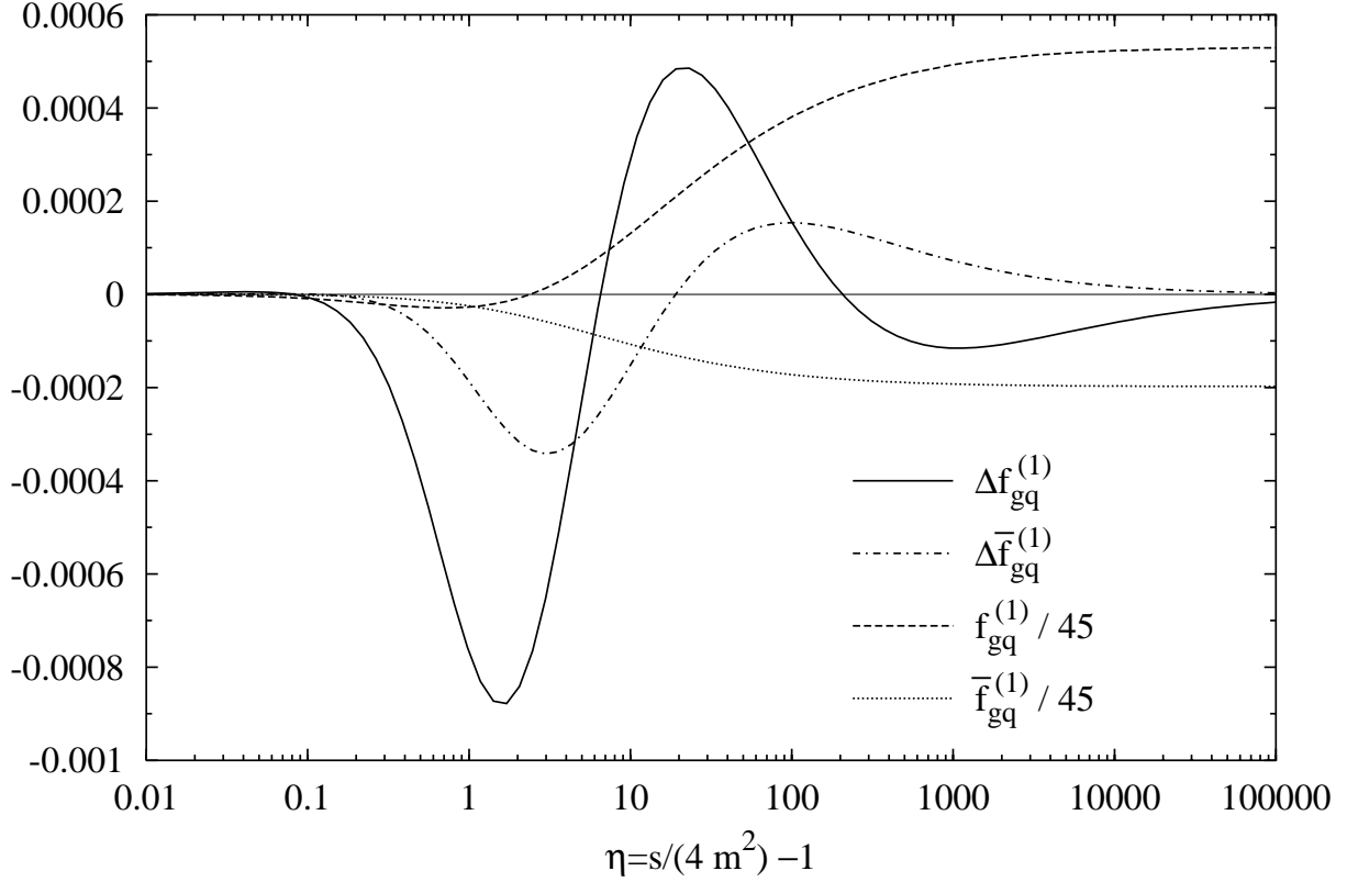
Figure 7.10: The NLO polarized and unpolarized scaling functions \tilde{f}_{gq}^{(1)} and \tilde{f}_{gq}^{-(1)} in the \overline{\text{MS}} scheme as function of \eta . The unpolarized scaling functions have been divided by 45.
