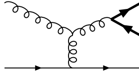
Figure 7.9: The only new Feynman diagram appearing in the \bar{g}q \rightarrow Q\bar{Q}q process. The others follow from Fig. 6.1 by replacing the photon by a gluon.
