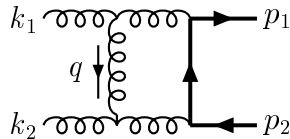
Figure 3.3: The hadroproduction box graph leading to the basic scalar integral (3.15).
