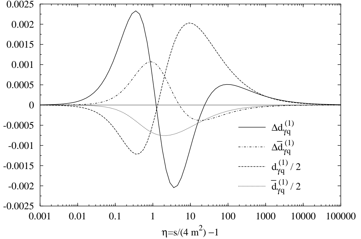
Figure 7.2: The NLO polarized and unpolarized “Compton” scaling functions \tilde{d}_{\gamma q}^{(1)} and \tilde{d}_{\gamma \bar{q}}^{(1)} in the \overline{\text{MS}} scheme as function of \eta as defined in (7.12). The unpolarized scaling functions have been divided by 2.
