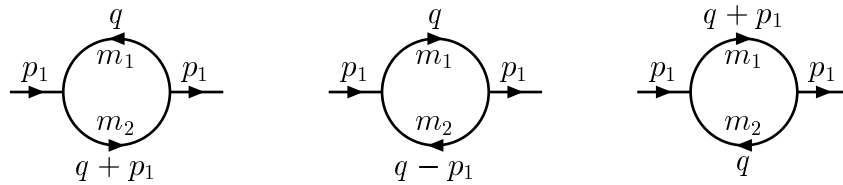
Figure 3.4: By assigning the loop momentum differently in one graph, it is shown that B_0(p_1, m_1, m_2) = B_0(-p_1, m_1, m_2) = B_0(p_1, m_2, m_1) .
