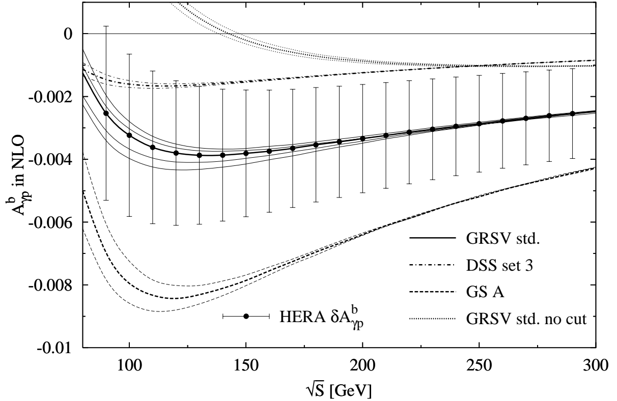
Figure 8.7: NLO antibottom photoproduction spin asymmetry A_{\gamma p}^{\bar{b}} with a cut p_T \geq 1.5 GeV using the GRSV standard, DSS set 3, and GS A polarized parton densities [15, 17, 18]. For the unpolarized cross section GRV'94 parton densities [62] were used. The thick lines have m_b = 4.5 GeV, the lower thin lines have m_b = 4.4 GeV, and the upper ones have m_b = 4.6 GeV. We have set \mu_r^2 = \mu_f^2 = 2.25(m_b^2 + p_T^2) . For GRSV standard varying \mu_r^2 and \mu_f^2 independently with a(m_b^2 + p_T^2) , m_b = 4.5 GeV, and a = 1, \dots, 3.5 yields the outer thin lines. GRSV standard curves without p_T -cut and points with the expected statistical error according to (8.20) are also shown.
