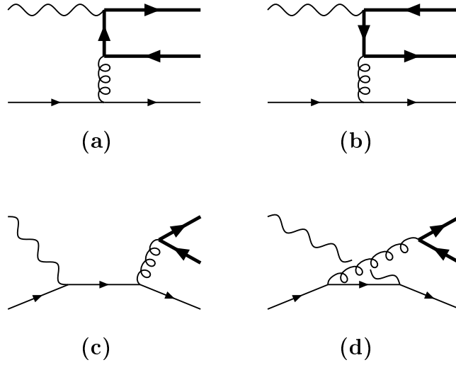
Figure 6.1: Feynman diagrams for the NLO light quark initiated subprocess \gamma q \rightarrow Q\bar{Q}q : “Bethe-Heitler” graphs (a) and (b), “Compton” graphs (c) and (d).
