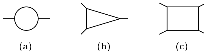
Figure 3.1: The topologies that can occur in the NLO virtual contributions: (a) self-energy, (b) vertex correction, and (c) box diagram. Note that the straight lines here can symbolize photons, gluons, ghosts, or quarks, as is appropriate.
