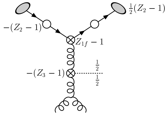
Figure 4.4: Effective counterterm contributions to be summed for the renormalization of the quark-gluon vertex. An example configuration is shown, where both quark lines are external and the gluon internal. The (crossed) circles indicate the contributions from Tab. 4.1, and the empty circle means mass renormalization with Z_m has been done previously. The gray ovals indicate the wave functions and the dotted line splits the internal contribution.
