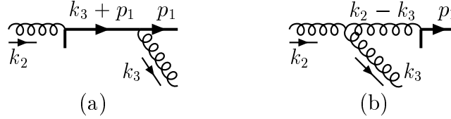
Figure 5.2: Two examples of 1 \rightarrow 2 sub-diagrams occurring in the real NLO graphs. The full 2 \rightarrow 3 process is decomposed in a 2 \rightarrow 2 process followed by a 1 \rightarrow 2 decay, examples of the latter are shown here.
