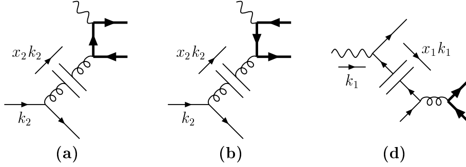
Figure 6.2: Factorized Feynman diagrams for obtaining the collinear contributions of Fig. 6.1. There is no factorized diagram corresponding to Fig. 6.1 (c).
