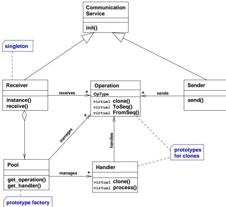
Fig. 6: The general architecture of the communication framework in UML notation.
