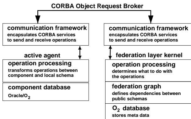
Fig. 2: The layers in the CORBA-based architecture of our prototype implementation.
