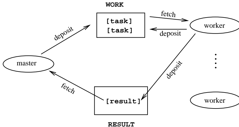
Figure 3: The coarse structure of the master-worker program for the parallel best-first search tree algorithm.
