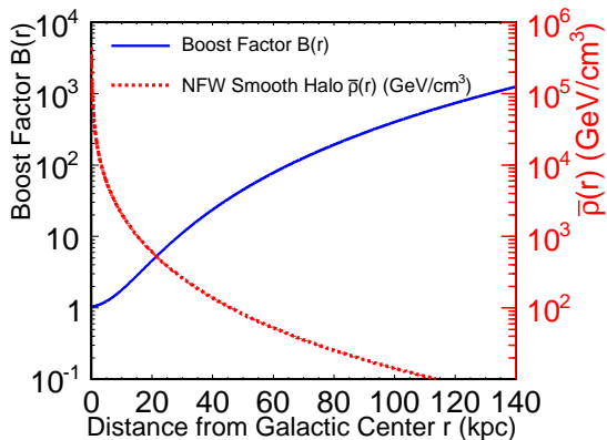
FIG. 11. Boost factor as function of the distance from the Galactic Center for the simplest model of [53] and a dark matter density using the NFW halo profile.
