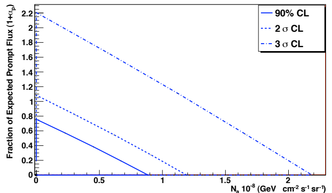
FIG. 9. Allowed regions for astrophysical muon neutrinos with an E^{-2} spectrum and prompt atmospheric neutrinos at 90%, 2\sigma , and 3\sigma confidence level. The lines indicate the boundary of the allowed region at the stated confidence level. The best fit point is indicated by the black dot at the origin.
