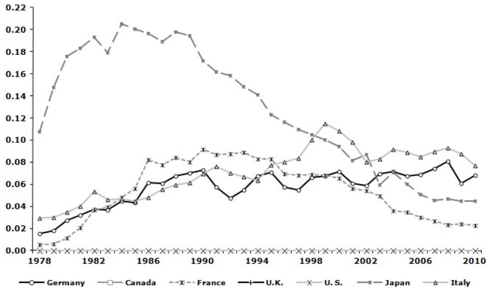
Figure 2: Gas-Specific Risks.
