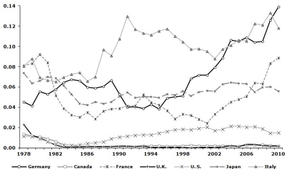
Figure 3: Oil-Specific Risks.
