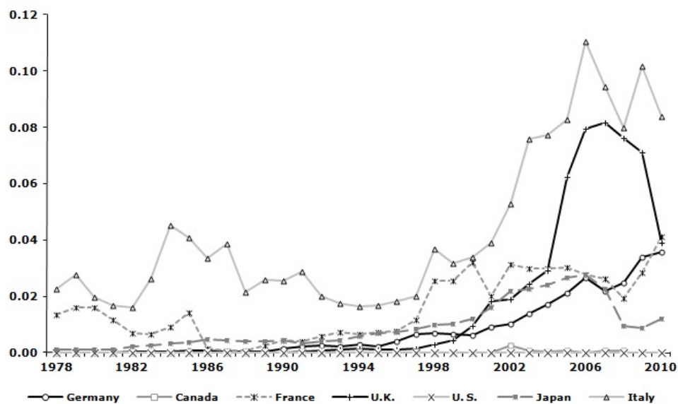
Figure 4: Hard-Coal-Specific Risks.
