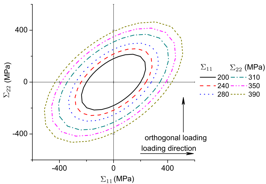
Figure 5.20.: Evolution of the yield surfaces as predicted by the extended Feigenbaum & Dafalias model for the Mg alloy AZ31, monotonic uniaxial tension test followed by monotonic uniaxial tension into the orthogonal direction
