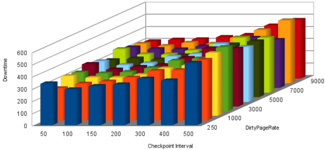
Figure 3: Effect of checkpoint intervals on service downtime in (ms)
