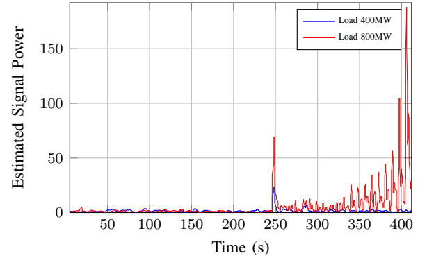
Fig. 7: ESPRIT based stability estimation at node 6
