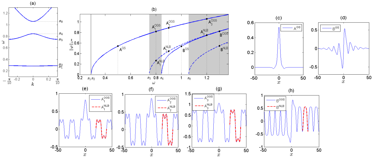
FIGURE 9. Panel (a): the band-structure for V(x) = \sin^2(\frac{\pi x}{10}) ; (b): a bifurcation diagram of GS and NLBs for (1.1) in 1D, \sigma = 1 . (c) and (d): plots of the GS at A^{\text{GS}} and B^{\text{GS}} resp.; (e)-(h): OGS and NLB at the remaining marked points.
