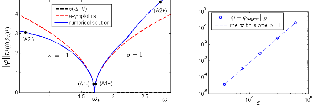
FIGURE 3. Left: Bifurcation diagram in the (\omega, \|\varphi\|_{L^2(\mathbb{P}^2)}) -plane for example A: N = 1 , k_* = (\frac{1}{2}, \frac{1}{2}) . Dashed lines: approximation \|\varphi\|_{L^2(\mathbb{P}^2)} \sim |A| \sqrt{(\omega - \omega_*)/\Omega} with \Omega = \sigma = \pm 1 . Curves bifurcating to the left/right of \omega_* are for \sigma = \mp 1 , respectively. The spectrum \sigma(-\Delta + V) is plotted on the horizontal axis. Right: Error for \sigma = -1 , where \varphi_{asympt} := \varepsilon A \xi_1(x, k_*) .
