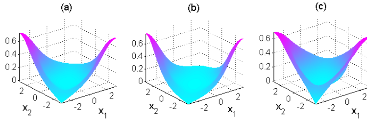
FIGURE 8. Nonlinear Bloch waves for example C. (a): the approximation \varepsilon \sum_{j=1}^2 A_j \xi_1(x, k_*^{(j)}) with \varepsilon = 0.516 ; (b) and (c): \varphi at (C-) and (C+) resp. in Fig. 7. In (b) \sigma = -1 and \omega = \omega_* - \varepsilon^2 \approx 1.31 and in (c) \sigma = 1 and \omega = \omega_* + \varepsilon^2 \approx 1.842 .
