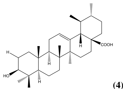
Figure 1: Isolated compounds: (1) \beta -Sitosterol, (2) Lupeol, (3) R=CH 3 , Betulinic acid - R=COOH, (4) Ursolic acid
