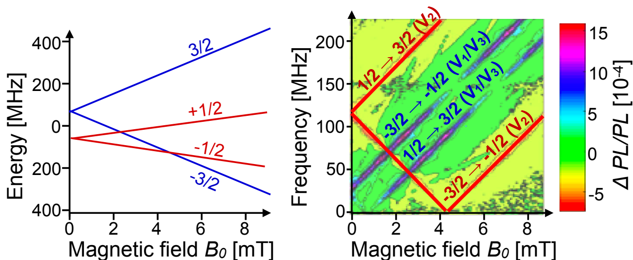
Figure 18. Left: Energy level system of the V_2 \text{Si}^- vacancy in SiC (6H polytype). Right: Experimental ODMR spectra as a function of the magnetic field (horizontal axis) and RF frequency (vertical axis). The experimental spectrum contains transitions from V_1 and V_3 vacancies. The color indicates the relative change in PL.
