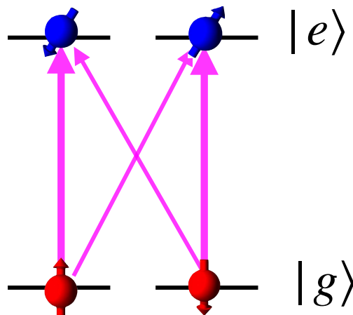
Figure 13. Eigenstates of the nuclear spin in the ground- and electronically excited states of a rare-earth ion. The quantization axes (indicated by the direction of the arrows) of ground- and excited state have different orientations, not along the magnetic field. The pink arrows between the ground- and excited states indicate optical transitions with the widths representing different transition dipole moments.
