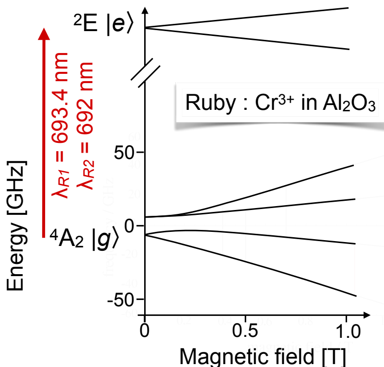
Figure 15. Partial energy level scheme of \text{Cr}^{3+} in Ruby.
