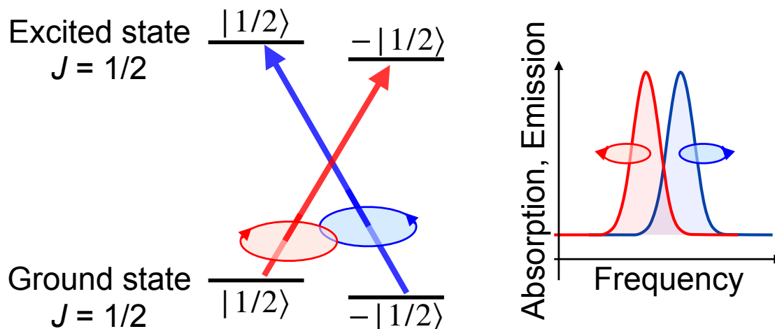
Figure 10. Energy level system and resonance lines of a Zeeman doublet.
