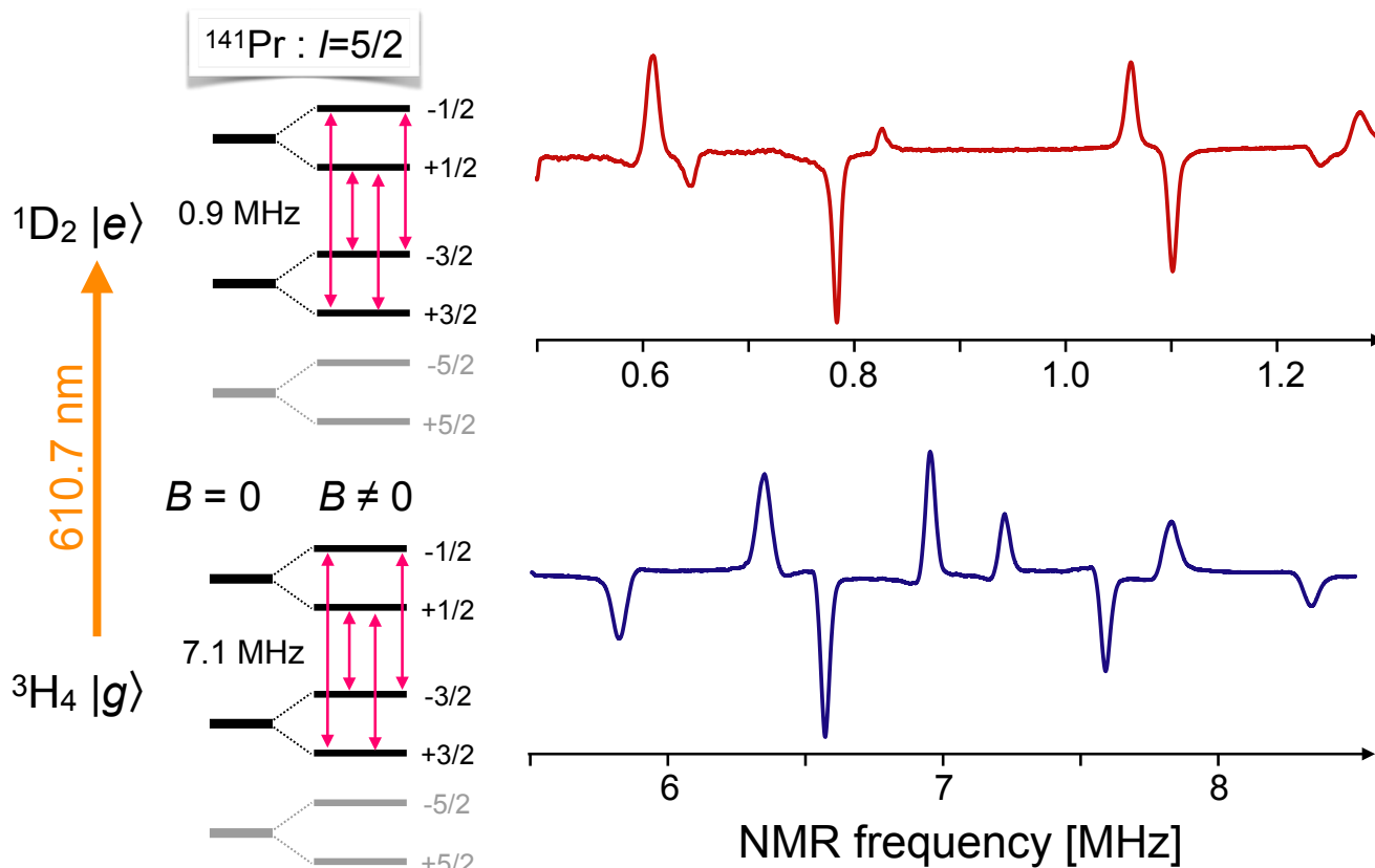
Figure 14. Energy levels and NMR spectra of ^{141}\text{Pr} in the ground- and electronically excited states of \text{Pr}^{3+} in an \text{YAlO}_3 host crystal, measured by coherent Raman scattering. The grey parts of the level scheme do not contribute to the spectra shown in the figure but are included for completeness. The four positive lines correspond to the transitions of one crystallographic site, as marked in the level scheme. The four negative lines belong to the corresponding transitions in a different crystallographic site.
