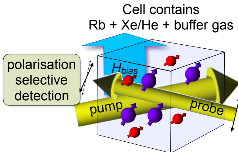
Figure 12. Setup for zero- and low-field NMR in an optical magnetometer based on alkali atomic vapor.
