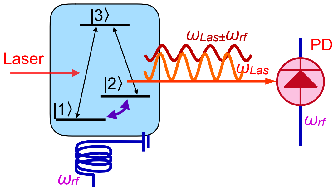
Figure 8. Basic principle of coherent Raman scattering.
