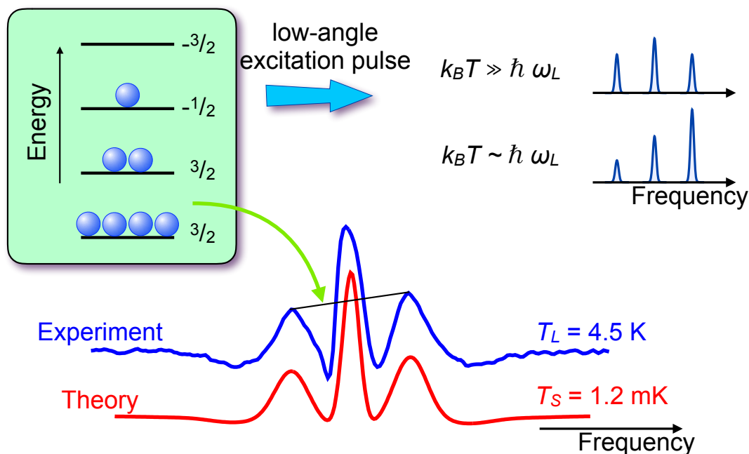
Figure 20. Experimental and simulated NMR spectra of ^{75}\text{As} in GaAs, measured with a small flip angle. The different amplitudes of the quadrupole satellites are then proportional to the population differences across the corresponding transitions and therefore allow a direct measurement of the spin temperature.
