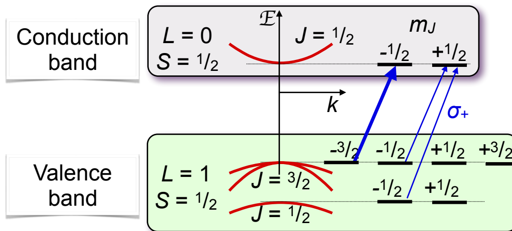
Figure 19. Optical pumping in a direct-band-gap semiconductor. The arrows mark the allowed optical transitions for circularly polarised light.
