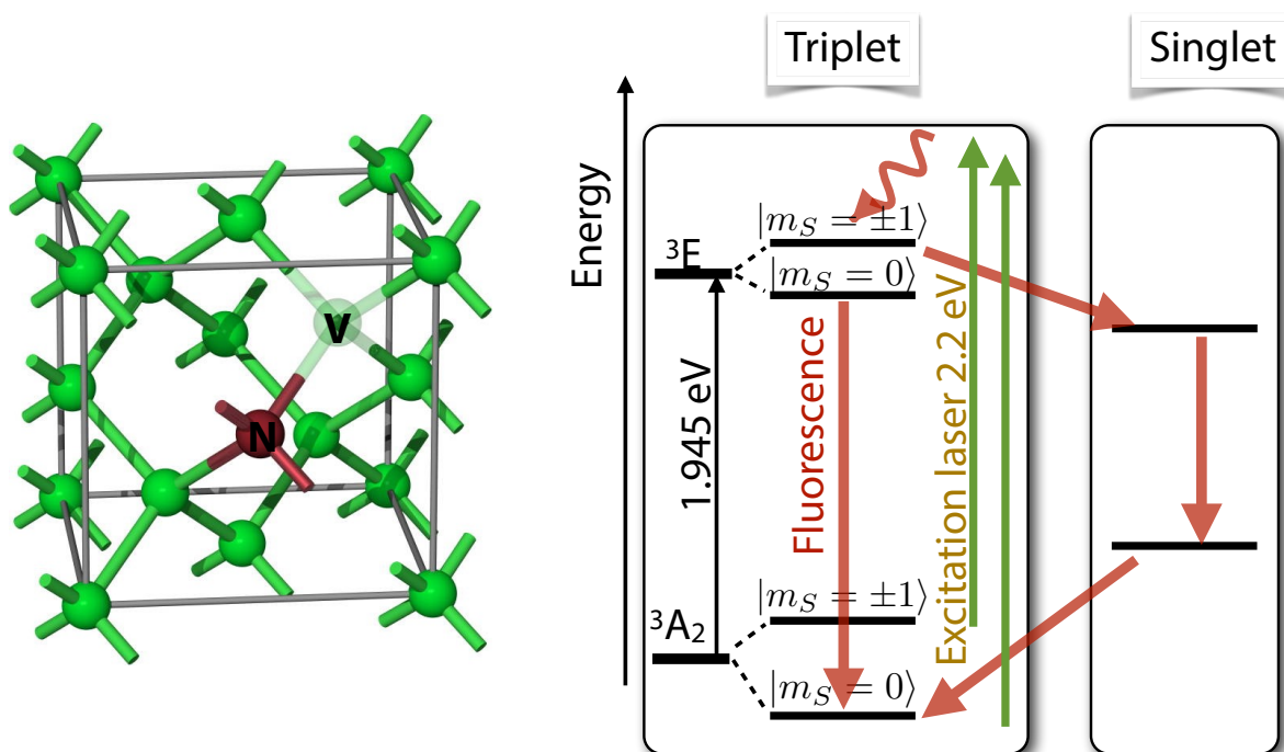
Figure 16. Structure of the nitrogen-vacancy (NV) defect center in diamond and energy level system. Optical excitation results in spin-dependent intersystem crossing (ISC) to the singlet state, which occurs predominantly for the m_S = \pm 1 states and therefore results in preferential population of the m_S = 0 state of the ^3A_2 ground state.
