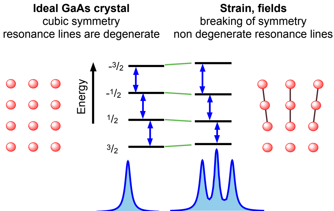
Figure 27. Spectra of I = 3/2 spins in ideal and distorted crystals.
