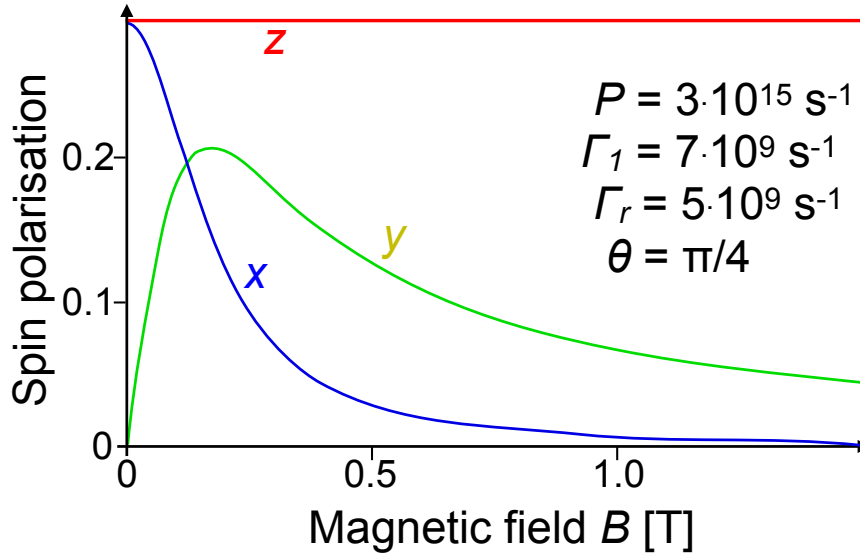
Figure 21. Polarization of the components of the electron spin in the conduction band as a function of the magnetic field B applied along the z -axis. The laser is incident in the xz -plane, at an angle of 45^\circ from the magnetic field. The remaining parameters are shown in the figure.
