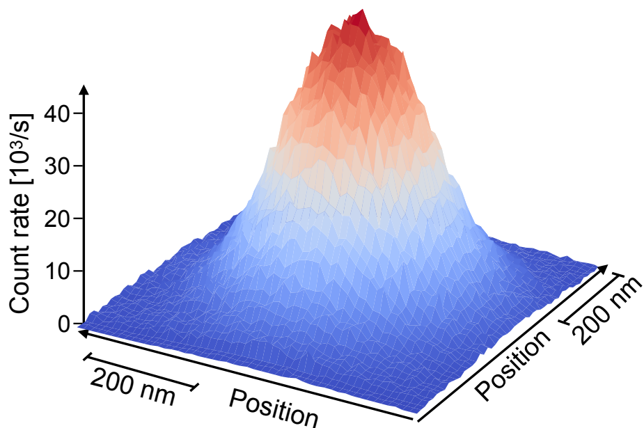
Figure 9. Photon count rate from a single NV center in diamond measured as a function of position.
