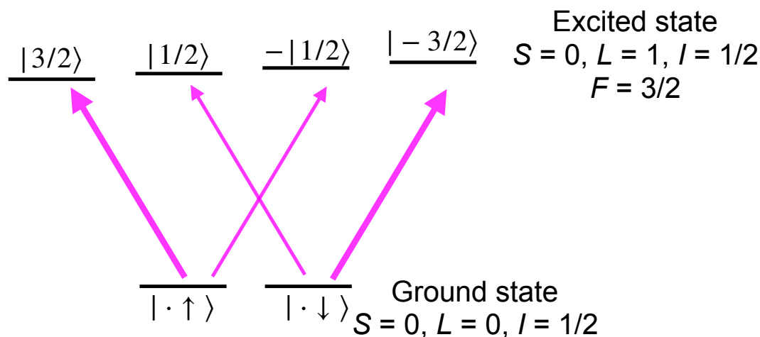
Figure 11. Detection of a nuclear spin state in a system with vanishing electron spin in the ground state. The transition strength of the thinner arrows is \sqrt{3}/3 \approx 0.58 times that of the thicker ones.
