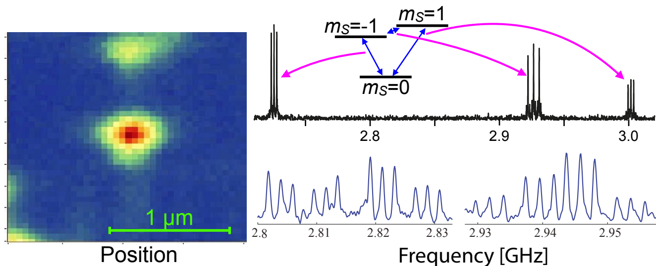
Figure 17. Left: scanning confocal image of a single NV center. Right: Optically detected ESR spectra of 2 different NV centers showing hyperfine interaction with the ^{14}\text{N} (top) and the ^{14}\text{N} plus a ^{13}\text{C} (bottom) nuclear spin.
