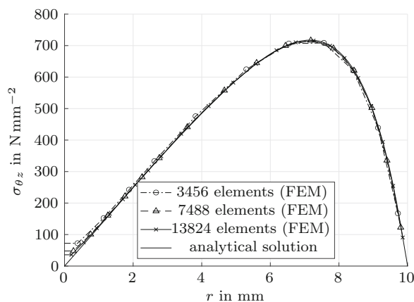
(b) torsion test, E = 210\,000 N/mm 2 , \nu = 0.3 , \ell = 1.0 mm
