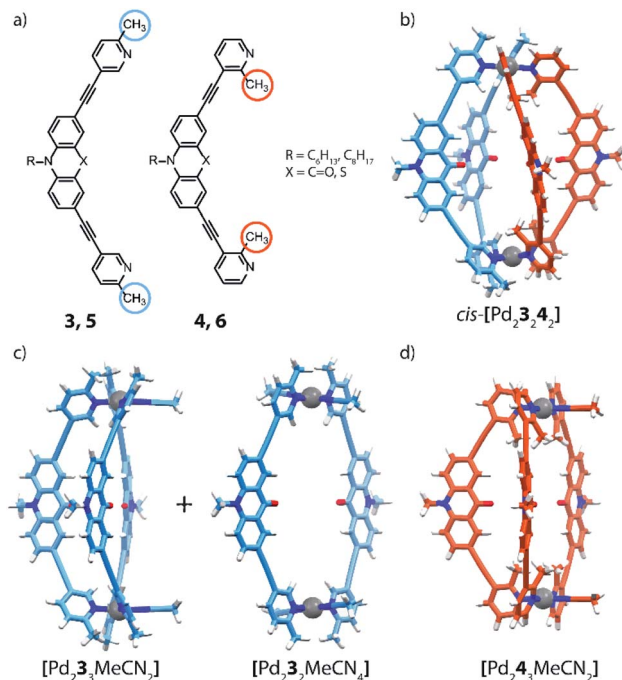
Fig. 5 (a) Banana-shaped ligands with outside- and inside-pointing methyl groups; (b) DFT model of heteroleptic cage cis -[Pd 2 L 2 L 2 ]; (c) DFT model of bowl and ring obtained with ligand 3 and (d) bowl obtained with ligand 4 .
