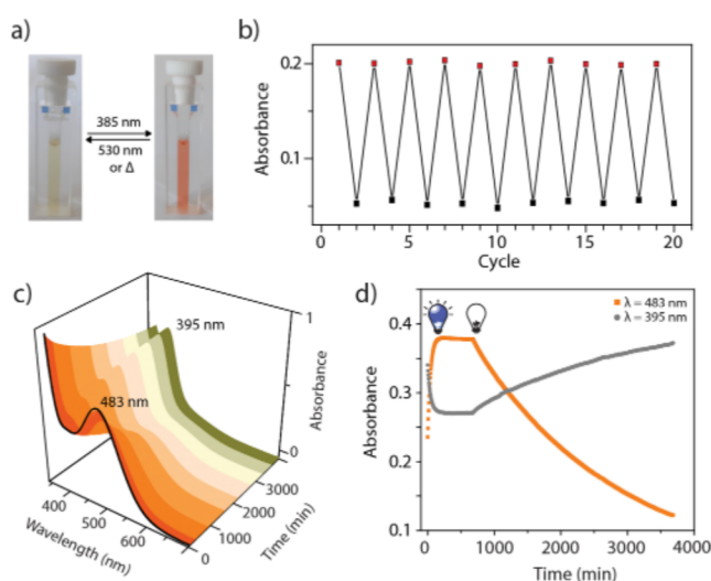
Figure 4. (a) Cage solution color change after irradiation (pale yellow: cis-Cage (+ higher assemblies), red: trans-Cage ); (b) fatigue experiment of structural interconversion upon irradiation with 385 and 530 nm in an alternating sequence; absorbance values measured at \lambda = 483 nm; (c) time-dependent UV–vis spectra showing thermal relaxation from the trans-Cage to cis-Cage mixture; (d) UV–vis monitoring of the system reaching the PSS and maintaining the out-of-equilibrium state ( trans-Cage ) with constant irradiation at 385 nm; turning off the light leads to thermal decay.
