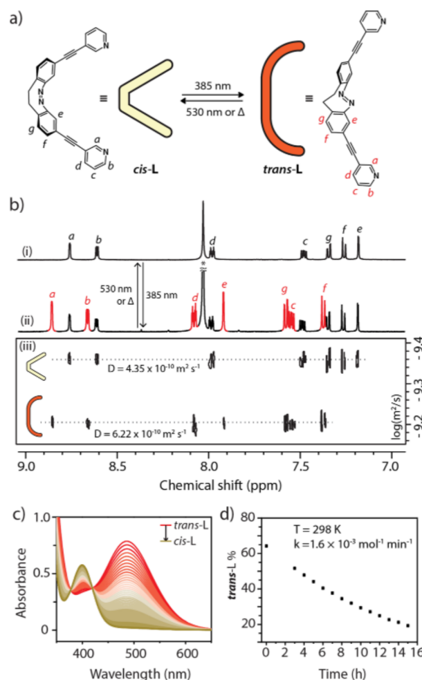
Figure 1. (a) Photoswitching between the two L isomers; (b) 1 H NMR (500 MHz, DMF- d 7 , 298 K) of (i) cis -L and (ii) the mixture of cis -L and trans -L after irradiation at 385 nm for 10 min, (iii) DOSY of the two ligand isomers; (c) absorption spectra showing the thermal relaxation from trans -L (red line) to cis -L (beige line) obtained every 30 min (DMF, 1.12 mM, 298 K); (d) kinetics of trans -L isomerization, monitored by 1 H NMR.
