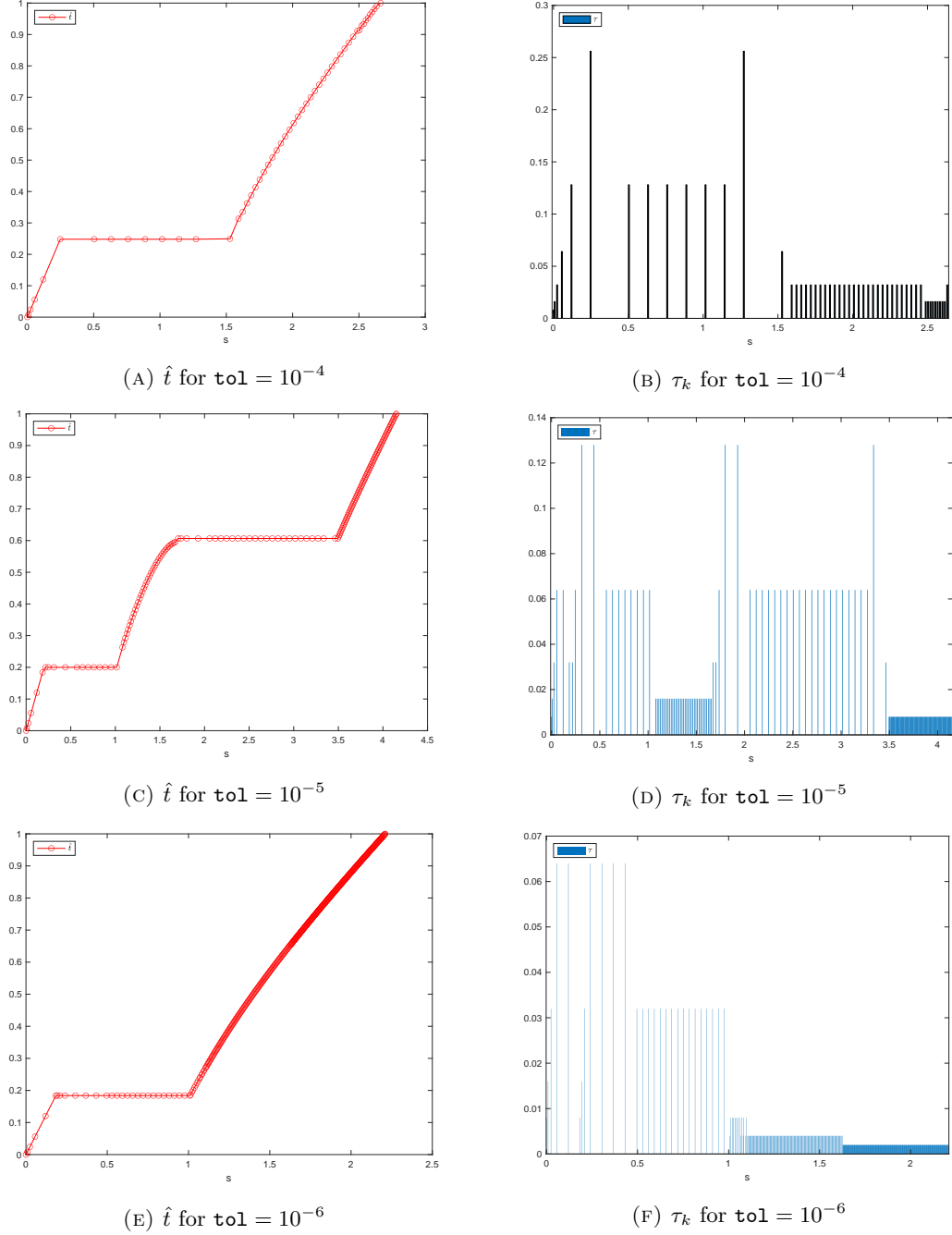
FIGURE 4. Physical time and step size for \text{tol} = 10^{-4} , \text{tol} = 10^{-5} and \text{tol} = 10^{-6} additional viscous jump is approximated than for the other tolerances. Note that, due to the
