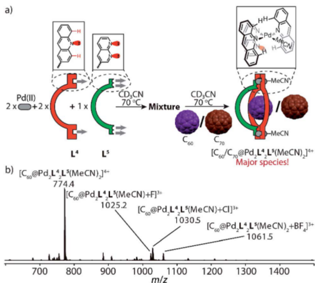
Fig. 6 Self-assembly of fullerene-containing heteroleptic bowl [\text{C}_{60}/\text{C}_{70}@\text{Pd}_2\text{L}^4_2\text{L}^5(\text{MeCN})_2]^+ : (a) ligands \text{L}^4 and \text{L}^5 react with \text{Pd}^{\text{II}} cations in a 2 : 1 : 2 ratio at 70 °C to give a convoluted mixture, followed by the addition of \text{C}_{60} or \text{C}_{70} to produce heteroleptic bowl [\text{C}_{60}/\text{C}_{70}@\text{Pd}_2\text{L}^4_2\text{L}^5_2] as major species; (b) high-resolution ESI mass spectrum of [\text{C}_{60}@\text{Pd}_2\text{L}^4_2\text{L}^5(\text{MeCN})_2]^+ and its anion adducts.
