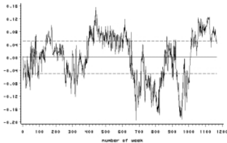
Figure 5: Cointegration regression residuals for 'Lufthansa' with boundaries of the 10% trading strategy
