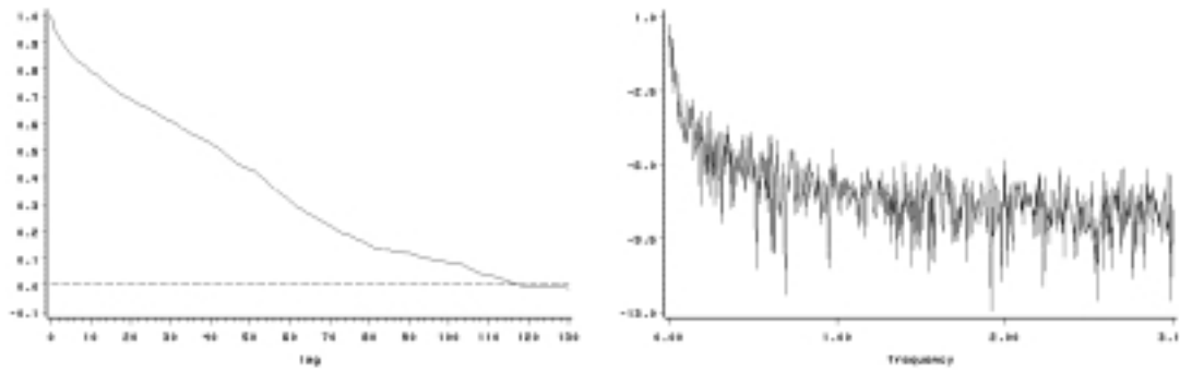
Figures 3 and 4: Autocorrelations and log-periodogram of 'Lufthansa' cointegration regression residuals
