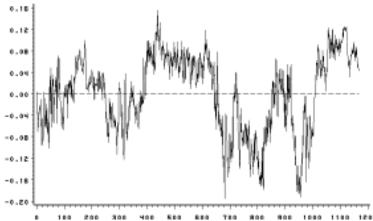
Figure 2: Cointegration regression residuals for 'Lufthansa'
