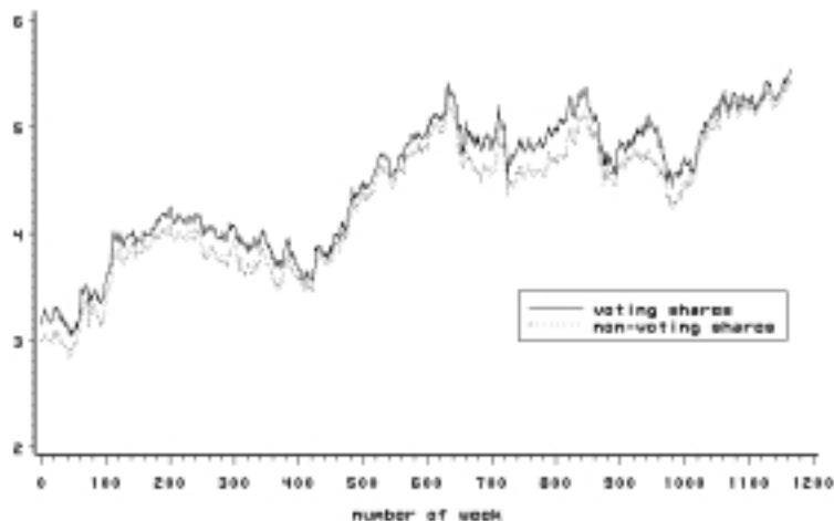
Figure 1: Log-prices of 'Lufthansa' voting and non-voting shares
