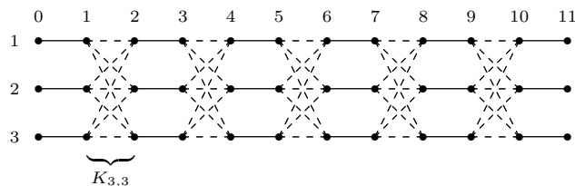
Fig. 8. The graph G_{h,\ell} , h = 3 , \ell = 11 , and its perfect matching.
