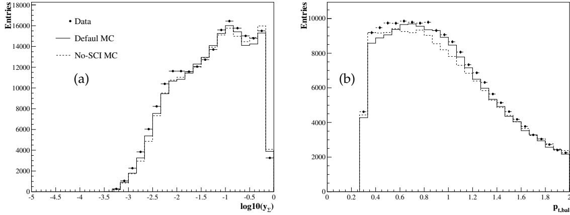
Figure 5.15: (a) y_{\Sigma} and (b) p_{t,bal} distributions for the MC simulation where no diffractive events were generated.
