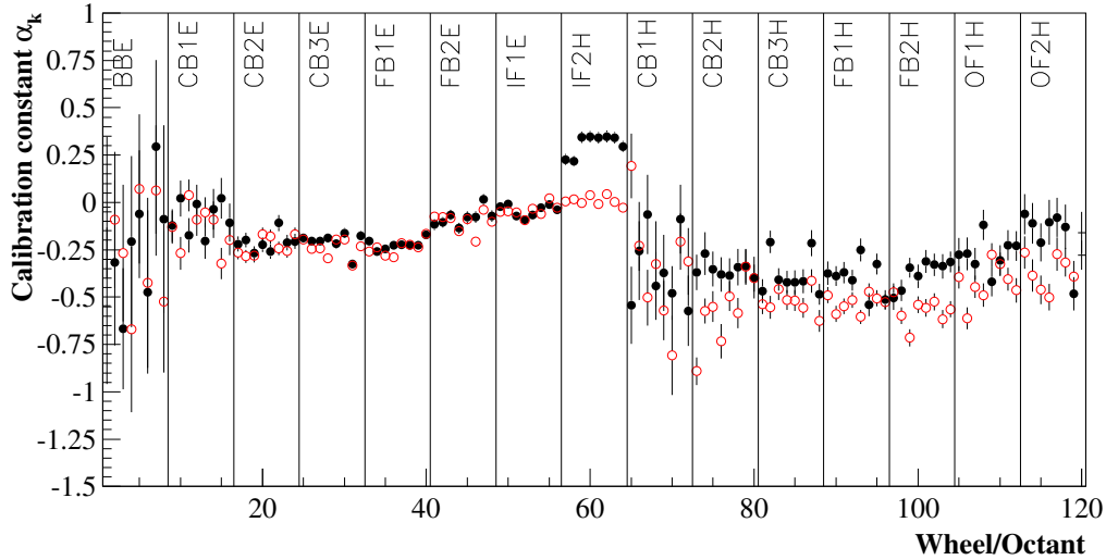
Figure 5.2: Calibration constants for the LAr calorimeter for data of the Shifted vertex period (closed points) and DJANGO MC (open points). Each wheel is labelled according its position with respect the nominal interaction point (central (CB), forward (IF,OF), Backward (B) see also Fig. 2.9). The lines indicate the octants of the corresponding wheels of the LAr calorimeter.
