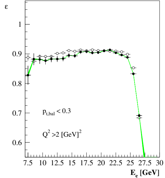
Figure 6.6: Efficiency of the p_{t,bal} < 0.3 cut using only events with Q^2_{\Sigma} > 2 \text{ GeV}^2 . Open points show the efficiency of the signal MC DJANGO, while full points is data where the \gamma p is subtracted using PHOJET.
