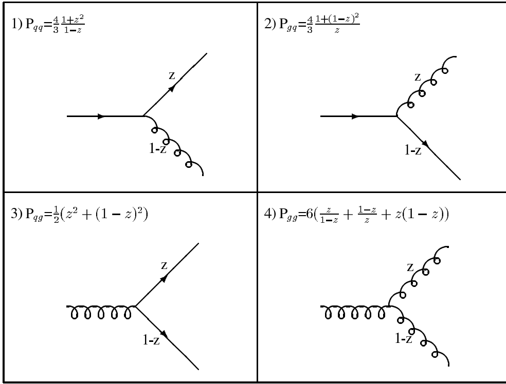
Figure 1.4: Splitting functions
