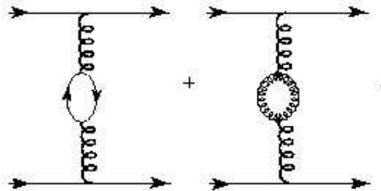
Figure 1.3: Loop diagrams illustrating the interaction between quarks and gluons.
