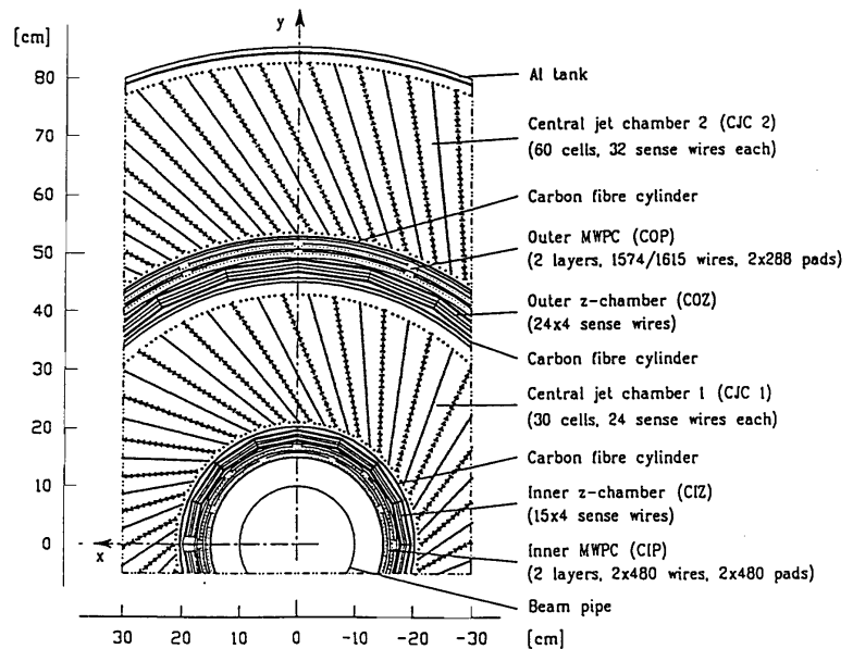
Figure 2.6: Radial view of the tracking detectors [40]
