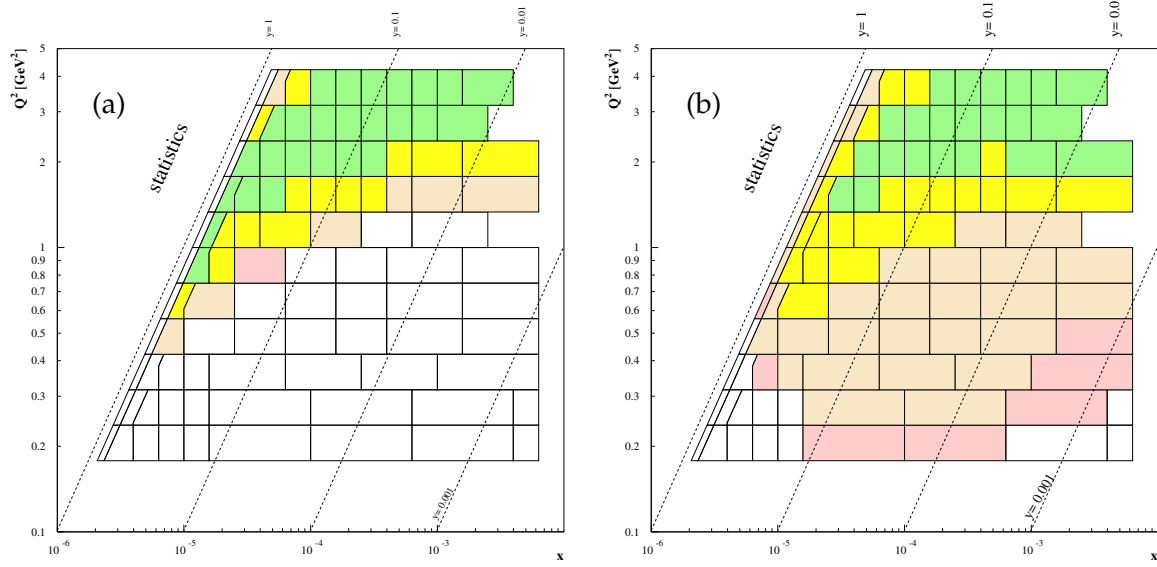
Figure 6.13: Statistics of each Q^2 - x bin during the shifted vertex data (a) reconstructed with the electron method and (b) reconstructed with the \Sigma method
