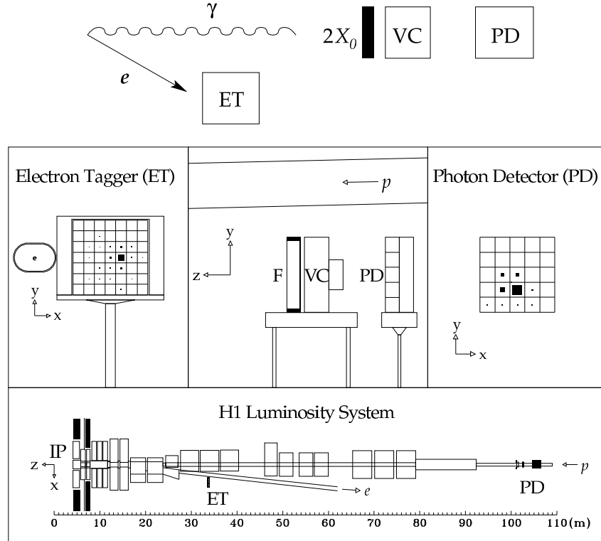
Figure 2.10: Luminosity system [39, 58].
