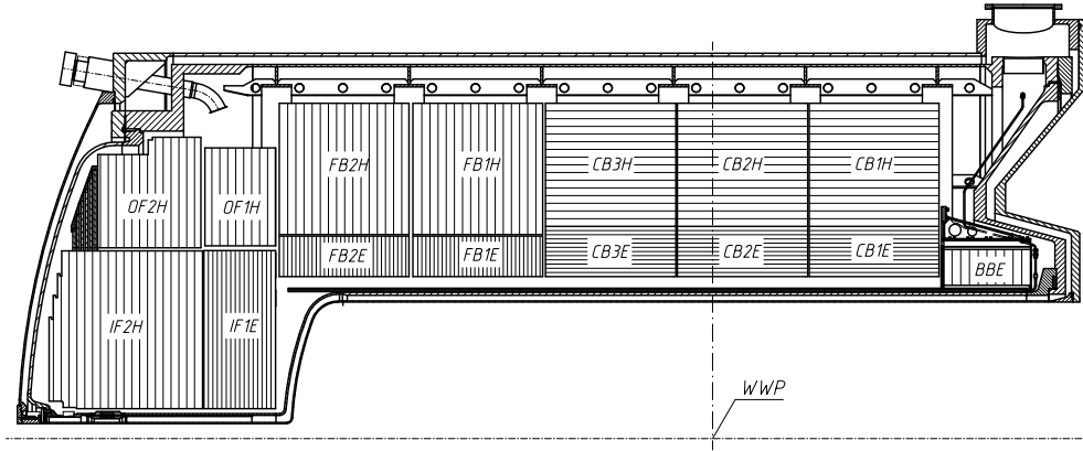
Figure 2.9: r-z view of the LAr calorimeter. The modules are labelled according to its position with respect the interaction point (WWP) either central (CB) backward (B) or forward (IF,OF). The modules corresponding to the electromagnetic and hadronic section are in addition labelled with a E or a H [40, 41].
