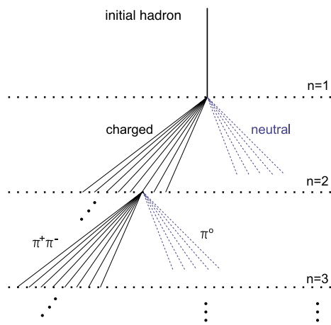
Fig. 5 First three steps of a hadronic cascade in the simplified Heitler-Matthews model (image from Ulrich et al. 2011). Solid (dashed) lines represent charged (neutral) pions. Only one of the splittings is shown after the second step
