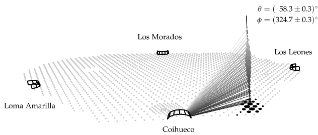
Fig. 6 Hybrid detection of an air shower illustrated with an event recorded by the Pierre Auger Observatory (from Aab et al. 2014a). Dots represent particle detectors on the ground, the four named structures at the edges of the array are fluorescence telescope stations. The shower axis (solid line) with its light intensity profile (grey dots) is indicated, as well the footprint in the ground array (black cylinders). The sizes of the dots and cylinders indicate the logarithm of the local light and particle density, respectively
