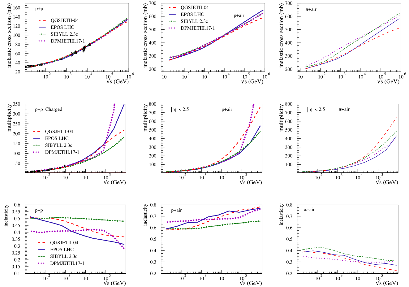
Fig. 16 Basic features of hadronic interactions as a function of \sqrt{s_{NN}} (images from Pierog 2018). From left to right: p - p , p -air, and \pi -air. From top to bottom: total inelastic cross-section, hadron multiplicity at mid-rapidity |\eta| < 2.5 , and inelasticity (complement of the energy
