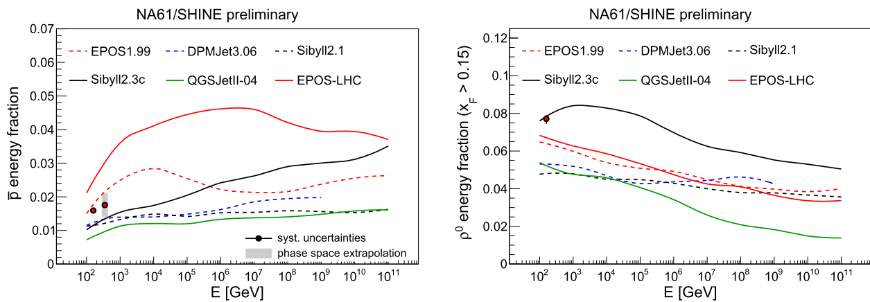
Fig. 19 Energy fraction transferred to anti-protons (left) and \rho^0 -mesons (right) in \pi -C collisions as measured by NA61/SHINE (data points) and as predicted by hadronic interaction models over the whole range of beam energies relevant for air showers (images from Prado 2019; Unger 2020)
