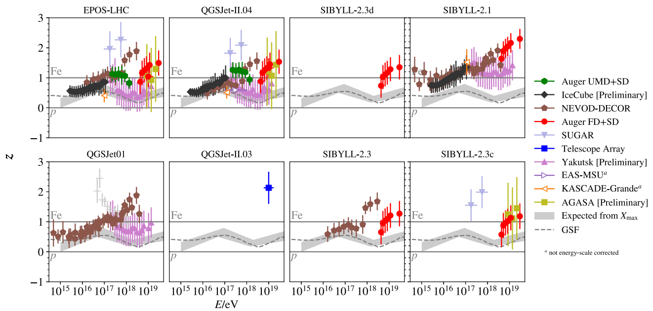
Fig. 3 Compilation of muon measurements converted to the abstract z -scale and after cross-calibrating the energy scales of the experiments as described in the text (image from Soldin 2021). Shown for com-
