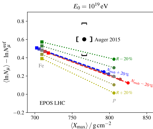
Fig. 11 Impact of modifying the average hadron multiplicity N_{\text{mult}} and the ratio R of electromagnetic to hadronic energy in an air shower on predictions for the depth of shower maximum X_{\max} and the number of muons N_\mu for 10^{10} GeV showers (image from Baur et al. 2019). The representative data point is taken from the Pierre Auger Observatory (Aab et al. 2015a)
