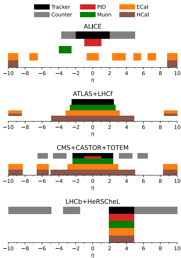
Fig. 17 Acceptances of the LHC experiments ALICE, ATLAS, CMS, LHCb, TOTEM, and LHCf, see Abelev et al. (2014d), Aad et al. (2008, 2009), Bayatian et al. (2006), Surányi et al. (2021), Alves et al. (2008), Aaij et al. (2015a), Khachatryan et al. (2021), Adriani et al. (2008), Anelli et al. (2008) for details. In the legend, a tracker follows individual particles in a magnetic field, while a counter measures particle densities in \eta -intervals. Muon refers to a special muon tracker, PID refers to the ability to identify individual particles, ECal and HCal refer to electromagnetic and hadronic calorimeters, respectively. The inner part |\eta| < 1 of the CMS tracker is partially marked red to indicate its PID capabilities for particles with p_T \lesssim 2 \text{ GeV } c^{-1} . Similarly, the acceptance |\eta| > 8.4 of the LHCf experiment around ATLAS is partially marked brown to indicate its capability to measure neutrons
