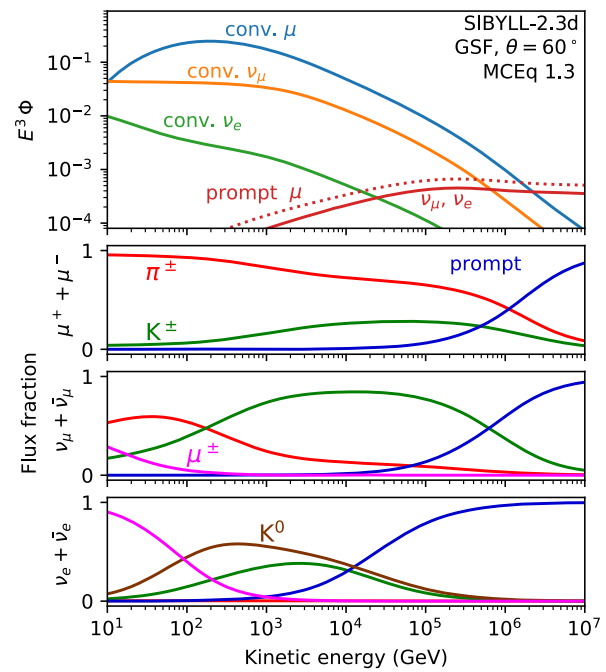
Fig. 9 Top panel: Conventional and prompt lepton fluxes in \text{GeV}^2/(\text{cm}^2 \text{ s sr}) and fractional contributions from parent mesons for \theta = 60^\circ . The calculation uses MCEQ, the SIBYLL2.3d hadronic interaction model and the GSF cosmic-ray flux model as described in the text. Rare decays of unflavoured vector mesons and electromagnetic pairs contribute to the difference between prompt muons (dotted line) and neutrinos (solid line). Lower panels: flux fraction by the type of lepton ancestor. Prompt leptons originate predominantly from decays of charm mesons
