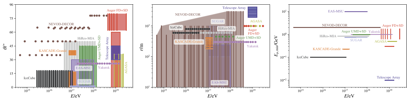
Fig. 7 Air shower experiments have measured the muon density at ground under various conditions, which are shown here (image from Soldin 2021). Points and lines indicate a measurement in a narrow bin of the parameter, while boxes indicate integration over a parameter range. Left: Zenith angle of air showers versus shower energy. Centre:
