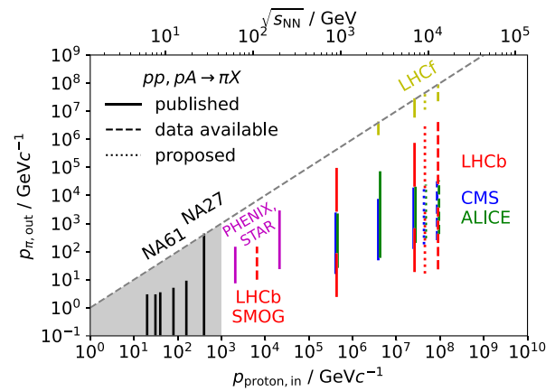
Fig. 18 Overview of data on pion spectra in p - p , p -Pb collisions as a function of the momentum of the incoming proton (Adare et al. 2011; Agakishiev et al. 2012; Chatrchyan et al. 2012b; Abelev et al. 2014e; Abgrall et al. 2014a; Aguilar-Benitez et al. 1991; Adam et al. 2015d; Aaij et al. 2012c; Adriani et al. 2016; Aamodt et al. 2011). The proposed p -O collisions are indicated. In case of LHCb, only hadron yield ratios were measured and not full spectra
