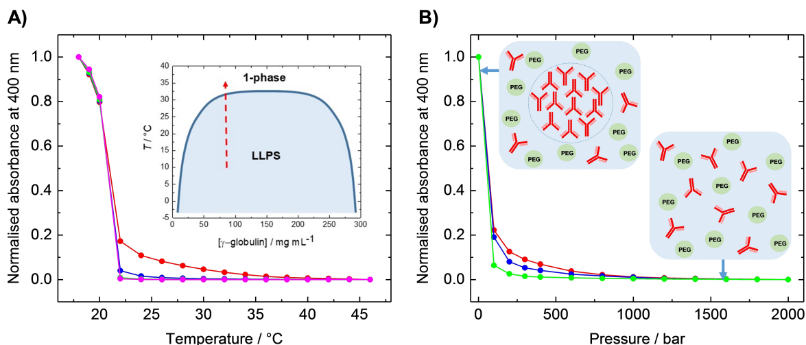
Figure 2. A) UV-Vis absorption at 400 nm of 80\text{ mg mL}^{-1} \gamma -globulin/10% (w/v) PEG 1000 as a function of temperature in buffer (red), 0.2 M TMAO (blue), 0.5 M TMAO (green), and 0.7 M TMAO (magenta). The absorption data were normalized to 1.0 representing their maximum values. Data points are averages of three independent measurements. Below a particular temperature, the “cloud temperature” ( T_{\text{cloud}} ), the sample became visibly cloudy, and the transmitted intensity rapidly dropped, leading to a sharp increase in the absorption. This clouding marks the onset of phase separation and is due to the formation of small droplets of protein-rich phase in the dilute solution or small droplets of protein-poor phase in the concentrated protein solution. Inset: Temperature-concentration phase diagram of \gamma -globulin/10% (w/v) PEG 1000 [7] and direction of the turbidity measurement (red arrow). B) UV-Vis absorption at 400 nm of \gamma -globulin/10% (w/v) PEG 1000 as a function of pressure in buffer (red), 0.2 M TMAO (blue), and 0.5 M TMAO (green) at T = 20^\circ\text{C} . Inset: Schematic pictures representing the PEG-induced liquid–liquid phase separation (LLPS) region of \gamma -globulin (red) and the dissolution of the liquid droplet phase at high pressures.
