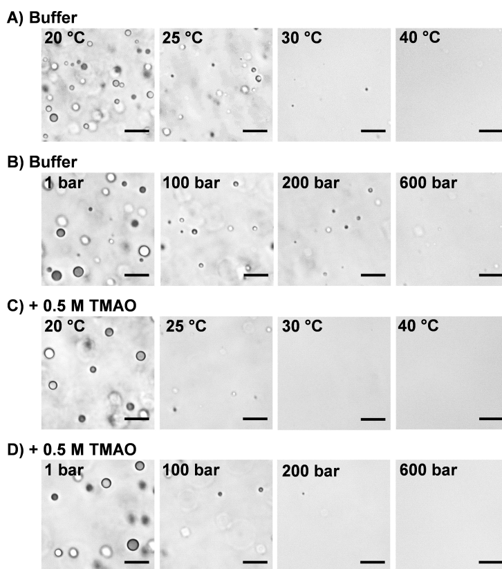
Figure 1. Light microscopy snapshots of 80 mg mL -1 \gamma -globulin in 10% (w/v) PEG 1000 containing buffer solution as a function of A) temperature and B) pressure at T = 20^\circ\text{C} , and in the presence of 0.5 M TMAO as a function of C) temperature and D) pressure dependence at T = 20^\circ\text{C} . Scale bars: 20 \mu\text{m} .
