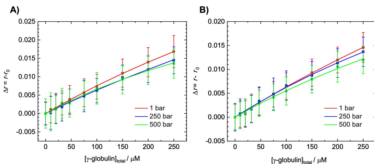
Figure 3. Fluorescence anisotropy data for the self-association of \gamma -globulin at different pressures A) in buffer and B) in the presence of 0.5 M TMAO at T = 20 °C. The experimental data, \Delta r vs. [\gamma\text{-globulin}]_{\text{total}} were fitted accordingly to a 1:1 binding model (represented by lines) in order to evaluate the binding constant, K_b .
