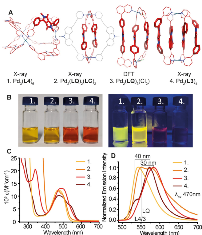
Figure 5. (A) Comparison of the structures of Pd 3 (L 4 ) 6 (X-ray), Pd 2 (LQ) 2 (LC) 2 (X-ray), [Pd 2 (LQ) 3 (Cl) 2 ] (DFT) and Pd 2 (L 3 ) 4 (X-ray) with DPPs highlighted by thicker sticks. (B) Photos of assemblies under ambient (left) and UV light (right). (C) Absorption spectra of the four assemblies in CH 3 CN normalized for a chromophore concentration of 0.35 mM. (D) Normalized emission spectra of the four assemblies in CH 3 CN (λ ex = 470 nm). Emission maxima of ligands L 4 /3 and LQ indicated to visualize the bathochromic shift, especially for Pd 2 (LQ) 3 (CH 3 CN) 2 and Pd 2 (L 3 ) 4 .
