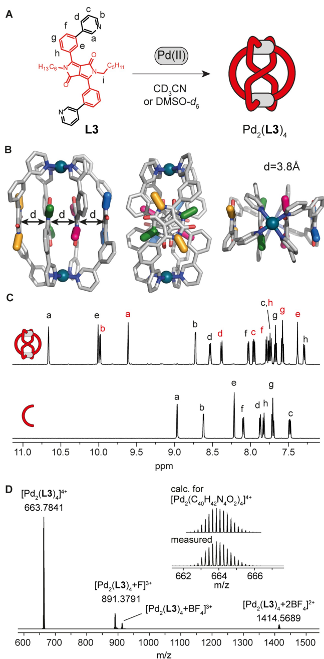
Figure 4. (A) Self-assembly of ligand L3 with 0.5 equiv. of Pd(II) cations to give [\text{Pd}_2(\text{L3})_4](\text{BF}_4)_4 . (B) Different views of the X-ray crystal structure of [\text{Pd}_2(\text{L3})_4](\text{BF}_4)_4 with the distances between the DPP backbones indicated. Alkyl chains and counterions are omitted for clarity. (C) Enlargement of the aromatic region of the ^1\text{H} NMR spectra in \text{CD}_3\text{CN} of L3 and corresponding Pd-based assembly [\text{Pd}_2(\text{L3})_4](\text{BF}_4)_4 . (D) ESI-MS spectrum of [\text{Pd}_2(\text{L3})_4 + n\text{BF}_4]^{(4-n)+} with n=0-2 . The observed and calculated isotopic patterns of [\text{Pd}_2(\text{L3})_4]^{4+} are shown in the inset.
