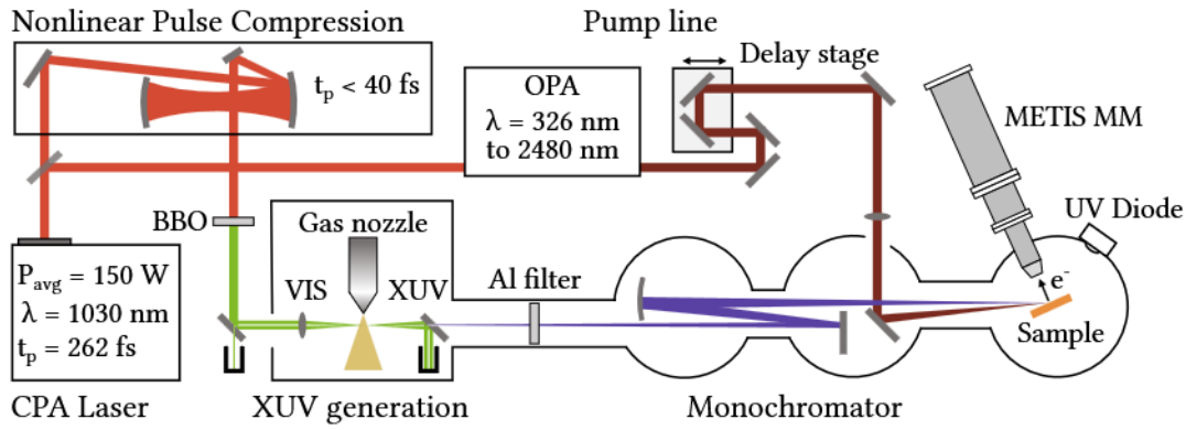
Figure 2.16: Schematic layout of the METIS beamline. The layout shares many similarities with the beamline presented in Chapter 3, but key differences are the higher average-power laser system, gas-filled multi-pass cell (MPC), beam separation of XUV and SHG light, and the TOF detector for the MM.
