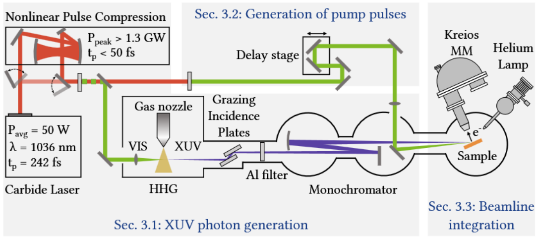
Figure 3.2: Schematic layout of the beamline, which is explained in detail in the following chapters. A commercial laser with optional post-compression is used to generate XUV photons, which emit electrons from a studied sample that are collected by a MM. A second beam path is frequency-doubled and utilized as pump for time-resolved experiments. Published in Ref. [135].
