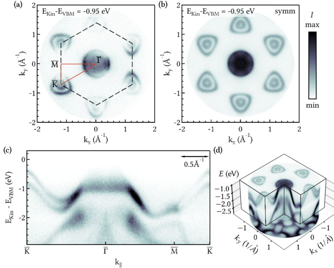
Figure 5.1: Bulk WS 2 band structure characterization. (a) Momentum map with dashed surface BZ and path along high-symmetry points (red solid line), which is used for the band structure cut in (c). (b) Symmetrized momentum map for illustrative purposes, clearly showing triangular warping at the \bar{K} points. (d) Three-dimensional plot that illustrates an acquired data cube. Published in Ref. [135].
