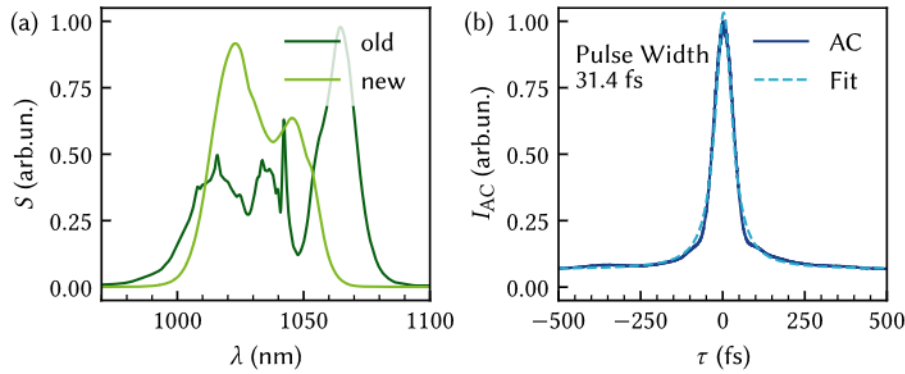
Figure 3.10: Output characterization of the adapted MPC. (a) Spectrum comparison of old and new MPC design. (b) Intensity autocorrelation after dispersion compensation with Lorentzian fit.
