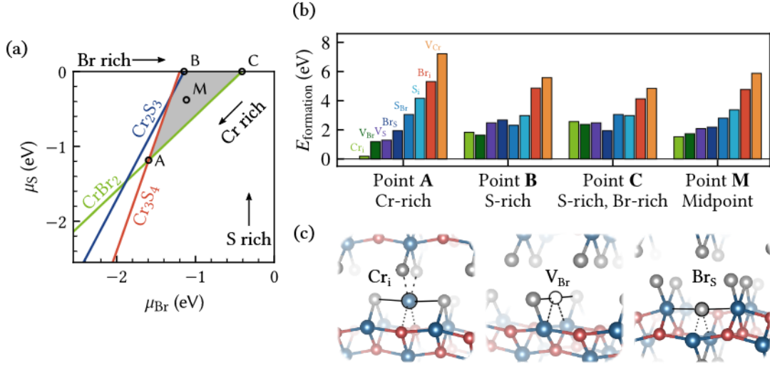
Figure 5.19: DFT-calculated formation of native point defects in CrSBr. (a) Thermodynamic stability region of bulk CrSBr (shaded region) as a function of the individual elements' chemical potentials. (b) Individual point-defect formation energies at different points of the stability region. (c) Atomic structure of the three most favorable point defects. Published in Ref. [274].
