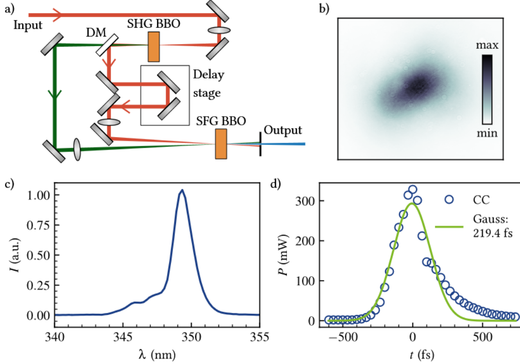
Figure 3.5: A compact setup for third harmonic generation of 1036 nm photons. (a) Schematic layout for the portable setup, where DM stands for dichroic mirror. The generated output is characterized in the following plots: (b) Beam profile, (c) spectrum, and (d) cross correlation signal of IR and SH. The last is fitted with a Gaussian distribution and gives a pulse duration of 219 fs FWHM.
