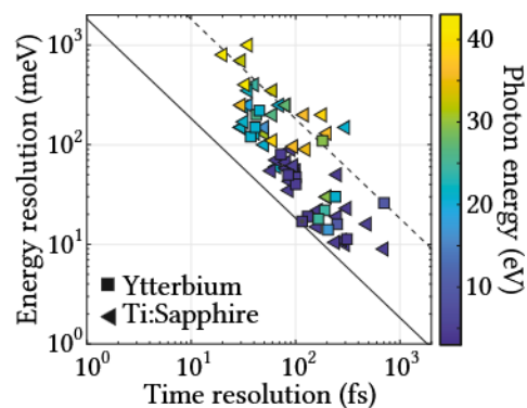
Figure 6.1: Survey of the time-bandwidth product in experimental probe sources. The solid line marks the transform limit, and the dotted line marks ten times the transform limit. Reprinted from Ref. [11], Copyright 2026, with permission from Elsevier.
