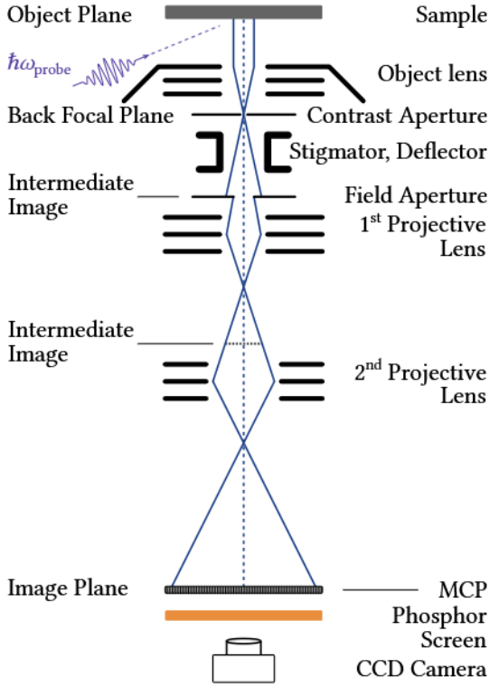
Figure 2.6: Schematic of a prototypical PEEM column. Reprinted from Ref. [84], with permission from Elsevier.
