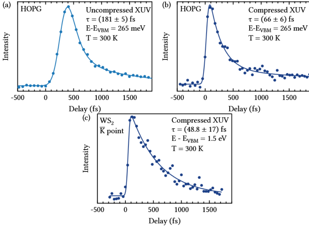
Figure 3.8: Temporal resolution for compressed and uncompressed XUV pulses. (a, b) Transient response of HOPG for both pulses with fits according to Eq. (3.3), yielding enhanced temporal resolution for the compressed pulses, as expected. (c) Transient response of the bulk \text{WS}_2 \bar{\text{K}} -point, with a fit yielding the ultimate temporal resolution in the compressed configuration. Published in Ref. [135].
