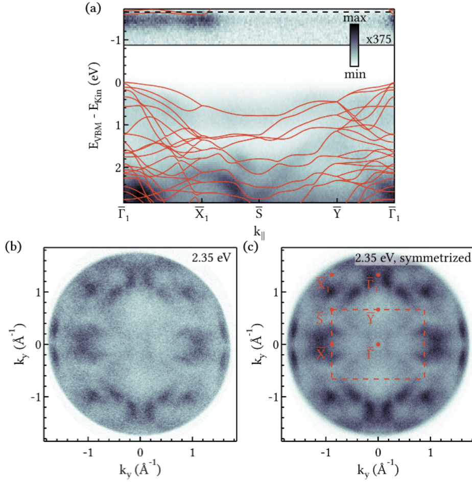
Figure 5.20: Comparison of calculated and experimental band structure of CrSBr. (a) ARPES band structure, symmetrized to negate intensity gradients from the probe incidence direction. Above -0.9 eV, acquisition time is increased x25 and contrast is increased x15. The dotted line indicates E_F . Overlaid is the calculated band structure from DFT within the meta-GGA SCAN functional. The calculation visually agrees with experimental data, including the conduction band dispersion. (b, c) Momentum map at 2.35 eV before and after symmetrization. Published in Ref. [274].
