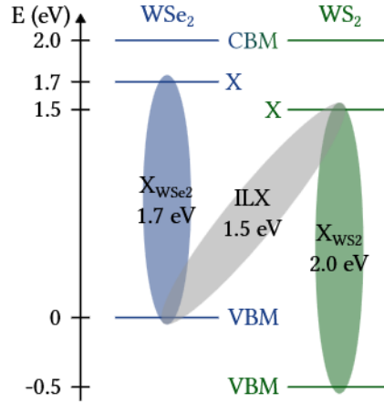
Figure 5.13: Expected energy level alignment of a \text{WS}_2/\text{WSe}_2 heterobilayer. Level positions taken from Refs. [199, 252, 253].
