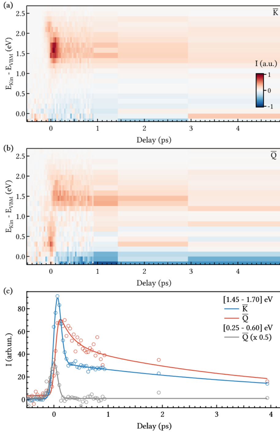
Figure 5.15: Transient ARPES signal. (a) and (b) show the transient response at \bar{K} and \bar{Q} , respectively. Both exhibit a long-lived signal in the range 1.45 eV to 1.70 eV, together with short-lived features near temporal overlap. (c) Integrated intensity at the two high-symmetry points, fitted with Eq. (5.7). The 0.25 eV to 0.60 eV LAPE signal at \bar{Q} is fitted with a Gaussian plus linear background.
