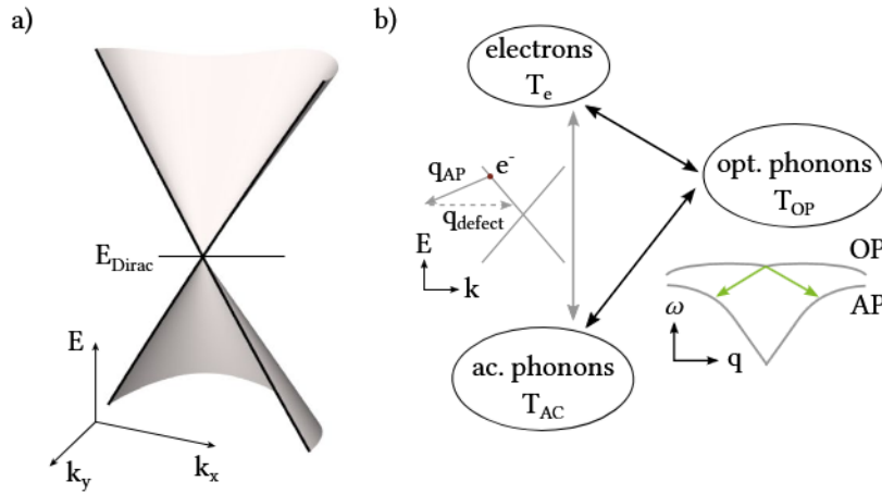
Figure 4.4: (a) HOPG Dirac cone at K/K'. (b) Three-temperature model for hot-electron decay. (a) Adapted from Ref. [120] (Merboldt et al. ), licensed under CC BY 4.0. (b) Adapted with permission from Ref. [14]. © American Physical Society.
