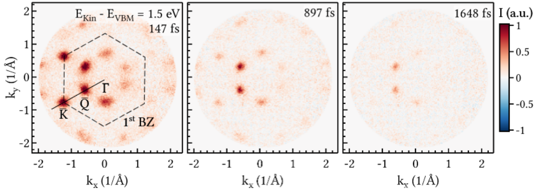
Figure 5.3: Bulk \text{WS}_2 momentum map above the VBM for three delays. The dashed line marks the first surface BZ and the solid line marks the position of the band-structure cut shown in Fig. 5.4a. Published in Ref. [135].
