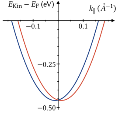
Figure 4.1: Schematic of the surface state in Au(111) with plot parameters taken from Ref. [86].
