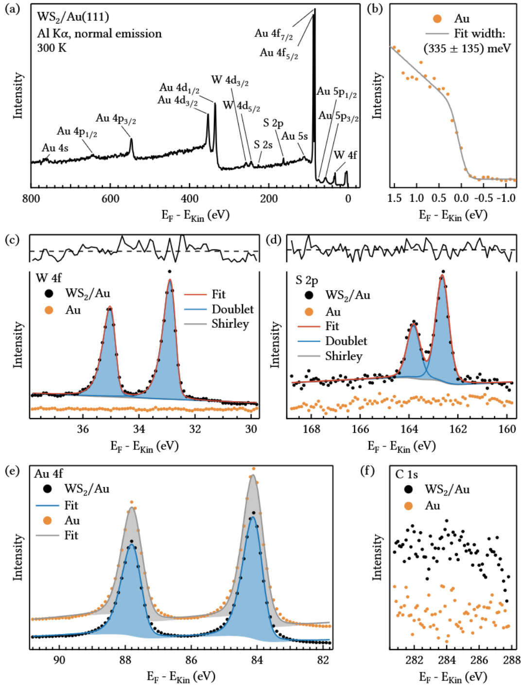
Figure 4.3: XPS characterization of \text{WS}_2 growth on Au(111). Black (orange) markers denote XPS data points after \text{WS}_2 growth (clean Au). (a) Survey spectrum showing only expected contributions from Au, W, and S core levels. (b) Fermi edge of clean Au(111). (c, d) W 4f and S 2p core levels with fitted spin-orbit doublet, respectively. The solid black line indicates the fit residual. (e) Au 4f level before and after growth, fitted with the same doublet line shape. (f) C 1s region, confirming the absence of detectable carbon contamination.
