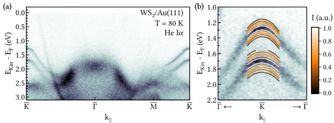
Figure 5.6: (a) Band structure of monolayer WS 2 on Au(111). In contrast to the bulk WS 2 spectra, the VBM now lies at \bar{K} and the sp -band of the substrate is prominent. (b) Zoom-in at the WS 2 \bar{K} point with two fits using Eq. 5.5, which are overlaid as contour lines.
