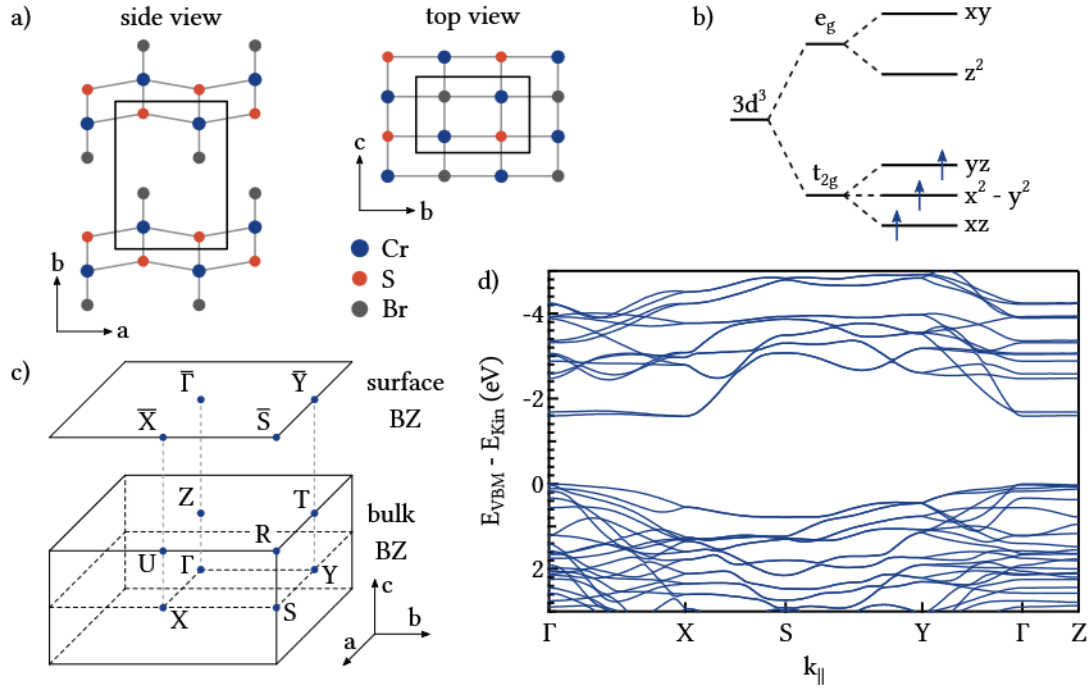
Figure 4.7: Bulk CrSBr crystal and electronic structure. (a) Schematic orthorhombic lattice of a bilayer shown in top and side view. The unit cell is marked by solid black lines. (b) Crystal field splitting of the Cr 3d manifold in CrSBr, yielding a high-spin configuration. The material-specific orbital ordering follows Ref. [77]. (c) Bulk and surface BZ of a simple orthorhombic crystal, with high-symmetry points relevant for this thesis marked in blue. (d) Bulk band structure calculated using density functional theory (DFT) with the meta-GGA SCAN functional, highlighting the anisotropic conduction-band dispersion along \Gamma -X and \Gamma -Y.
