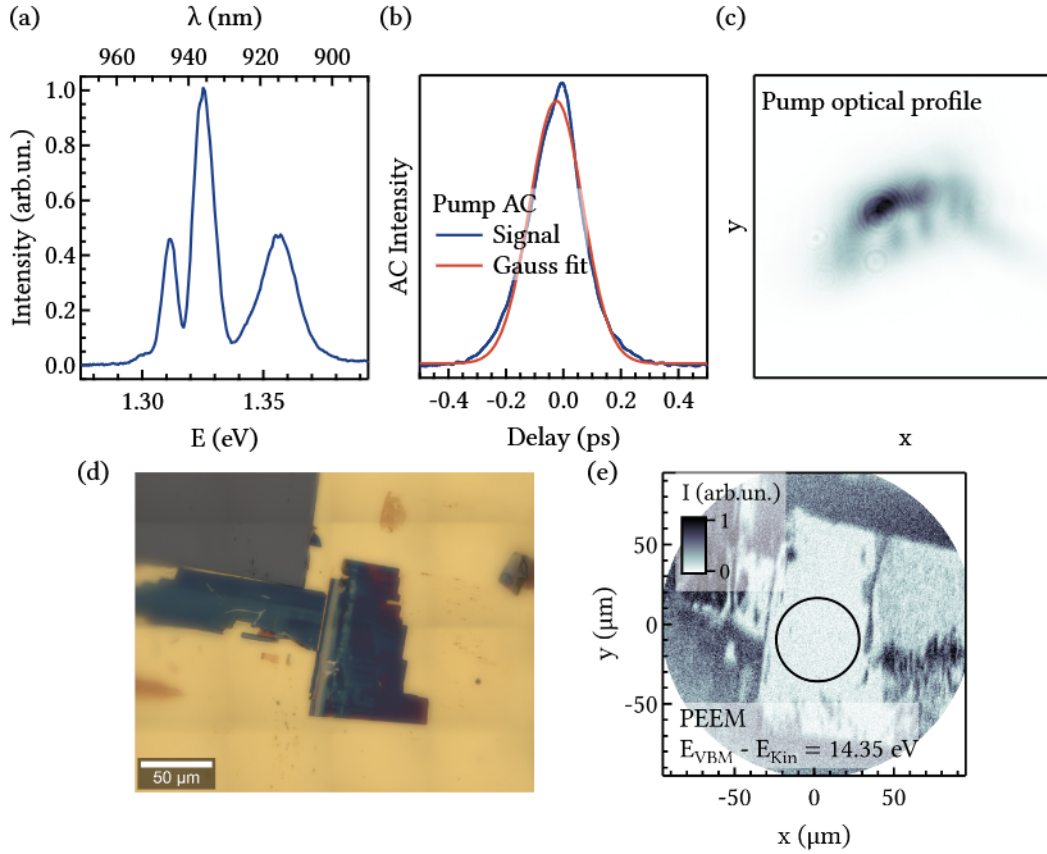
Figure 5.22: Characterization of the optical pump pulse and the exfoliated sample. (a) Spectrum of the pump pulse tuned to the CrSBr exciton resonance at 1.3 eV to 1.4 eV. (b) Pump autocorrelation with Gaussian fitting, yielding a pulse duration of 154 fs. (c) Optical beam profile. (d) Optical image of the exfoliated bulk CrSBr on gold. Different-sized flakes appear as different color shadings. (e) PEEM image of the studied flake area, with a circle marking the field aperture.
