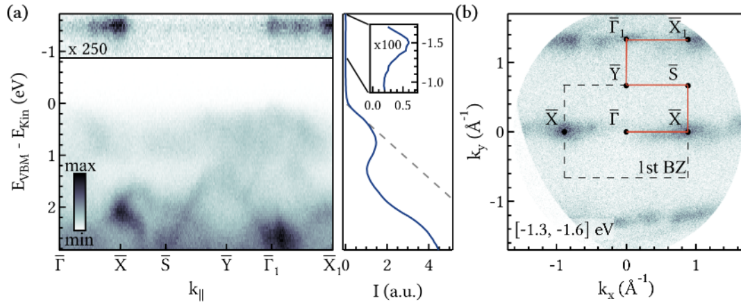
Figure 5.18: Experimental band structure of bulk CrSBr at room temperature. (a) ARPES band structure along high symmetry points of the surface BZ. Data above -0.85 \text{ eV} have x25 acquisition time and x10 contrast increase. The EDC on the right highlights spectral intensity above the VBM, which in turn is determined by linear extrapolation (dotted gray line). (b) Momentum map of the integrated energy range -1.6 \text{ eV} to -1.3 \text{ eV} , exhibiting highly localized intensity patterns along \bar{\Gamma} – \bar{X} . Overlaid are high symmetry points, the 1st BZ boundary (dotted line), and the path of the band-structure cut (solid line). Published in Ref. [274].
