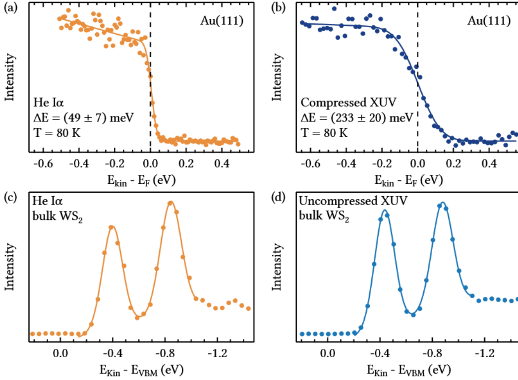
Figure 3.7: Comparison of total energy resolution for He I \alpha , compressed XUV, and uncompressed XUV photons. (a, b) Angle-integrated Fermi edge of Au(111) for He I \alpha and compressed pulses, respectively. Fits according to Eq. (3.2) show significant resolution broadening for the compressed light pulses, as expected. (c, d) Angle-integrated EDC at the bulk WS 2 \bar{K} -point acquired with He I \alpha and uncompressed pulses, respectively. Within the experimental settings, Gaussian fits with linear background yielded the same band widths. Published in Ref [135].
