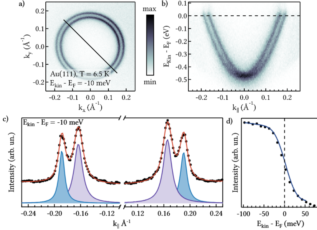
Figure 2.15: KREIOS momentum mode characterization on the Au(111) surface state. (a) Momentum map close to Fermi, showing two rings from Rashba spin-orbit splitting. The solid line marks the cut in (b), showing the surface state's parabolic dispersion, and the line profile in (c). The line profile was fitted with four pseudo-Voigt functions. (d) Angle-integrated Fermi edge, yielding 49 meV Gaussian width from a fit according to Equation (3.2). Published in Ref. [135].
