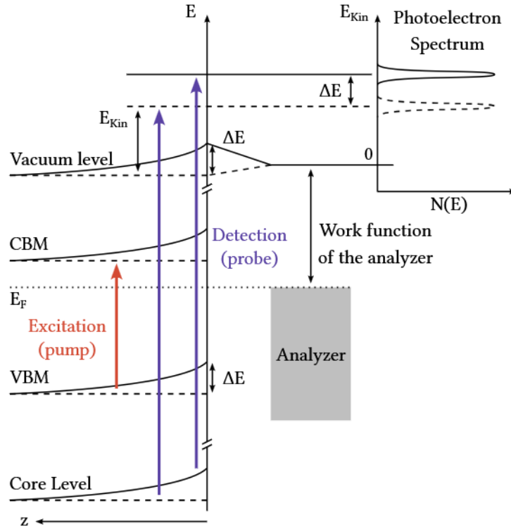
Figure 2.12: Schematic surface photovoltage effect on the energy-band alignment. Dashed lines mark energy levels with flat bands and solid lines mark upward band bending at the surface. Upon optical excitation, photocarriers partially screen the space-charge field and induce dynamic band flattening, which causes an apparent energy shift in the photoemission spectrum because the analyzer defines a fixed energy reference via Fermi-level alignment. Reprinted from Ref. [127], with permission from Elsevier.
