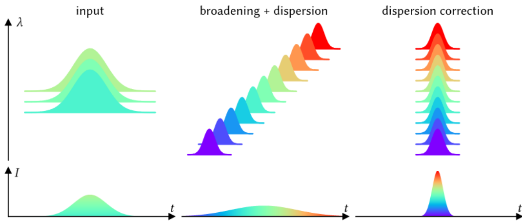
Figure 3.1: Nonlinear compression schematic. The narrowband input pulse is spectrally broadened via SPM and undergoes additional dispersion that stretches the pulse in time (second column). Dispersion correction temporally aligns all frequency components, yielding a broadband output pulse with shorter pulse duration and higher peak intensity (third column).
