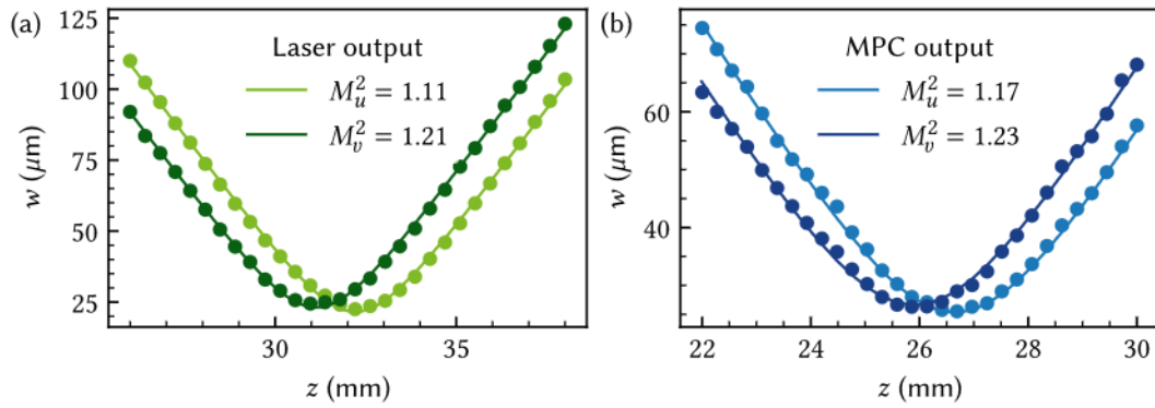
Figure 3.4: M^2 measurement for (a) Carbide laser and (b) MPC output. The acquired beam waist w is fitted according to Eq. 2.5 (solid line) along two perpendicular axes u and v . Published in Ref. [135].
