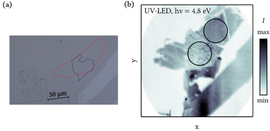
Figure 5.10: Identification of the \text{WS}_2/\text{WSe}_2 flake. (a) Optical microscope image with red and black outlines marking the \text{WS}_2 and \text{WSe}_2 monolayer regions, respectively. (b) Energy-integrated PEEM image of the same region, resolving bubbles and fissures in the transferred layers. The circles indicate the field-aperture positions used for ARPES on the heterobilayer overlap region and on monolayer \text{WS}_2 .
