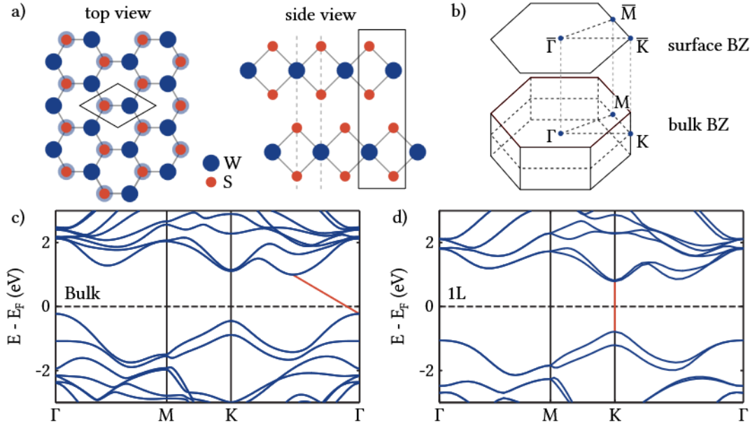
Figure 4.5: WS 2 crystal and electronic structure. (a) Schematic hexagonal lattice of a bilayer with 2H stacking geometry in top and side view. Solid black lines mark the unit cell and gray dotted lines visualize the vertical layer alignment. (b) Bulk and hexagonal Brillouin zone of a hexagonal crystal with high-symmetry points relevant for this thesis marked in blue. (c) and (d) display ab initio band-structure calculations for bulk and monolayer crystals, respectively. Both VBM and CBM positions change in the monolayer limit to the K point, and the band gap, indicated by a red line, increases. (c) and (d) adapted from Ref. [30], with the permission from AIP publishing.
