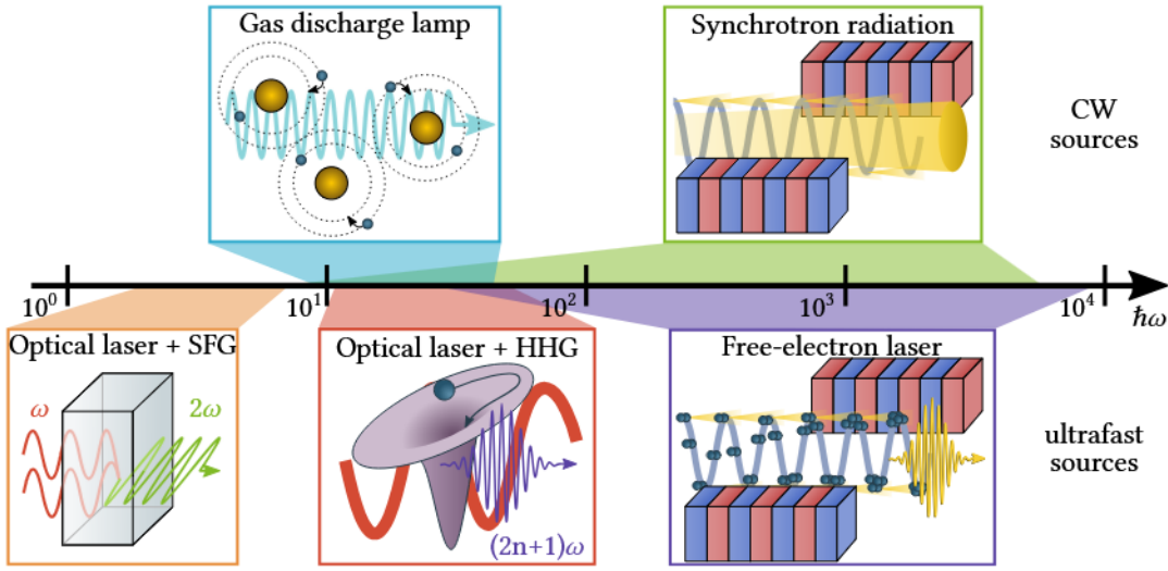
Figure 1.1: Overview of continuous wave (CW) and ultrafast light sources for ARPES. Adapted with permission from Ref. [1], © American Physical Society.
