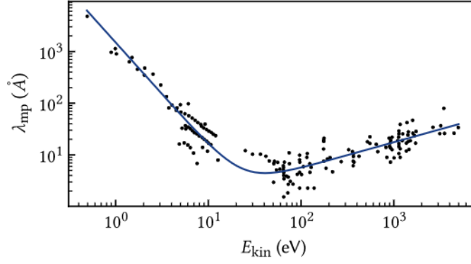
Figure 2.5: Electron inelastic mean free path of elemental solids. The solid line with empirical relation \lambda_{\text{mp}} = AE_{\text{kin}}^{-2} + B\sqrt{E_{\text{kin}}} illustrates the general trend. Fit parameters A and B are not universal and depend on material class and dataset. Adapted from Ref. [69]. © 1979 Heyden & Son Ltd. Reproduced with permission of John Wiley & Sons Limited through PLSclear.
