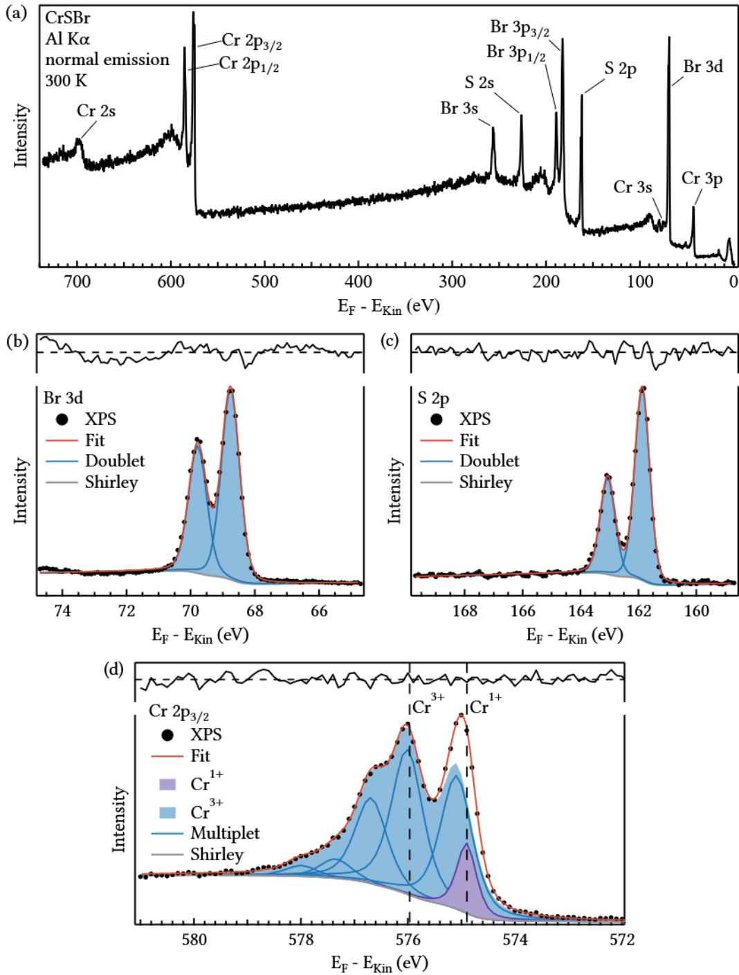
Figure 5.21: XPS characterization of bulk CrSBr. (a) Survey spectrum showing only expected contributions from Cr, S, and Br core levels. (b, c) Br 3d and S 2p core levels with fitted spin–orbit doublet, respectively. The solid black line indicates the fit residual. (d) Cr 2p 3/2 core level, exhibiting multiplet splitting and an additional component for the Cr i . Published in Ref. [274].
