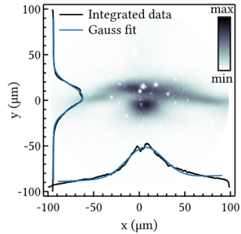
Figure 3.6: PEEM image of XUV probe spot on HOPG. Integrated side profiles are fitted with Gaussian distributions yielding 19.5 \mu\text{m} \times 31.7 \mu\text{m} . Published in Ref. [135].
