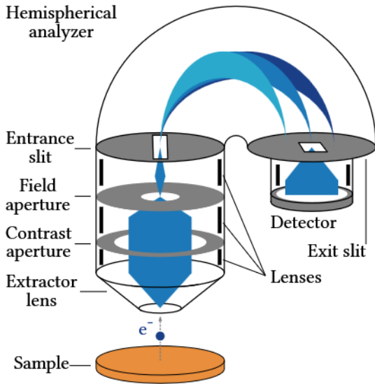
Figure 2.14: Schematic illustration of the KREIOS 150 MM. Published in Ref. [135].
