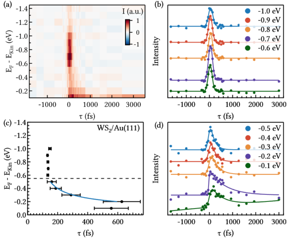
Figure 5.8: Hot electron relaxation in \text{WS}_2/\text{Au}(111) . (a) Angle-integrated delay map. The single traces above -0.6 eV are plotted in (b) with single Gaussian fits and the traces below -0.6 eV are plotted in (d) with fits according to (3.5). (c) Gaussian widths for the high energy window and exponential decay rates for the low energy window. The latter is fitted with a Fermi-liquid fit function.
