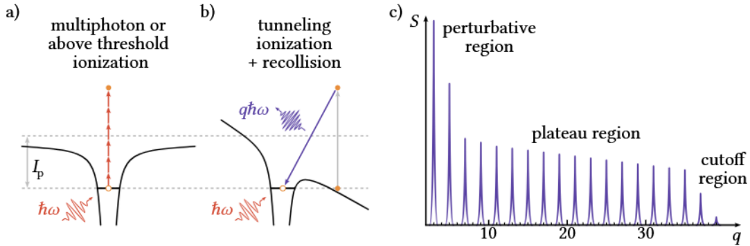
Figure 2.3: Schematic representation of electron ionization mechanisms and high harmonic generation. (a) Multiphoton ionization. (b) Tunneling ionization with recollision model, resulting in harmonic emission. (c) Schematic high-harmonic spectrum S as a function of harmonic order q at energy q\hbar\omega .
