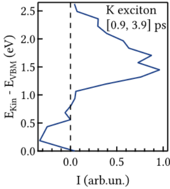
Figure 5.17: Angle-integrated ARPES signal of the K exciton for 0.9 ps to 3.9 ps.
