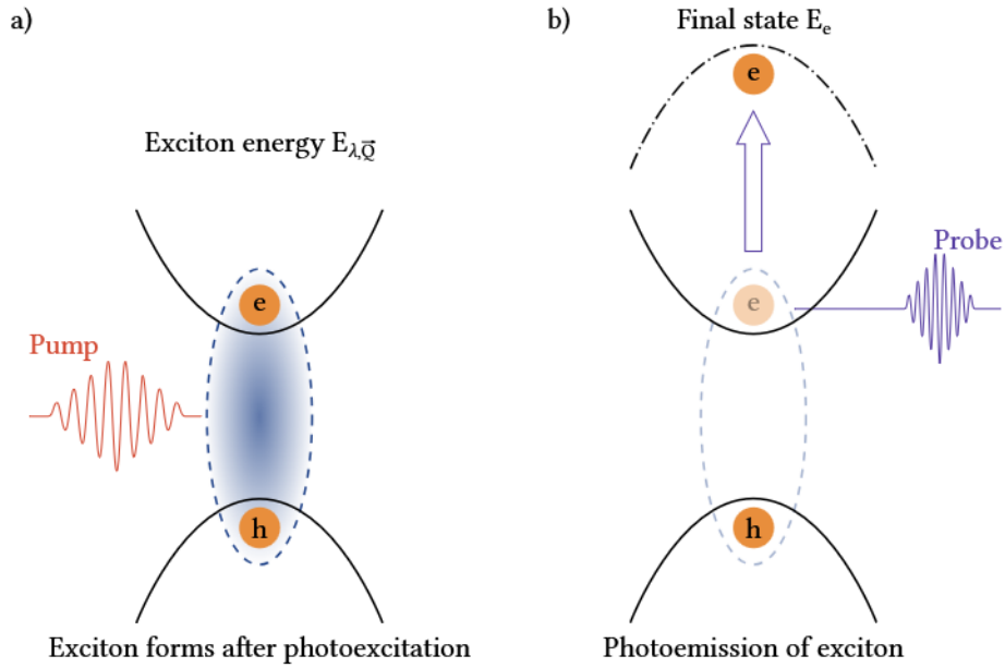
Figure 2.10: Exciton fingerprint in photoemission, adapted from Ref. [112] (Man et al. ), licensed under CC BY-NC 4.0. (a) Exciton formation upon optical excitation. (b) Valence-band-like dispersion signature of the photoemitted electron.
