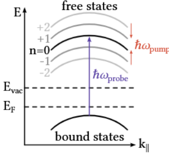
Figure 2.11: Schematic illustration of LAPE sidebands: absorption and stimulated emission of pump photons lead to replicas of the photoemission feature spaced by \hbar\omega_{\text{pump}} .
