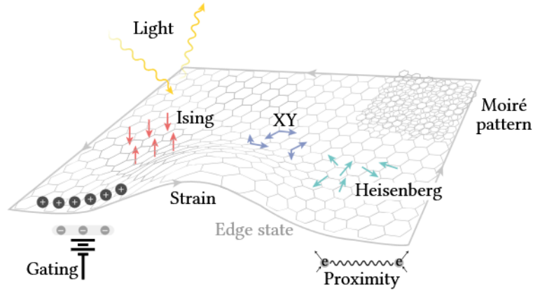
Figure 1.2: Schematic overview of control knobs and emergent phenomena in two-dimensional vdW materials and heterostructures. Electrostatic gating, strain, moiré superlattices (twist), optical excitation, and interlayer proximity coupling provide routes to tune electronic and magnetic behavior. The Ising/XY/Heisenberg labels indicate different magnetic anisotropy regimes. Reproduced from Ref. [25], with permission from Springer Nature.
