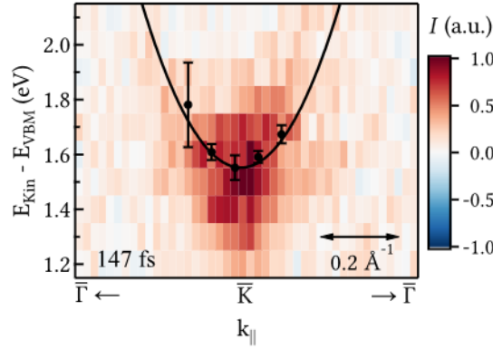
Figure 5.5: Dispersion of the transiently occupied conduction band at \bar{K} . Markers show the momentum-dependent band position retrieved from Gaussian fitting, but the SNR does not allow unambiguous extraction of the effective mass. The solid line uses 0.36 m_e from Ref. [236].
