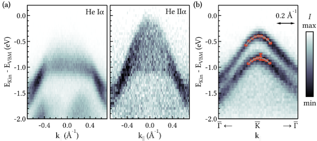
Figure 5.2: (a) Influence of the PME on the photoemission intensity close to the VBM at the \bar{\Gamma} point. (b) Dispersion of the \bar{K} point. Markers denote the momentum-dependent band position extracted from Gaussian fitting. Consecutive fitting with a parabolic function yields the effective masses for the spin-split valence band. Partly published in Ref. [135].
