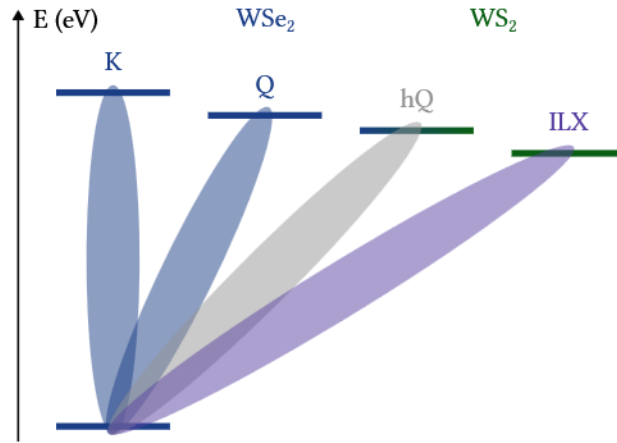
Figure 5.16: Possible exciton species in heterobilayer \text{WS}_2/\text{WSe}_2 after excitation of the K exciton in \text{WSe}_2 . In \text{WSe}_2 , the heterobilayer lowers the Q valley relative to K, thus shifting the CBM to \bar{Q} . In addition, energetically favorable hybrid excitons with hybridized electron or hole wave function could form with a plethora of conduction- and valence-band valley combinations (here, electron hybridization at Q is shown). Finally, electron transfer allows formation of ILX.
