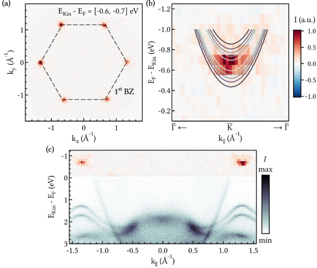
Figure 5.7: Transient \text{WS}_2/\text{Au}(111) signal at temporal overlap. (a) Integrated momentum map from -0.6 \text{ eV} to -0.7 \text{ eV} , only exhibiting intensity at the \bar{K} points. A dashed line marks the first surface BZ. (b) Dispersion of the signal at \bar{K} , which is fitted according to Eq. (5.5). (c) Band structure cut along \bar{K}-\bar{\Gamma}-\bar{K} , with the static band structure as reference.
