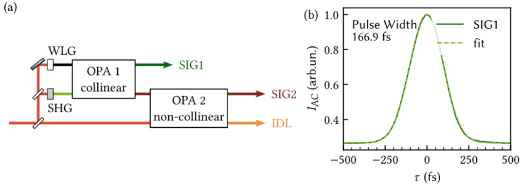
Figure 3.9: ORPHEUS-ONE-HP OPA. (a) Schematic OPA layout comprising two amplification stages. (b) Intensity autocorrelation of SIG1 output with Gaussian fit.
