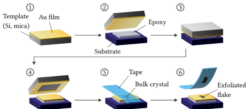
Figure 4.2: Schematic Au-assisted exfoliation on template-stripped gold. (1) Gold is evaporated on a smooth substrate. (2) The gold film is glued onto a sample plate to form (3) a sandwich structure that protects the Au surface from exposure to air. (4) Immediately before use, the substrate is peeled off to expose a fresh Au surface, onto which (5) a bulk vdW crystal is pressed. (6) In vacuum, the crystal is exfoliated, leaving a thin flake with a fresh surface suitable for low-temperature ARPES. Reproduced from Ref. [176] under the license CC BY-NC-ND 4.0, font style modified.
