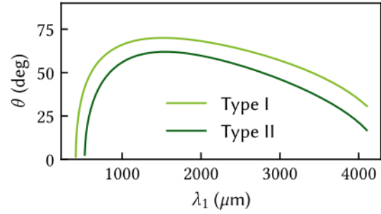
Figure 2.1: Phase-matching angle \theta between k_1 and the crystal optical axis for SHG in a BBO crystal. Computed with refractive indices specified in Ref. [57].
