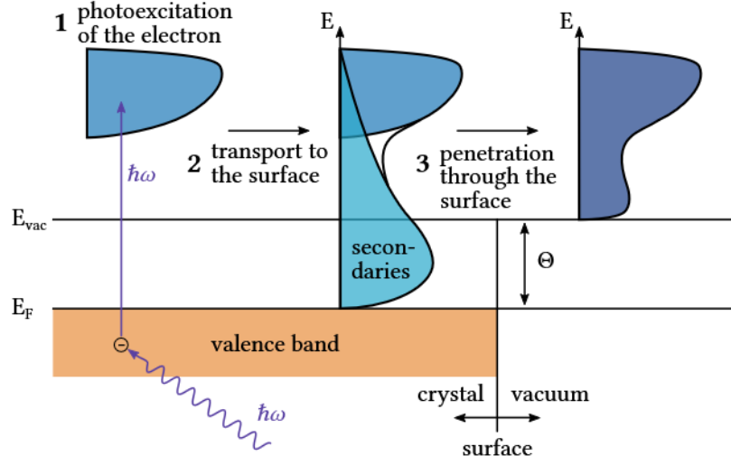
Figure 2.4: Schematic of the three-step model describing the photoemission process. The electron is excited above the vacuum energy in step 1, propagates to the surface in step 2, and leaves the surface barrier in step 3. Reproduced from Ref. [65], with permission from Springer Nature.
