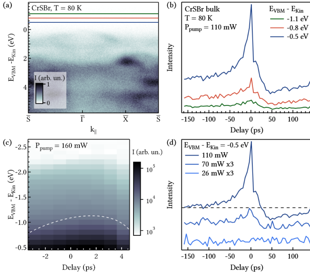
Figure 5.23: Transient ARPES signal on bulk CrSBr. (a) Static band structure with colored lines highlighting the energy positions of the traces in (b), which display a strong asymmetric signal over tens of ps. (c) Binding energy versus delay map around temporal overlap. The white dotted line is drawn by hand and serves as guide to the eye. (d) Transient intensity as a function of pump fluence, with the dotted line drawn by hand.
