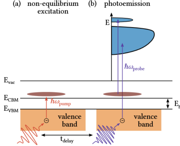
Figure 2.7: Schematic illustration of conduction-band excitation in a semiconductor, observed in trARPES. (a) Above-bandgap excitation with pump pulse \hbar\omega_{\text{pump}} produces a hot-electron distribution in the conduction band. (b) The probe pulse follows the pump after time t_{\text{delay}} and induces photoemission with photon energy \hbar\omega_{\text{probe}} from both the valence band and the transient conduction-band population.
