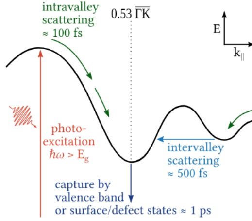
Figure 2.8: Hot-electron relaxation in bulk MoS 2 after above-bandgap excitation, captured with trARPES. Adapted with permission from Ref. [93]. © American Physical Society.
