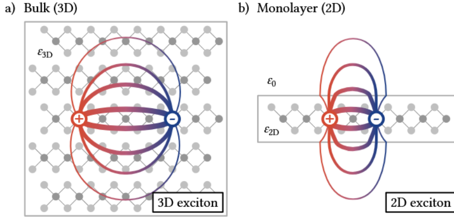
Figure 4.6: Effect of dielectric screening. The schematic electric field lines generated by the Coulomb interaction of the exciton's electron and hole are displayed in real space for a (a) bulk and (b) monolayer TMD. Reduced screening in the monolayer increases both the band gap and the exciton binding energy. Adapted with permission from Ref. [29]. © American Physical Society.
