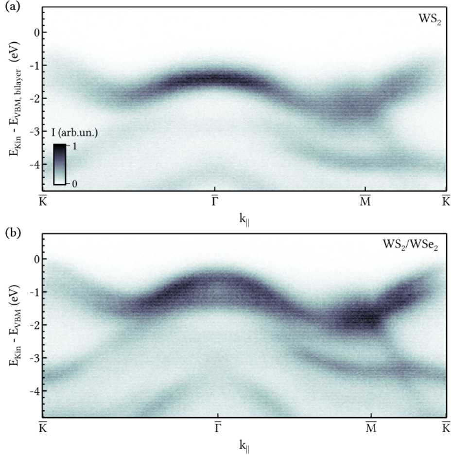
Figure 5.11: ARPES spectra of (a) the \text{WS}_2 monolayer region and (b) the \text{WS}_2/\text{WSe}_2 heterobilayer overlap region.
