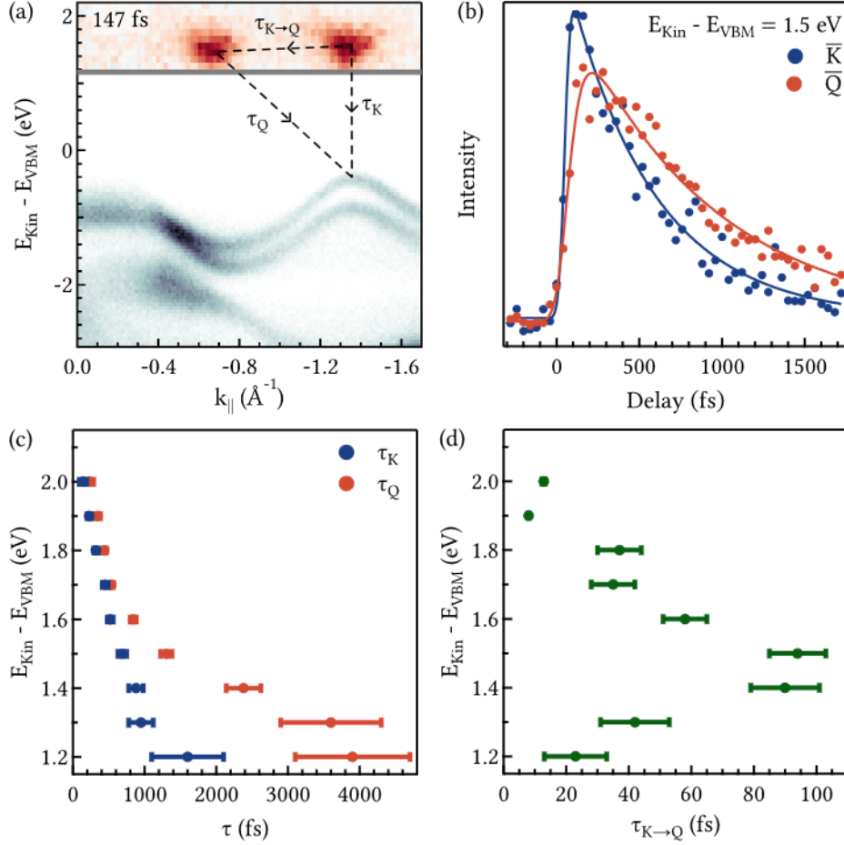
Figure 5.4: Hot electron relaxation in bulk WS 2 . (a) Band structure along \bar{\Gamma} - \bar{K} with the static spectrum at the bottom and the transient spectrum at 147 fs at the top. The dashed lines illustrate the relaxation pathways of the rate-equation model. (b) Exemplary transient intensities at \bar{Q} and \bar{K} for 1.5 eV with the model fit plotted as a solid line. (c, d) Energy-dependent scattering rates for \bar{K} , \bar{Q} , and intervalley scattering. Published in Ref. [135].
