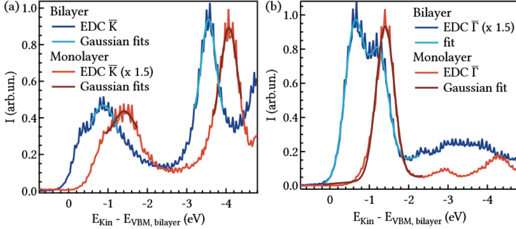
Figure 5.12: EDC comparison of monolayer \text{WS}_2 and the \text{WS}_2/\text{WSe}_2 heterobilayer at (a) \bar{K} and (b) \bar{\Gamma} . Peak fits in (a) yield an estimated valence-band offset of order 0.5 eV, consistent with a type-II band alignment. At \bar{\Gamma} in (b), the higher-binding-energy feature in the heterobilayer is shifted by approximately 160 meV with respect to the corresponding monolayer \text{WS}_2 feature. Such a fingerprint is consistent with screening-induced energy renormalization but is not, by itself, a unique signature of strong hybridization [250].
