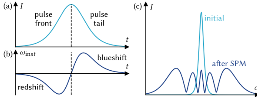
Figure 2.2: Calculated self-phase modulation (SPM) for n_2 > 0 . (a) Intensity profile of a \text{sech}^2 pulse. (b) Self-phase modulation (SPM)-induced instantaneous frequency shift. (c) Resulting spectral broadening (schematic).
