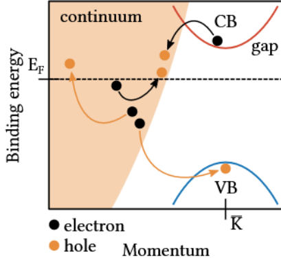
Figure 5.9: Schematic Auger-like scattering channel for TMDs on metallic substrates. Reprinted with permission from Ref. [242]. © 2015 American Chemical Society.
