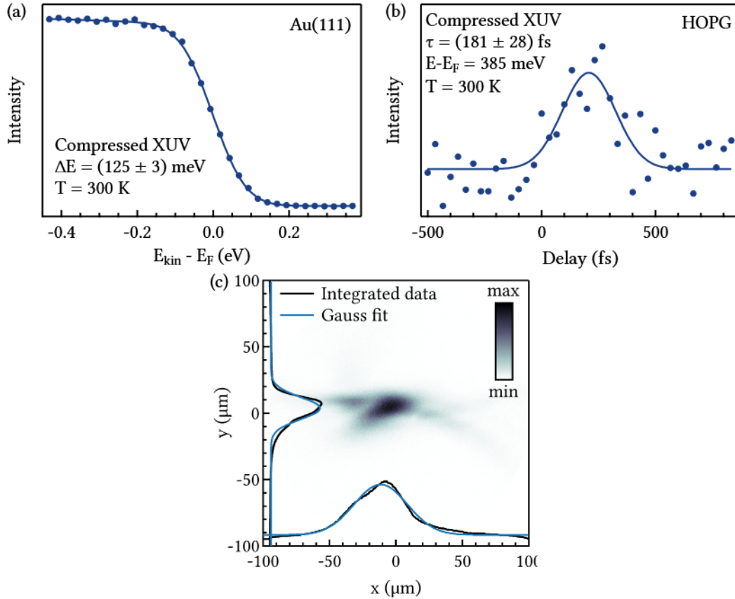
Figure 3.11: Beamline performance after OPA integration. (a) Fermi edge of Au(111) fitted with Eq. (3.2). (b) Transient response on HOPG with SIG1 as pump, fitted with a Gaussian function. (c) XUV spot size in PEEM with Gaussian fits for integrated distributions.
