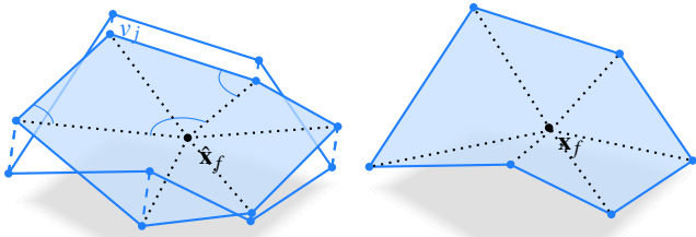
Figure 2: Left: Non-planar polygon and its orthogonal projection with maximum area. The projection's virtual vertex position \hat{\mathbf{x}}_f is the trace minimizer of the planar cotangent stiffness matrix. Right: The virtual vertex position \mathbf{x}_f is obtained by multiplying the original vertices with the discrete harmonic weights of the projection.
