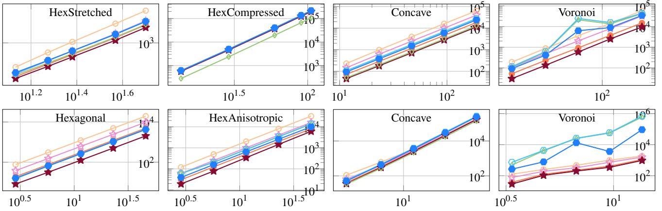
Figure 9: The condition number \kappa(\mathbf{S}^O) of the respective polygon stiffness matrices on planar (top) and spherical (bottom) polygon meshes. x-axis: inverse mean edge length, y-axis: Condition Number.
