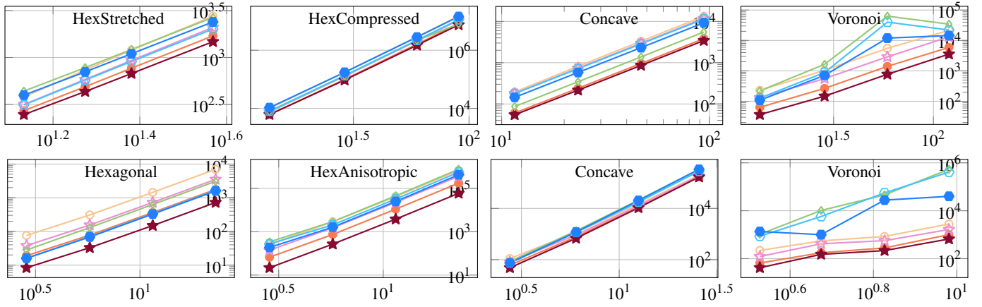
Figure 10: The condition number \kappa(\mathbf{L}^O) of the respective point-wise polygon Laplacians on planar (top) and spherical (bottom) polygon meshes. x-axis: inverse mean edge length, y-axis: Condition Number.
