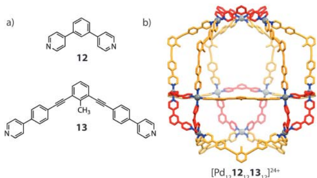
Fig. 8 (a) The short ( 12 ) and long ( 13 ) angular ligands (b) a heteroleptic [\text{Pd}_{12}\text{L}_{12}\text{L}_{13}]^{24+} cantellated tetrahedron.
