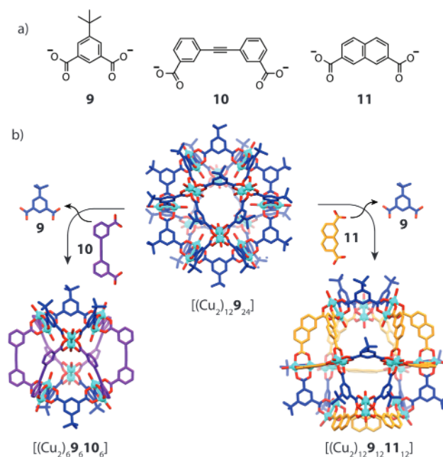
Fig. 7 (a) Bent dicarboxylate ligands 9–11 bearing angles of 120°, 60° and 120° respectively; (b) transformation of the homoleptic [(\text{Cu}_2)_{12}\mathbf{9}_{24}] cage to heteroleptic species [(\text{Cu}_2)_6\mathbf{9}_6\mathbf{10}_6] (left) and [(\text{Cu}_2)_{12}\mathbf{9}_{12}\mathbf{11}_{12}] (right) by ligand substitution.
