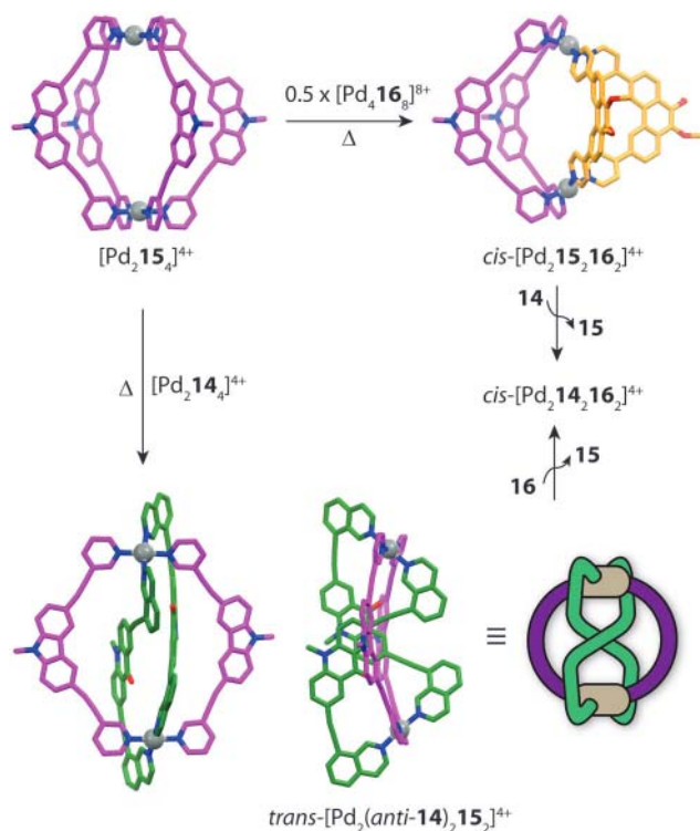
Fig. 11 Cage-to-cage integrative transformations of [\text{Pd}_2\text{15}_4]^{4+} to form either cis or trans heteroleptic cages. Each heteroleptic cage can be transformed to \text{cis-}[\text{Pd}_2\text{14}_2\text{16}_2]^{4+} by addition a competing ligand ( 14 or 16 ).
