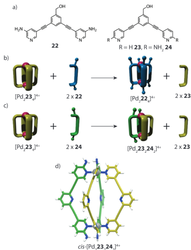
Fig. 14 (a) Banana-shaped pyridyl ligands containing amino substituents in meta- or ortho-positions; (b) ligand substitution reaction resulting in complete ligand displacement; (c) partial ligand displacement to give a heteroleptic cis -cage; (d) a DFT-model of cis - [\text{Pd}_2\mathbf{23}_2\mathbf{24}_2]^{4+} . Reproduced with permission from ref. 71.
