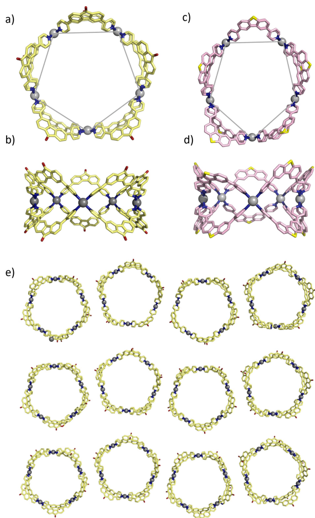
Figure 2. X-ray crystal structures of perfectly pentagonal \text{Pd}_5\text{L}^{10} in (a) top and (b) side view, and of distorted \text{Pd}_5\text{L}^{10} in (c) top and (d) side view; (e) solid-state packing of \text{Pd}_5\text{L}^{10} (counter anions and solvent molecules omitted for clarity).
