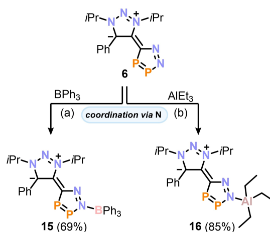
Scheme 4. Coordination of diphosphole 6 affording compounds 15 and 16 ; reagents and conditions: a) +1.0 eq. \text{BPh}_3 ; THF, -35^\circ\text{C} to r.t., 1 h; b) +1.0 eq. \text{AlEt}_3 ; toluene, -35^\circ\text{C} to r.t., 2 h.
