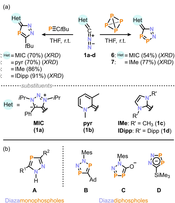
Scheme 2. (a) (3+2) Cycloaddition reactions of diazoalkenes with t BuCP and P 4 affording 2–5 and 6–7 , respectively. (b) Selection of literature known 1,2,4-diazamonophospholes ( A ) and 1,2,3,4-diazadiphospholes ( B–D ); R' ≠ R 2 = organic residue; MIC: mesoionic carbene. Mes: 1,3,5-trimethylphenyl.
