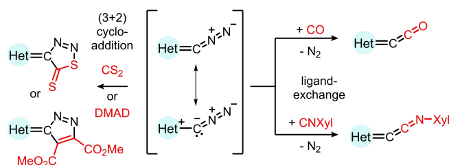
(b) Small molecule activation with stable diazoalkenes
