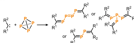
(b) Small molecule activation with stable diazoalkenes
