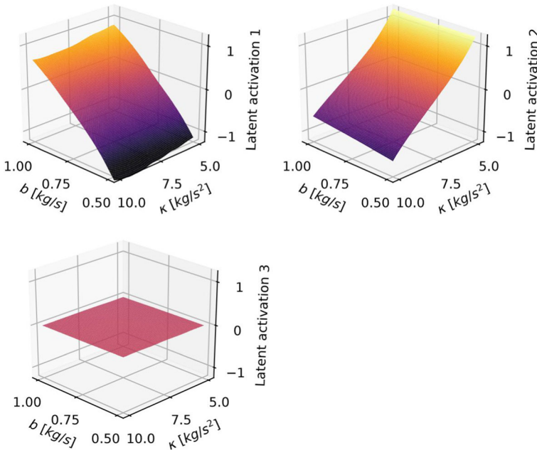
Fig. 4 Activations of SciNet's three latent units when trained to predict the behavior of a pendulum, plotted against the two constants ( b and k ) describing the damped pendulum equation (both divided by mass). Taken from Iten et al. (2020b), courtesy of the authors. Color available online
