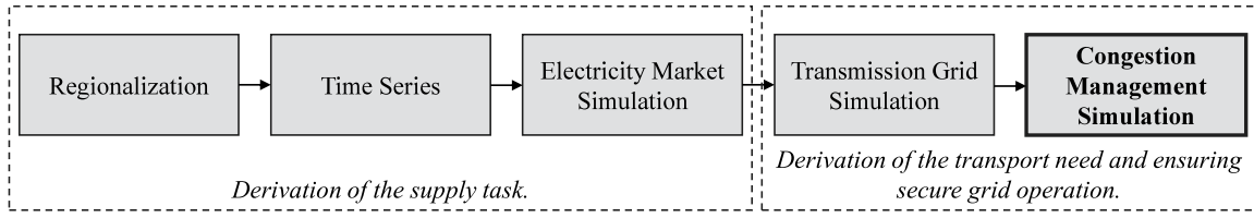
Fig. 1. Structure of the MILES framework.
