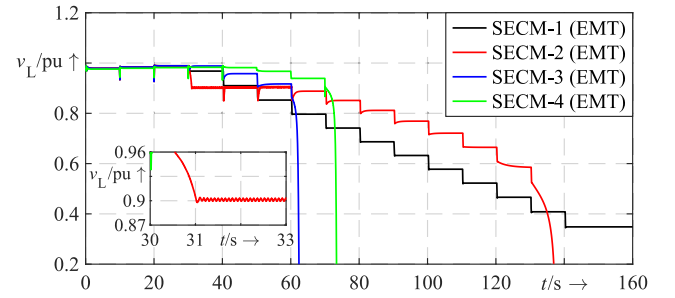
Fig. 11. Comparison of long-term voltages dynamics of the load voltage v_L for a droop converter with four different SECM and p_{L,1} = 1.0 .
