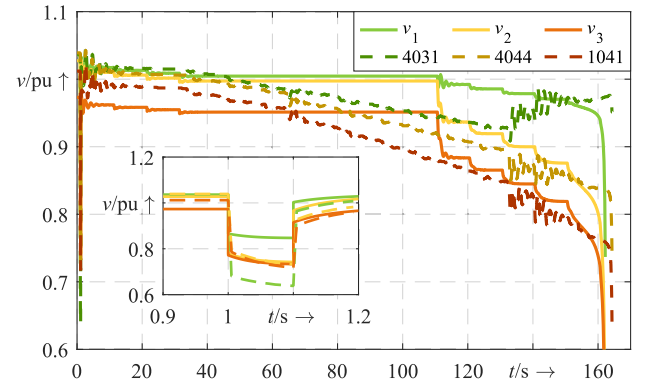
Fig. 5. Comparison of voltage dynamics between Nordic test system and ANS in a phasor simulation (for synchronous generators).
