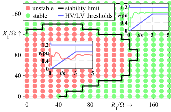
Fig. 6. Exemplary determination of a short-term voltage stability limit by short-circuit impedance sampling ( |\Delta X_f| = |\Delta R_f| = 10 \Omega ) and assessing high and low-voltage stability thresholds.
