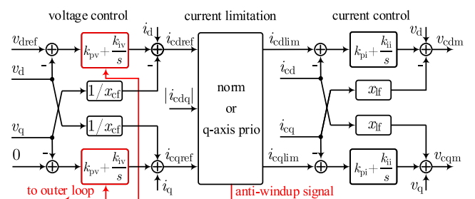
Fig. 2. Cascaded voltage and current control with current limitation and anti-windup method (own illustration, based on [13]).
