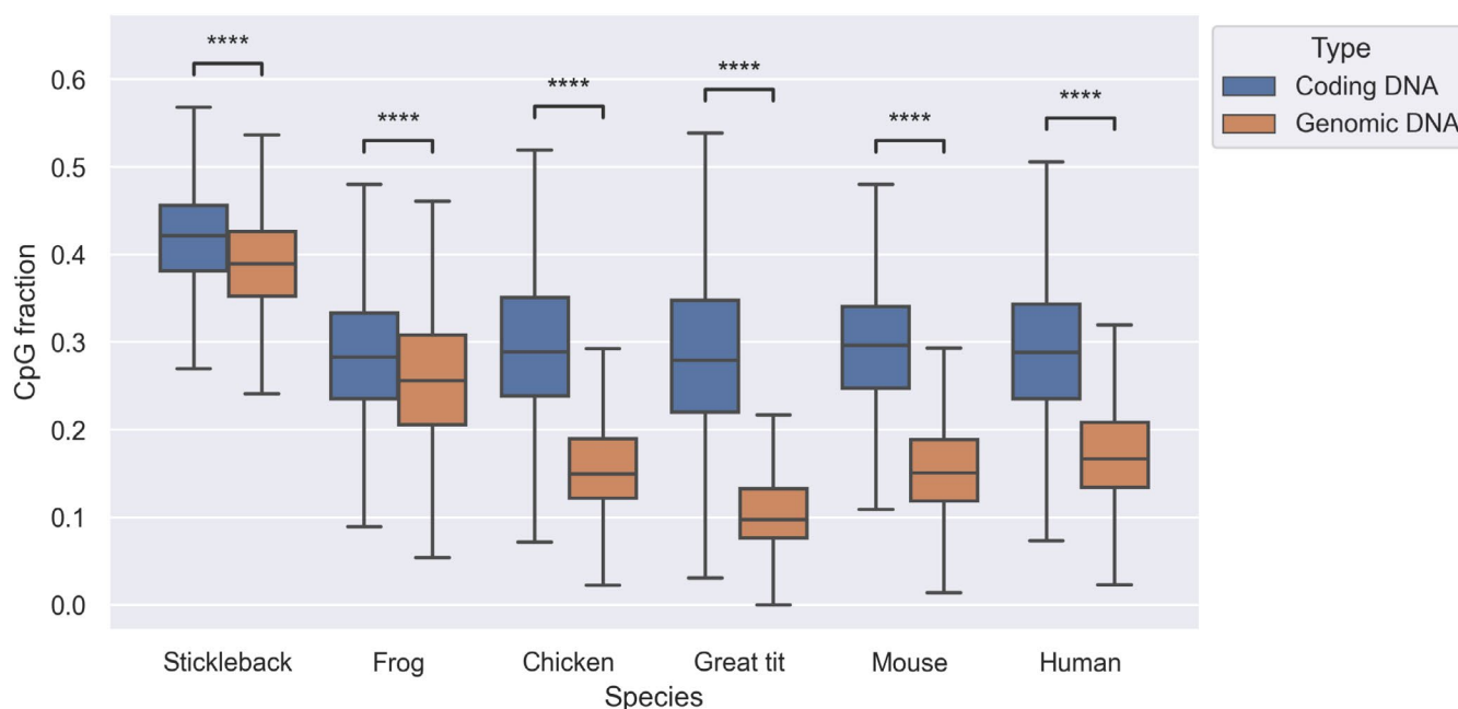
FIGURE 4 | CpG content in different vertebrate species summed across the genome. CpG content is measured as the fraction of CpG sites in GpC and CpG dinucleotides. Shown are protein coding DNA (Coding DNA, blue) and the entire genomes (Genomic DNA, orange). Statistical differences were assessed with a Mann–Whitney- U test, **** p \leq 10^{-4} .
