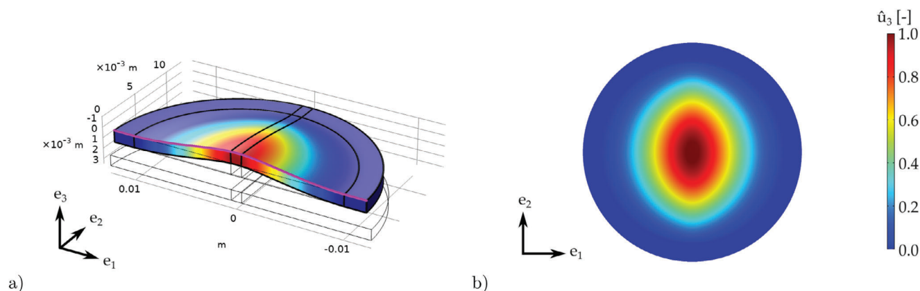
Figure 4. Normalized out-of-plane displacement field \hat{u}_3 = u_3 / \max(u_3) of the bidirectionally magnetized membrane obtained from a numerical simulation with a FE model. a) FE model of the membrane and the stiff permanent magnet (sectional view) where \hat{u}_3 is highlighted in color and the membrane is shown in the deformed state; the pink line illustrates the locations on which the out-of-plane displacement is qualitatively evaluated (cf. Figure 5). b) Top view on the normalized displacement field at the membrane top surface.
