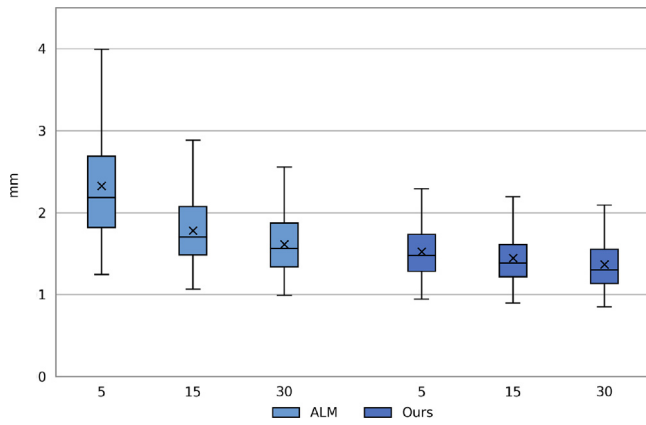
Fig. 10. A quantitative comparison of AnaConDaR against ALM [2] based on synthesized ground truth (Section 4.4). The results are grouped by the number of available target examples and reported in terms of the L2 error (mm). AnaConDaR outperforms ALM in each scenario.
