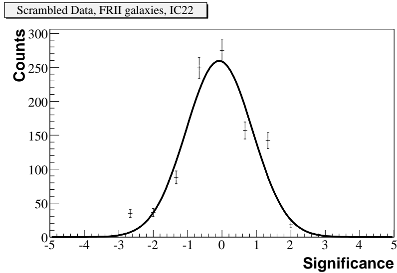
Figure B.44: Distribution of the median significance for 1000 scrambled data sets. It follows a Gaussian distribution with a mean of 0.
