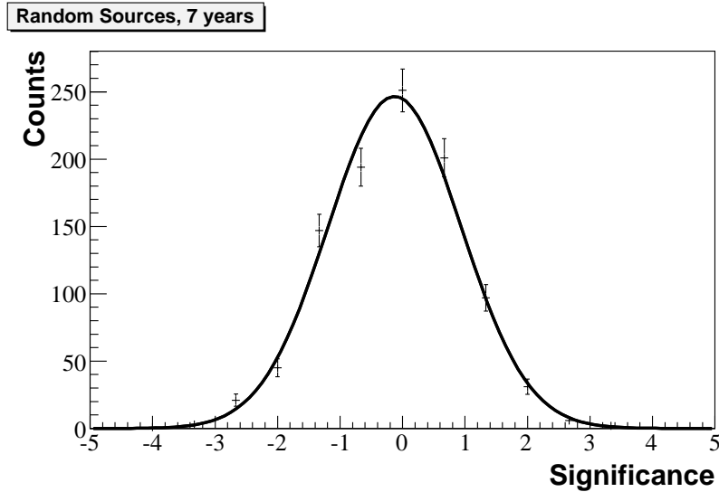
Figure B.35: Significance distribution in an analysis with 1000 randomized source catalogs.
