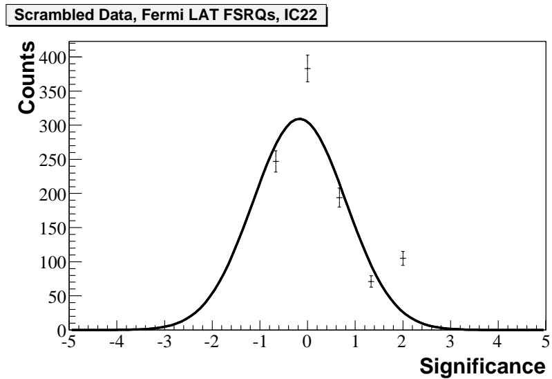
Figure B.49: Distribution of the median significance for 1000 scrambled data sets. It follows a Gaussian distribution with a mean of 0.
