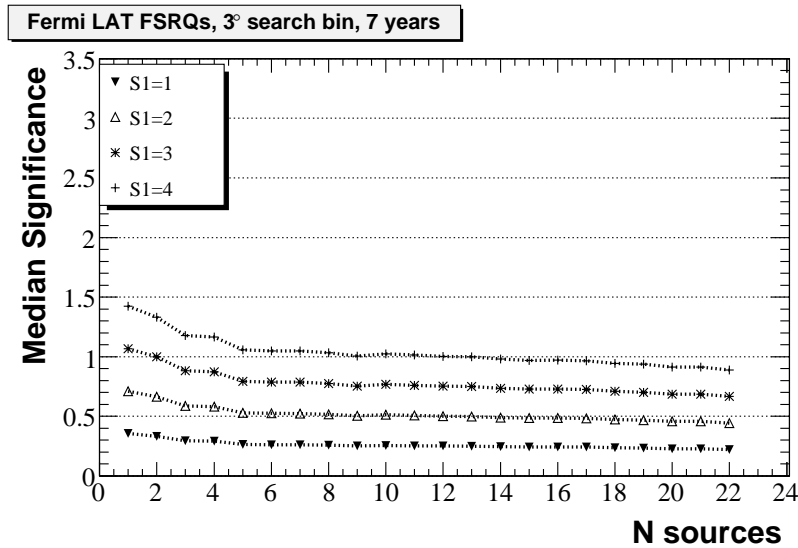
Figure B.26: The sample is dominated by the strongest source, the significance is always decreasing.
