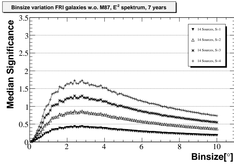
Figure B.14: Search bin variation for FR-I sources. The optimal search bin is 2.4°.
