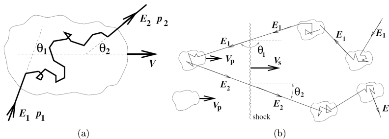
Figure 2.2: On the left (a) there is an illustration of the second order Fermi mechanism, the more effective first order mechanism is displayed on the right side (b) [Pro98].
