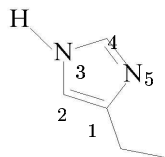
Abbildung 3.9: His (protoniert)
