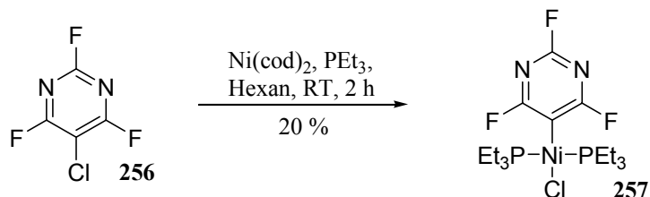
Schema 114: Oxidative Addition von Ni(cod) 2 an 5-Chlor-2,4,6-trifluorpyrimidin ( 256 ). [233]
