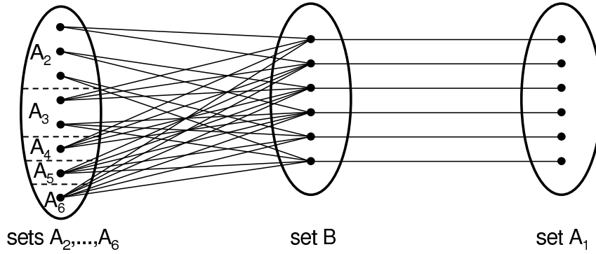
Figure 2: An illustration of Graph 2 for k = 6 .
