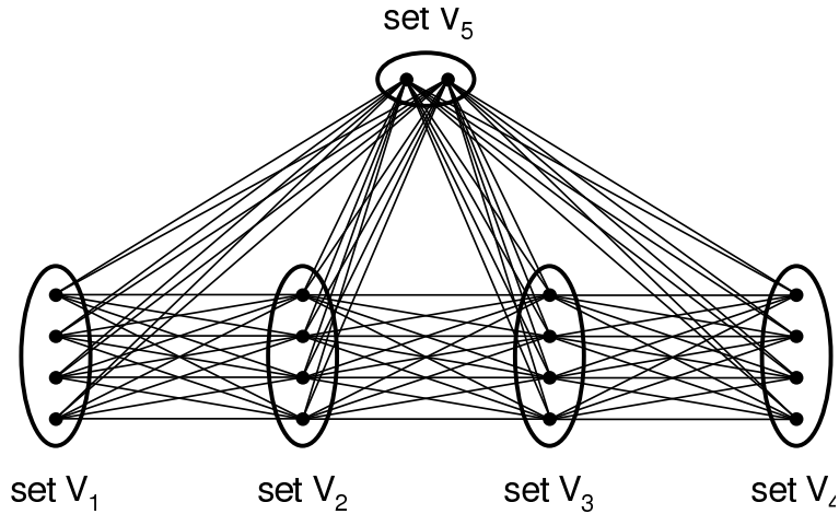
Figure 4: An illustration of Graph 4 for k = 4 .
