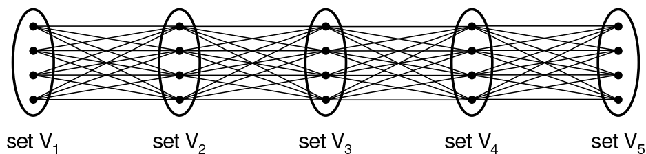
Figure 3: An illustration of Graph 3 for k = 4 .
