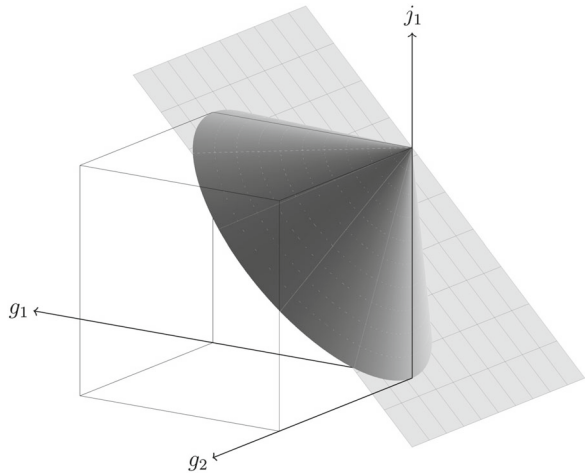
Fig. 2 Three dimensional illustration of the cone C and part of the plane \mathcal{D}_{loc}^A in the g_1, g_2, j_1 space for A = \text{id}
