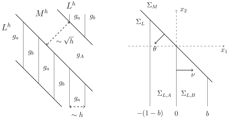
Fig. 3 Left: A sketch of the iterated laminate. Right: The local geometry as considered in Step 3
