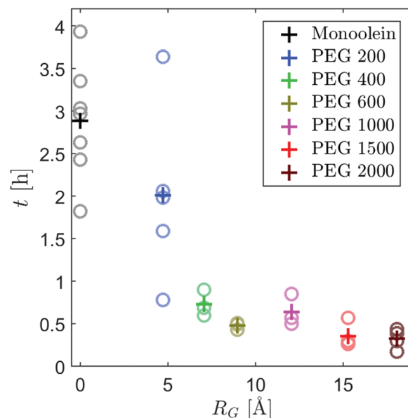
Fig. 4 Period t after a pressure-jump until the released water volume per time and Pn3m unit cell decreased below a limit of 30 \text{ \AA}^3 \text{ s}^{-1} as a function of the radius of gyration R_G of the added PEG as a measure for the speed of the equilibration dynamics. The results for pure monoolein are shown at R_G = 0 for comparison. The circles represent the obtained values of different samples to illustrate the variance. The crosses mark the mean values.
