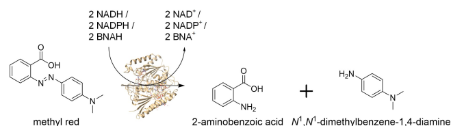
Figure 1. Schematic illustration of the catalyzed cleavage of the azo bond by an azoreductase using different co-substrates as electron donors (enzyme crystal structure of AzoRo, PDB ID: 7AWV).
