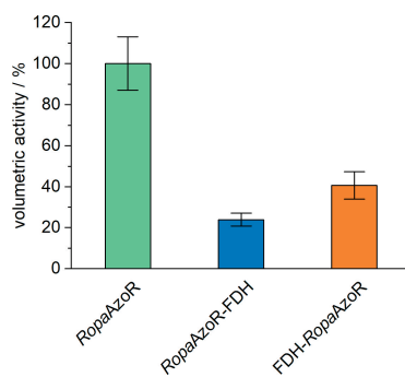
Figure 4. Volumetric activities for RopaAzoR and fusion proteins consisting of RopaAzoR and a formate dehydrogenase (FDH) from Candida boidinii . Values were normalized to RopaAzoR , which corresponds to 100% activity. Activity assays were carried out in a 96-well microplate with a total volume of 100 \mu\text{L} , consisting of 10% (v/v) CFPS-reaction solution and the assay solution with following final concentrations: 100 mM sodium phosphate buffer (pH 6), 50 \mu\text{M} FMN, 30 \mu\text{M} methyl red, and 150 \mu\text{M} NADH. Reactions were incubated at 25 ^{\circ}\text{C} and the degradation of methyl red was monitored by UV-vis spectrophotometry at 430 nm. Error bars are a result of duplicates. Duplicates are from two independent activity assays with enzymes derived from the same synthesis batch.
