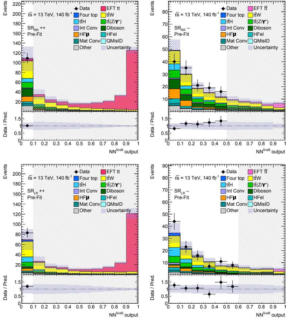
Figure 5.11: NN^{SvsB} output distribution for data and MC events in the 4 defined Signal Regions: SR_{RR}^{++} , SR_{RR}^{--} , SR_{LR}^{++} , SR_{LR}^{--} . Data events are not shown in bins with S/B > 5\% . The bottom panels show the data/MC agreement. The blue dashed band includes both statistical and systematic uncertainties.
