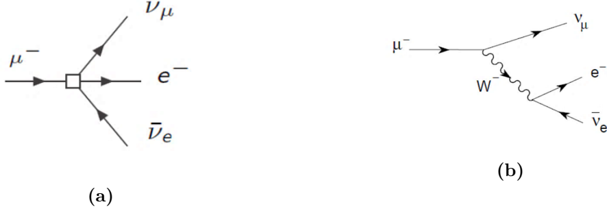
Figure 2.1: The \mu^- \rightarrow e^- \bar{\nu}_e \nu_\mu weak process described by the Fermi Theory (2.1a) and by the SM electroweak gauge theory (2.1b).
