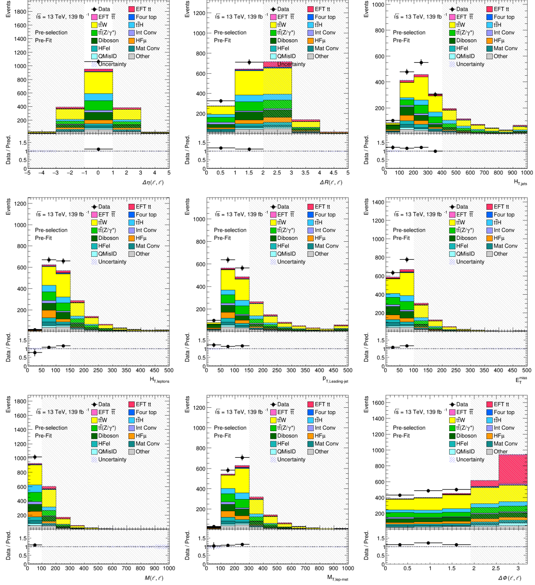
Figure E.3: Kinematic distributions of data and MC events related to the 9 input variables of \text{NN}^{\text{SvsS}} in the \Delta\Phi < 2.5 region. From top left to bottom right: \Delta\eta(\ell, \ell) , \Delta R(\ell, \ell) , H_{T,jets} , H_{T,leptons} , p_{T,LeadingJet} , E_T^{miss} , M(\ell, \ell) and M_{T,lep-met} . The distribution related to \Delta\Phi(\ell, \ell) is obtained by only applying the preliminary signal-like event selection. The bottom panels display the ratio between data and MC yields. Data events are not shown in bins where S/B \geq 5\% .
