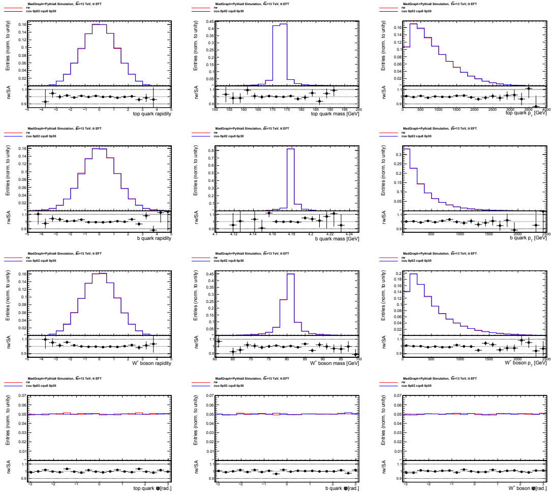
Figure C.14: Truth-level reweighting validation related to the additional tt sample generated with c_{RR} = 0.02 , c_{LR}^{(1)} = 0 , c_{LR}^{(8)} = 0.3 . The red and blue lines show the distribution resulting from the nominal and the reweighted samples respectively. All distributions are normalized to unity. The bottom panels show the ratio between the nominal and reweighted sample entries.
