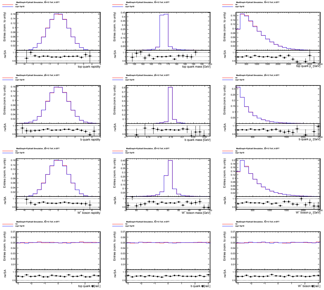
Figure C.4: Truth-level reweighting validation related to the additional tt sample generated with c_{LR}^{(1)} = 0.1 , c_{RR} = c_{LR}^{(8)} = 0 . The red and blue lines show the distribution resulting from the nominal and the reweighted samples respectively. All distributions are normalized to unity. The bottom panels show the ratio between the nominal and reweighted sample entries.
