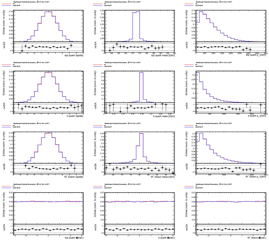
Figure C.6: Truth-level reweighting validation related to the additional tt sample generated with c_{LR}^{(8)} = 0.1 , c_{RR} = c_{LR}^{(1)} = 0 . The red and blue lines show the distribution resulting from the nominal and the reweighted samples respectively. All distributions are normalized to unity. The bottom panels show the ratio between the nominal and reweighted sample entries.
