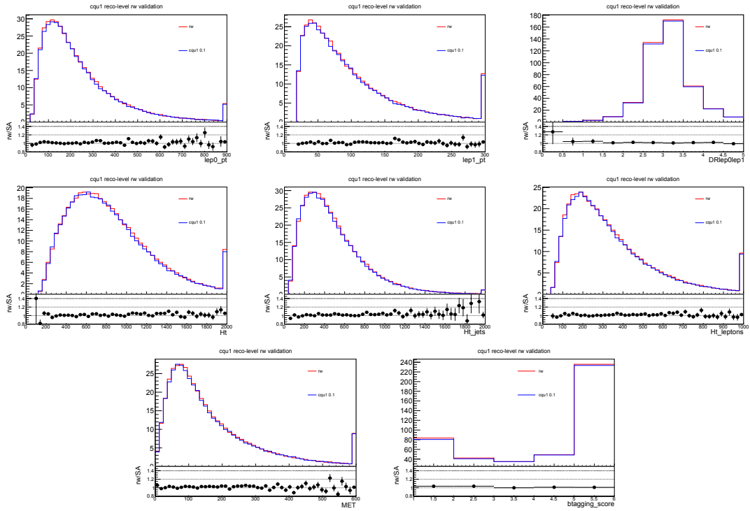
Figure C.16: Reco-level reweighting validation related to the additional tt sample generated with c_{LR}^{(1)} = 0.1 , c_{RR} = c_{LR}^{(8)} = 0
