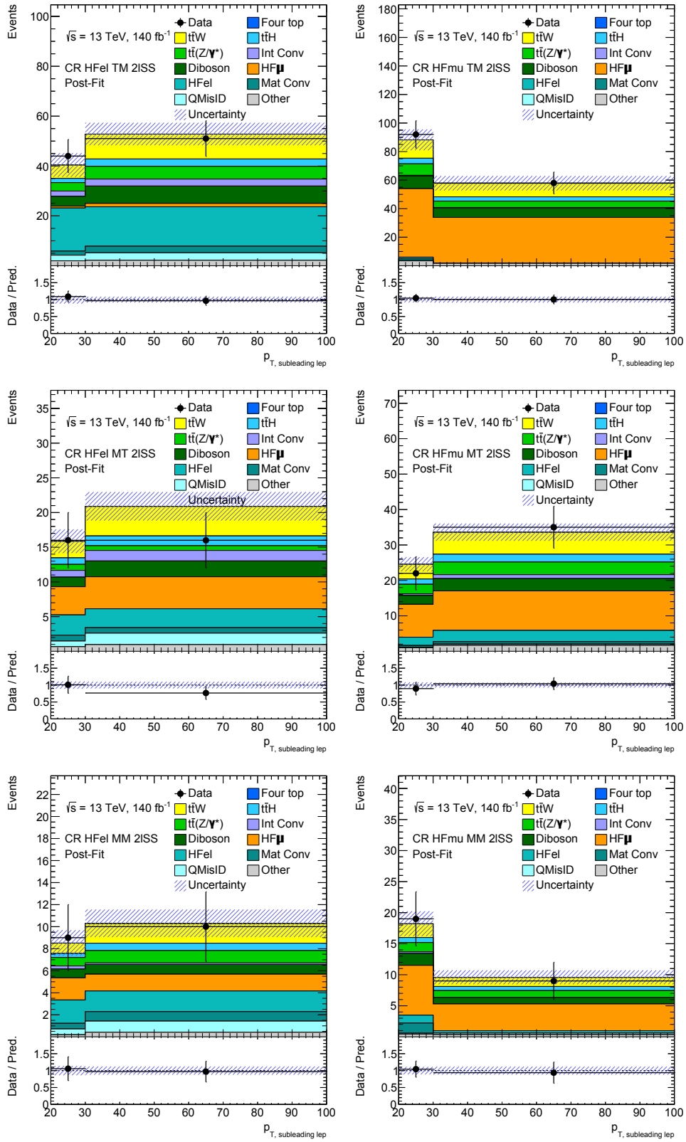
Figure 5.34: Post-fit distributions in the analysis HF -CRs of the variables used in the fit performed on Run 2 data. The blue hashed bands include both statistical and systematic uncertainties. The bottom panels display the ratio between observed and expected event yields, used to assess the post-fit data/MC agreement.
