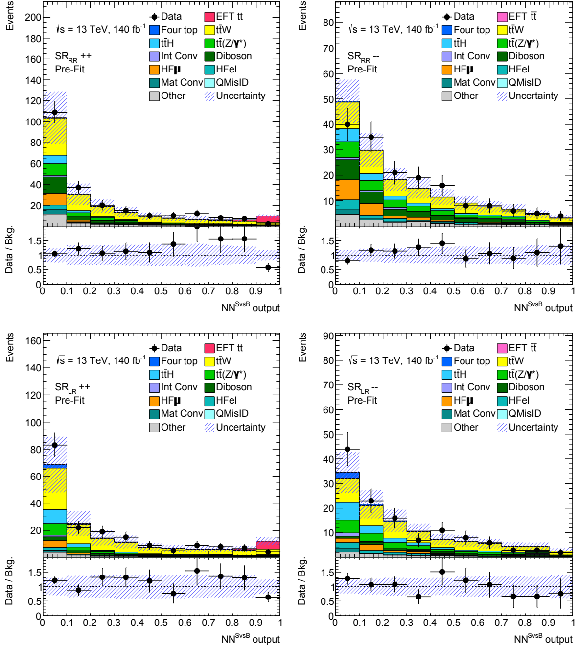
Figure 5.27: Unblinded distributions of the \text{NN}^{\text{SvsB}} output in the analysis SRs. The signal prediction is normalized according to the analysis expected sensitivity. The blue hashed bands include both statistical and systematic uncertainties. The bottom panels show the ratio between data and background prediction.
