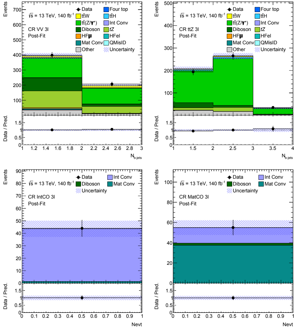
Figure 5.33: Post-fit distributions in the analysis VV , t\bar{t}Z , IntCO and MatCO CRs of the variables used in the fit performed on Run 2 data. The blue hashed bands include both statistical and systematic uncertainties. The bottom panels display the ratio between observed and expected event yields, used to assess the post-fit data/MC agreement.
