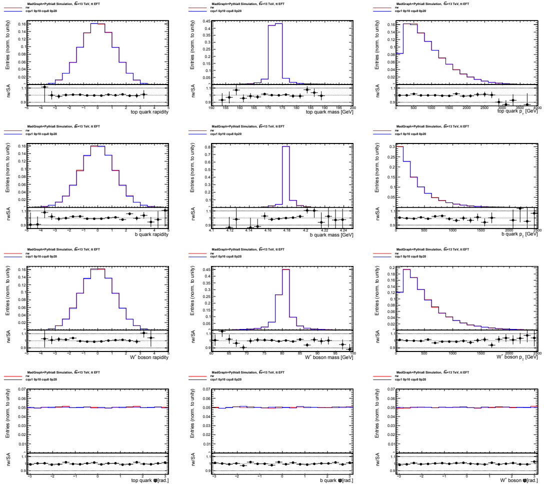
Figure C.8: Truth-level reweighting validation related to the additional tt sample generated with c_{RR} = 0 , c_{LR}^{(1)} = 0.1 , c_{LR}^{(8)} = 0.2 . The red and blue lines show the distribution resulting from the nominal and the reweighted samples respectively. All distributions are normalized to unity. The bottom panels show the ratio between the nominal and reweighted sample entries.
