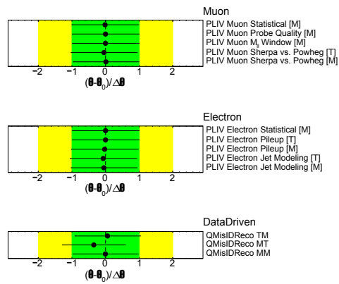
Figure 5.31: Pulls and constraints on the muon (top) and electron (middle) PLIV as well as on the data driven QMisID (bottom) related nuisance parameters resulting from the S+B fit to the Run 2 collision data performed over all analysis regions.
