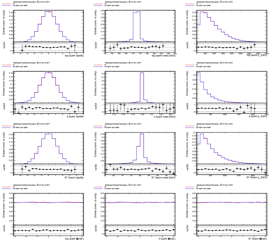
Figure C.10: Truth-level reweighting validation related to the additional tt sample generated with c_{RR} = 0.01 , c_{LR}^{(1)} = 0.05 , c_{LR}^{(8)} = 0 . The red and blue lines show the distribution resulting from the nominal and the reweighted samples respectively. All distributions are normalized to unity. The bottom panels show the ratio between the nominal and reweighted sample entries.
