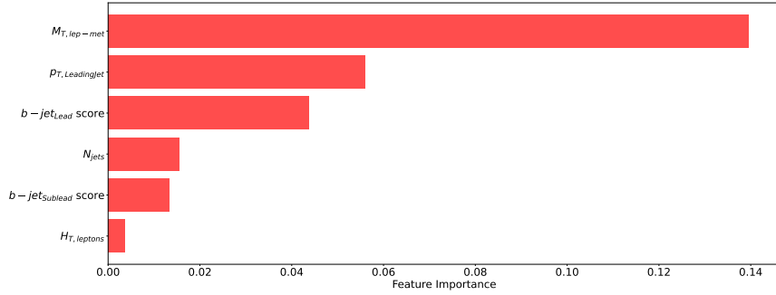
Figure E.8: NN^{SvsB} input variable ranking for SR_{LR} .
