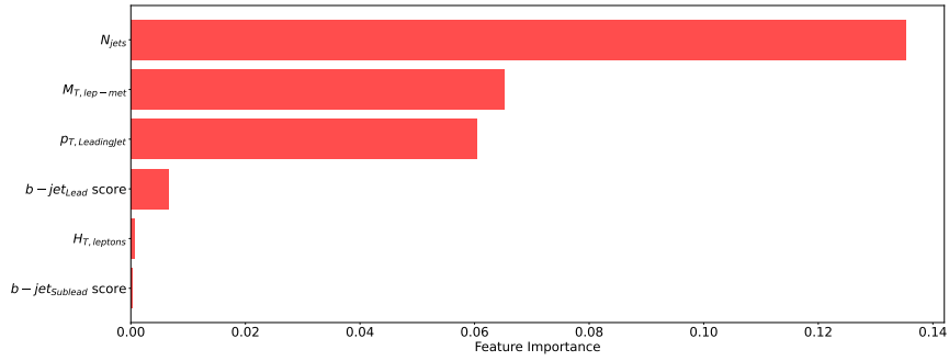
Figure E.7: NN^{SvsB} input variable ranking for SR_{RR} .
