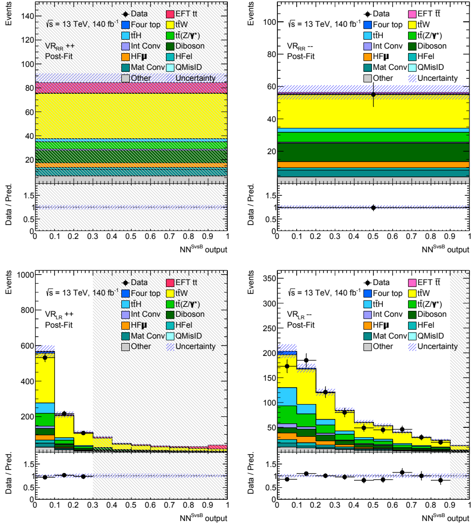
Figure 5.21: Post-fit distributions in the analysis VRs. The background-only fit has been performed over the CRs and the unblinded bins of the SRs. The blue hashed band includes both statistical and systematic uncertainties. The bottom panels display the ratio between observed and expected event yields. Data events are displayed only in bins with S/B < 5\% .
