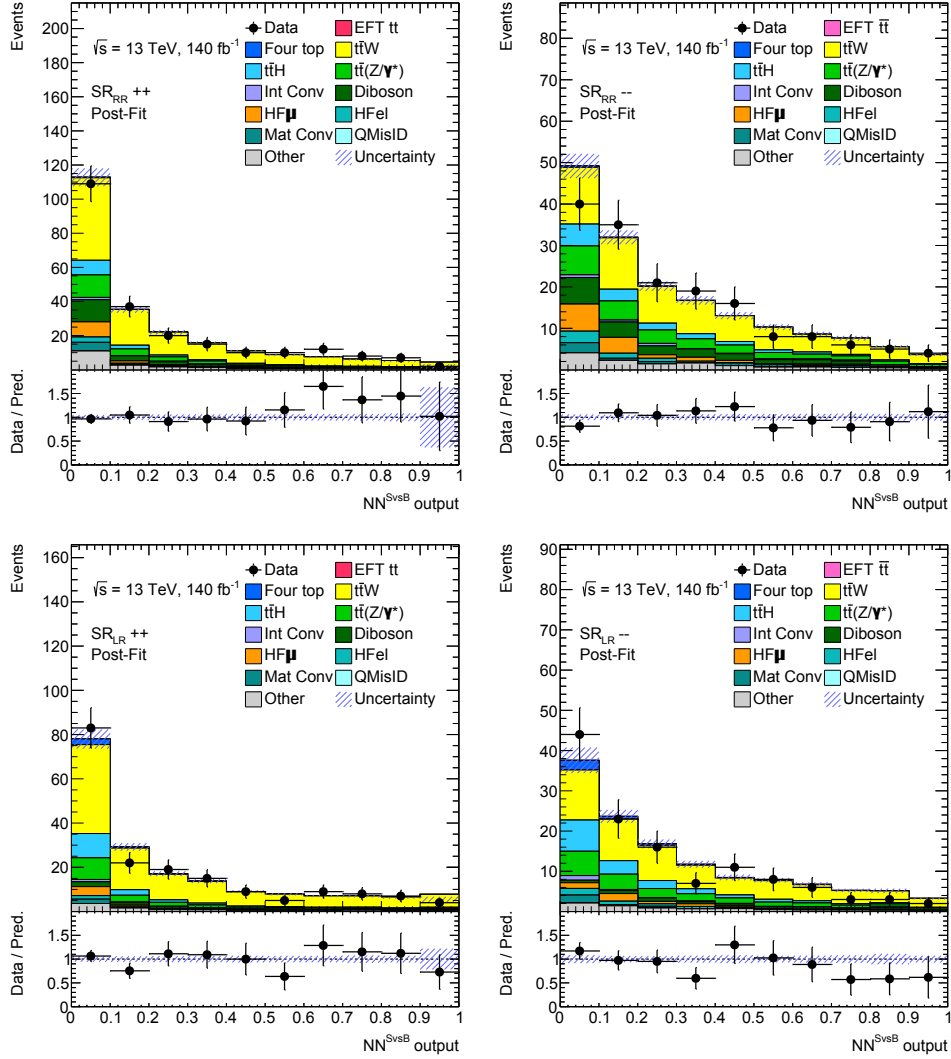
Figure 5.37: Post-fit distributions of the \text{NN}^{\text{SvsB}} output in the analysis SRs. The signal is normalized according to the analysis expected sensitivity. The fit is performed on Run 2 data. The blue hashed bands include both statistical and systematic uncertainties. The bottom panels show the ratio between data and MC yields.
