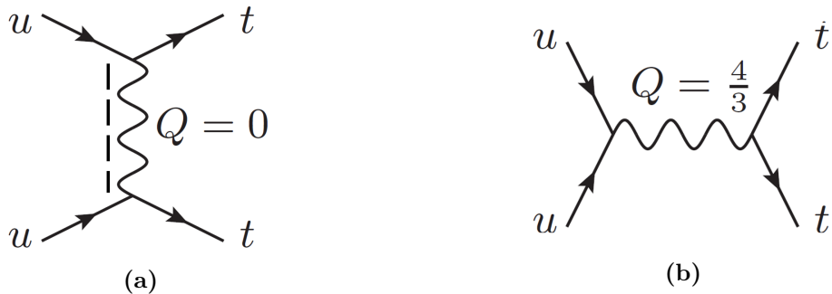
Figure 3.2: Same-sign top pairs t-channel (3.2a) and s-channel (3.2b) production.
