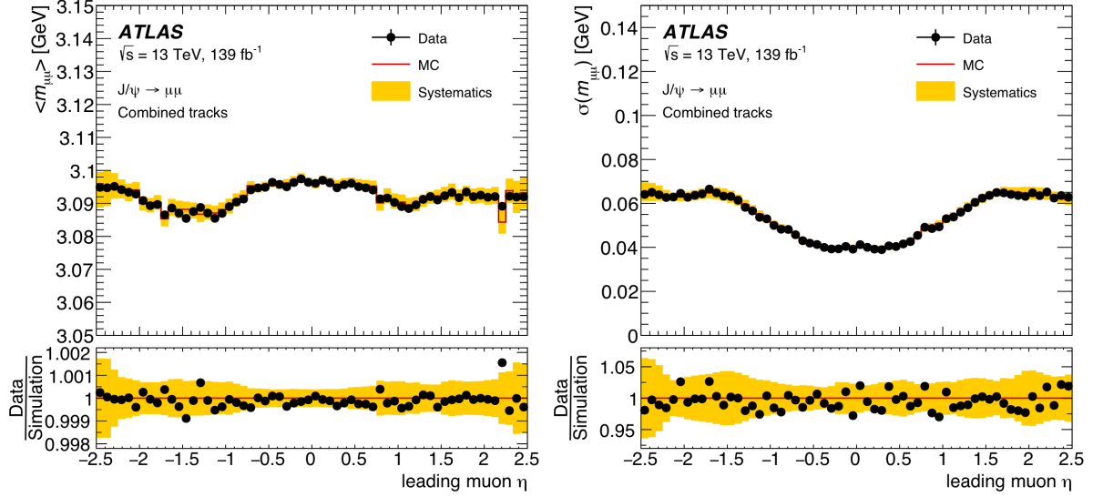
Figure B.7: Mean and width values resulting from the fit on data and corrected simulation using CB muons in J/\psi \rightarrow \mu\mu events. The values are shown as a function of the pseudorapidity of the leading muon with associated errors. The bottom panels show data/MC ratio.
