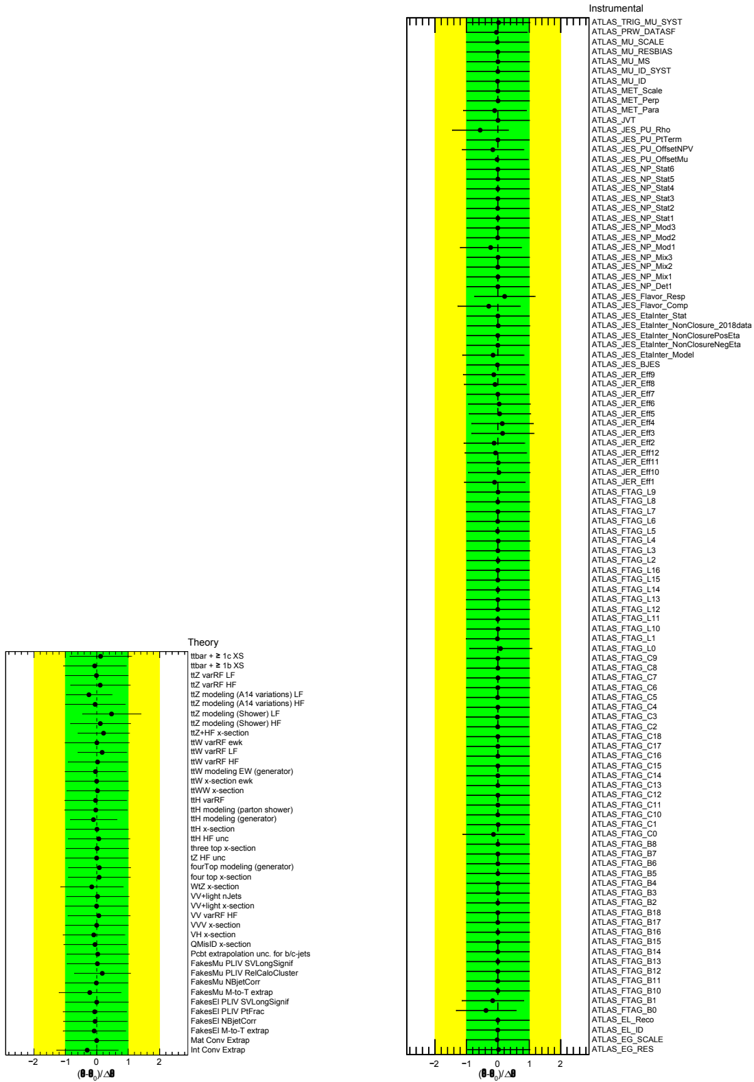
Figure 5.30: Pulls and constraints on the theory nuisance parameters (left) and on the instrumental nuisance parameters (right) resulting from the S+B fit to the Run 2 collision data performed over all analysis regions.
