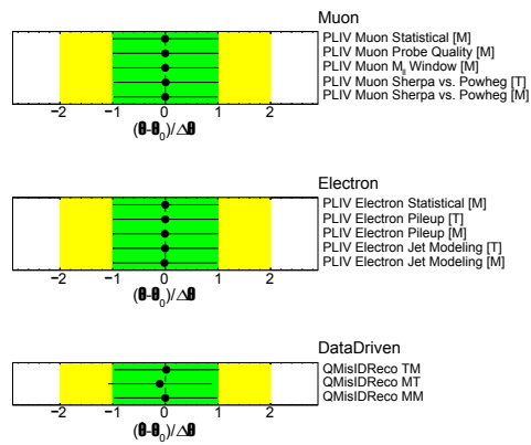
Figure 5.26: Pulls and constraints on the muon (top) and electron (middle) PLIV as well as on the data driven QMisID (bottom) related nuisance parameters resulting from a S+B fit to the Asimov dataset in all analysis regions.
