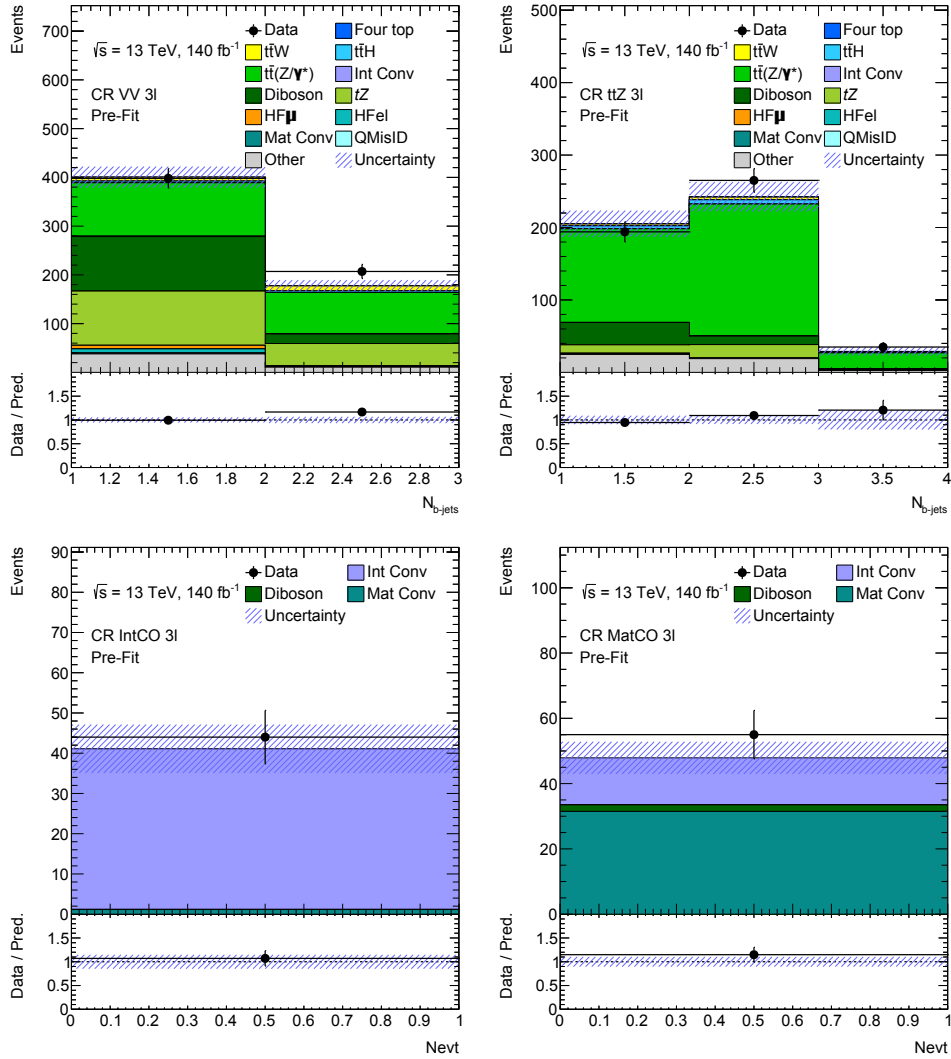
Figure 5.13: Distributions of the variables related to the CRs used in the analysis to estimate the backgrounds related to t\bar{t}Z and VV processes (top row) and non-prompt leptons from photon conversion (bottom row). The blue hashed band includes both statistical and systematic uncertainties. The bottom panels display the data/MC ratio.
