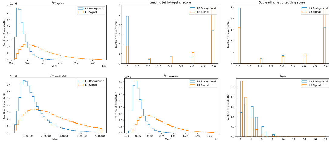
Figure E.6: Kinematic distributions related to the 6 input variables of NN^{SvsB} for events in SR_{LR} . From top left to bottom right: H_{T,leptons} , b-tagging score of the leading jet, b-tagging score of the subleading jet, p_{T,LeadingJet} , M_{T,lep-met} and n_{Jets} . Signal and background distributions are reported in orange and blue respectively. All distribution are normalized to unity.
