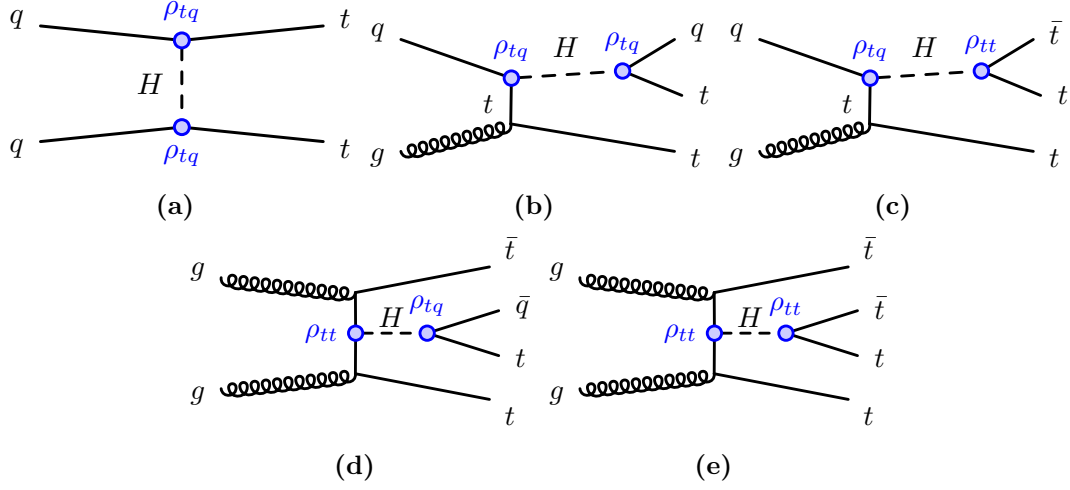
Figure A.1: Signal diagrams for the production and decay modes of the heavy scalar considered in the analysis. The couplings of the heavy H with SM particles are shown as well.
