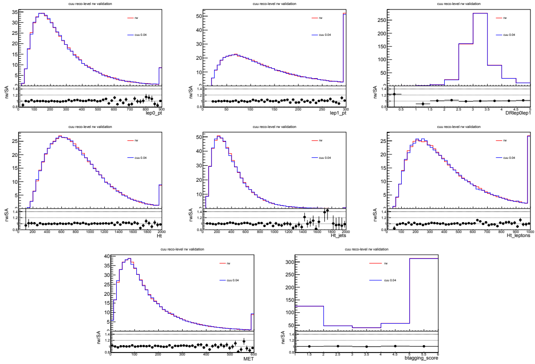
Figure C.15: Reco-level reweighting validation related to the additional tt sample generated with c_{RR} = 0.04 , c_{LR}^{(1)} = c_{LR}^{(8)} = 0
