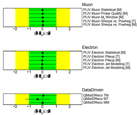
Figure 5.23: Pulls and constraints on the muon (top) and electron (middle) PLIV as well as on the data driven QMisID (bottom) related nuisance parameters resulting from a background-only fit performed over the 10 CRs and the unblinded bins of the SRs.
