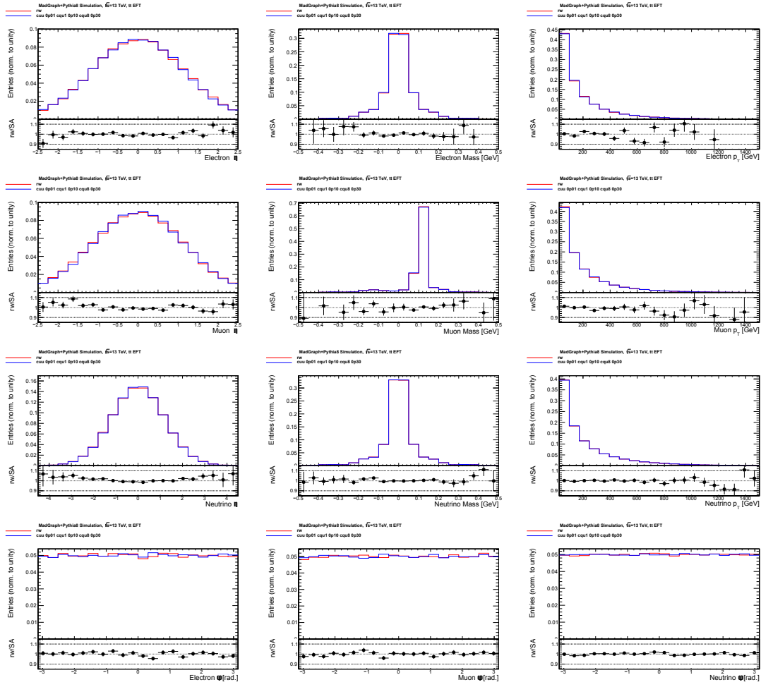
Figure C.11: Truth-level reweighting validation related to the additional t\bar{t} sample generated with c_{RR} = 0.01 , c_{LR}^{(1)} = 0.1 , c_{LR}^{(8)} = 0.3 . The red and blue lines show the distribution resulting from the nominal and the reweighted samples respectively. All distributions are normalized to unity. The bottom panels show the ratio between the nominal and reweighted sample entries.
