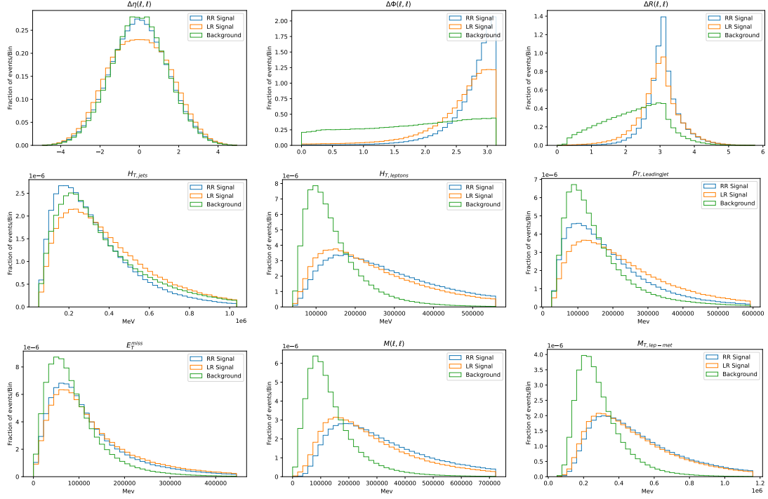
Figure E.1: Kinematic distributions related to the 9 input variables of \text{NN}^{\text{SvsS}} . From top left to bottom right: \Delta\eta(\ell, \ell) , \Delta\Phi(\ell, \ell) , \Delta R(\ell, \ell) , H_{T,jets} , H_{T,leptons} , p_{T,LeadingJet} , E_T^{miss} , M(\ell, \ell) and M_{T,lep-met} . RR signal, LR signal and background distribution are reported in blue, orange and green respectively. All distribution are normalized to unity.
