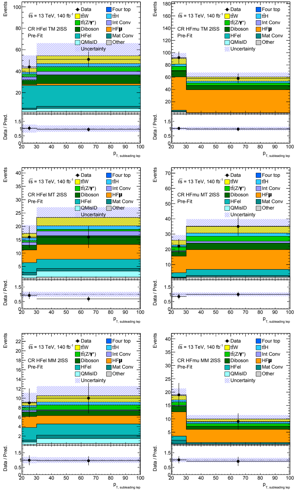
Figure 5.14: Distributions of the variables related to the CRs used in the analysis to estimate the backgrounds related to non-prompt leptons from heavy hadrons decay. From top left to bottom right: HFe TM, HF\mu TM, HFe MT, HF\mu MT, HFe MM and HF\mu MM. The blue hashed band includes both statistical and systematic uncertainties. The bottom panels display the data/MC ratio.
