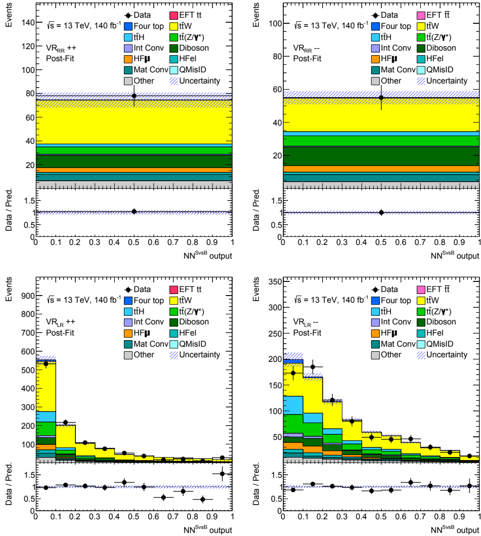
Figure 5.36: Post-fit distributions in the analysis VRs. The fit has been performed on Run 2 data events over all SRs and CRs. The blue hashed bands include both statistical and systematic uncertainties. The bottom panels display the ratio between observed and expected event yields, used to assess the post-fit data/MC agreement.
