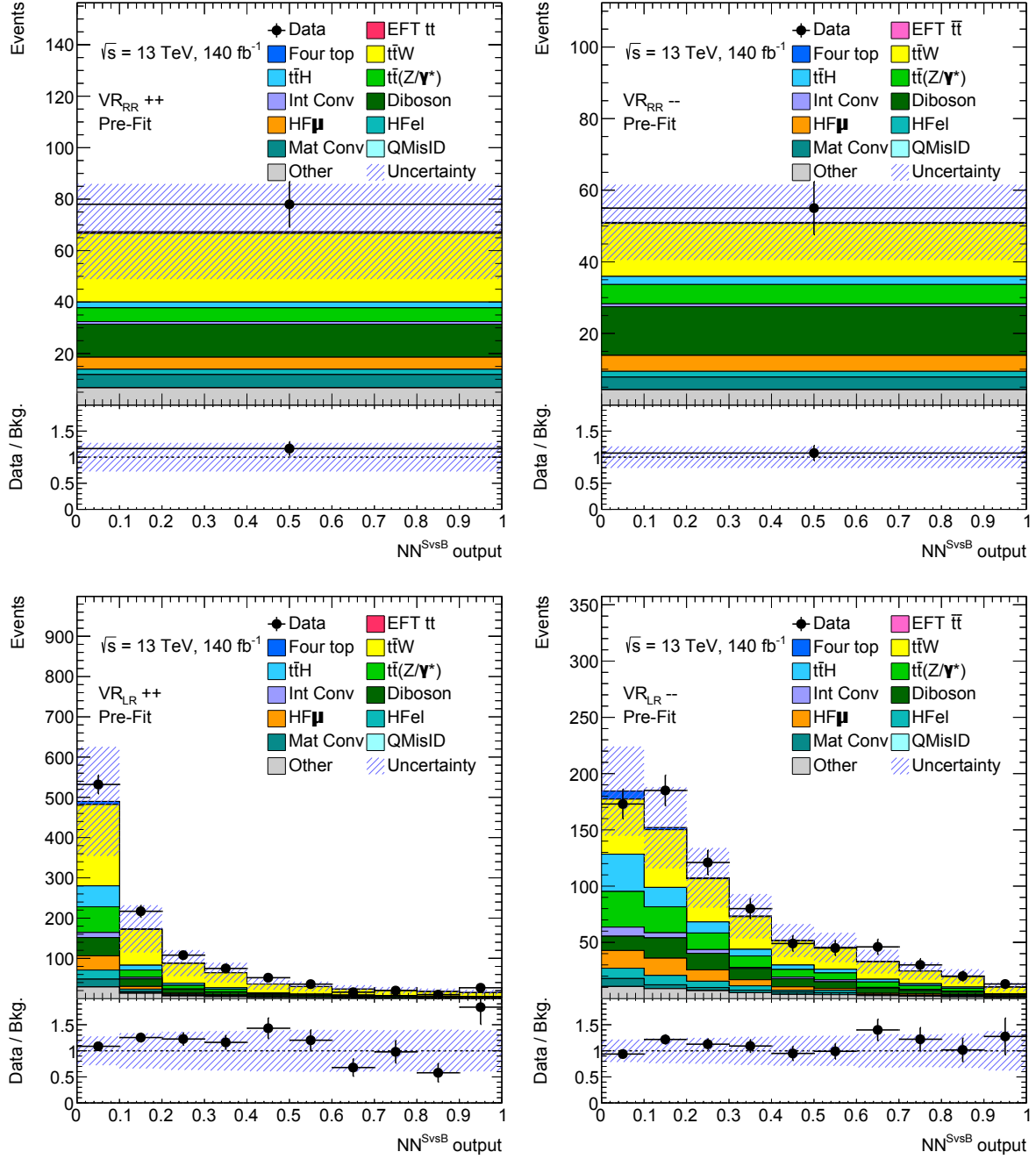
Figure 5.28: Distributions of the \text{NN}^{\text{SvsB}} output in the analysis VRs. The signal prediction is normalized according to the analysis expected sensitivity. The blue hashed bands include both statistical and systematic uncertainties. The bottom panels show the ratio between data and background prediction.
