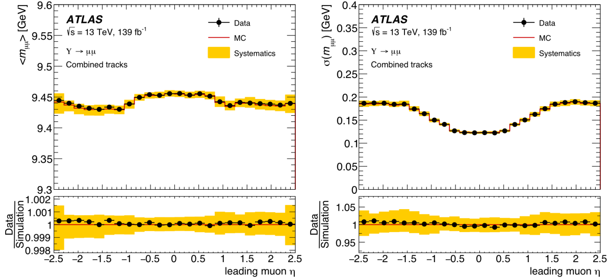
Figure B.8: Mean and width values resulting from the fit on data and corrected simulation using CB muons in Y \rightarrow \mu\mu events. The values are shown as a function of the pseudorapidity of the leading muon with associated errors. The bottom panels show data/MC ratio.
