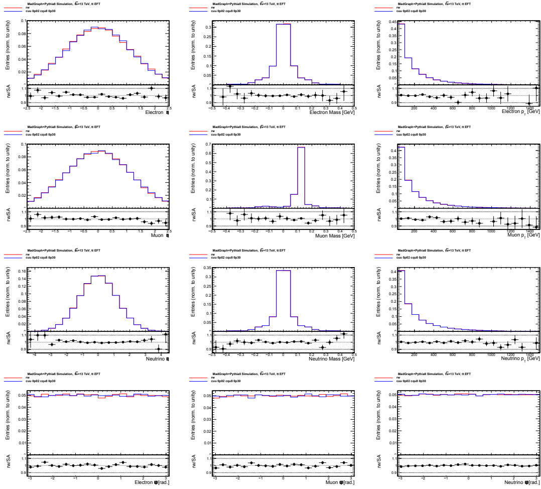
Figure C.13: Truth-level reweighting validation related to the additional tt sample generated with c_{RR} = 0.02 , c_{LR}^{(1)} = 0 , c_{LR}^{(8)} = 0.3 . The red and blue lines show the distribution resulting from the nominal and the reweighted samples respectively. All distributions are normalized to unity. The bottom panels show the ratio between the nominal and reweighted sample entries.
