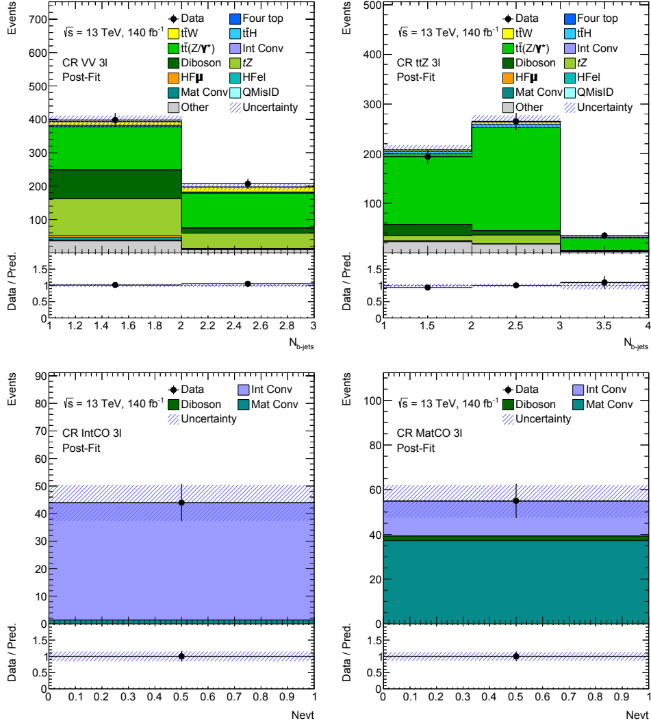
Figure 5.16: Post-fit distributions in VV , t\bar{t}Z , IntCO and MatCO CRs of the variables used in the background-only fit performed over the CRs and the unblinded bins of the SRs. The blue hashed band includes both statistical and systematic uncertainties. The bottom panels display the ratio between observed and expected event yields, used to assess the post-fit data/MC agreement.
