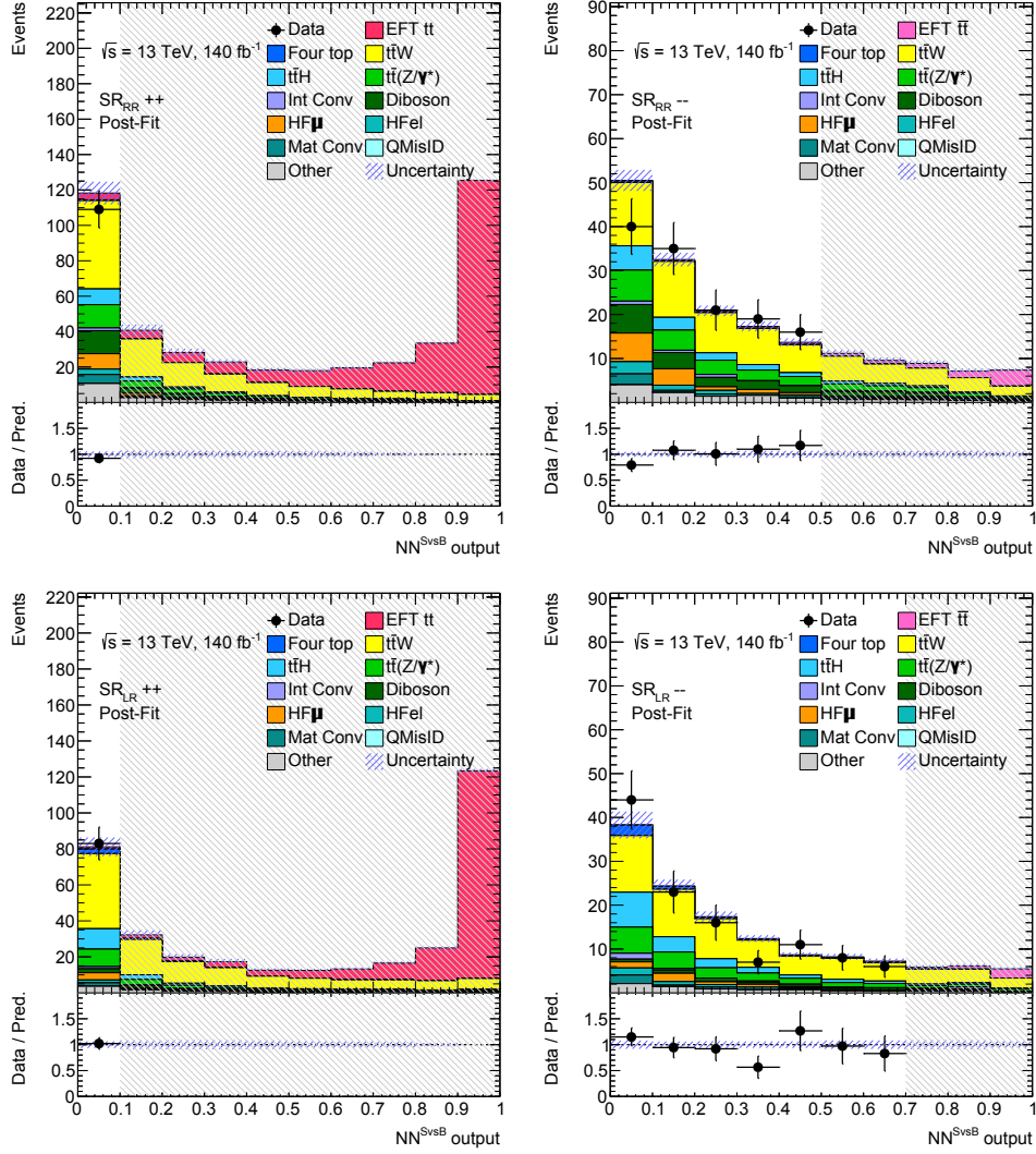
Figure 5.18: Post-fit distributions in the analysis SRs of the \text{NN}^{\text{SvsB}} output used in the background-only fit performed over the CRs and the unblinded bins of the SRs. The blue hashed band includes both statistical and systematic uncertainties. The bottom panels display the ratio between observed and expected event yields, used to assess the post-fit data/MC agreement. Data events are displayed only in bins with S/B < 5\% .
