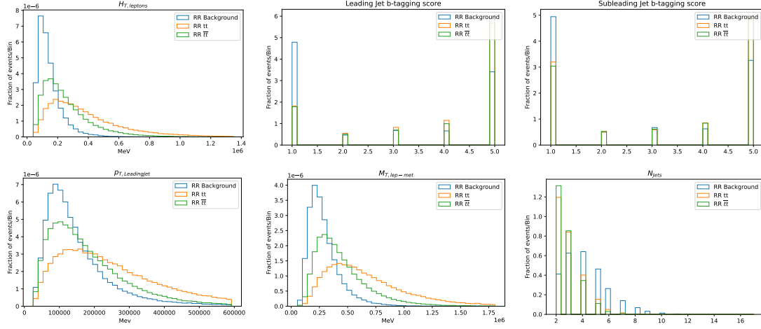
Figure E.10: Kinematic distributions related to the 6 input variables of NN^{SvsB} for events in SR_{RR} . From top left to bottom right: H_{T,leptons} , b-tagging score of the leading jet, b-tagging score of the subleading jet, p_{T,LeadingJet} , M_{T,lep-met} and n_{Jets} . The distributions related to tt , t\bar{t} and background events are reported in orange, green and blue respectively. All distribution are normalized to unity.
