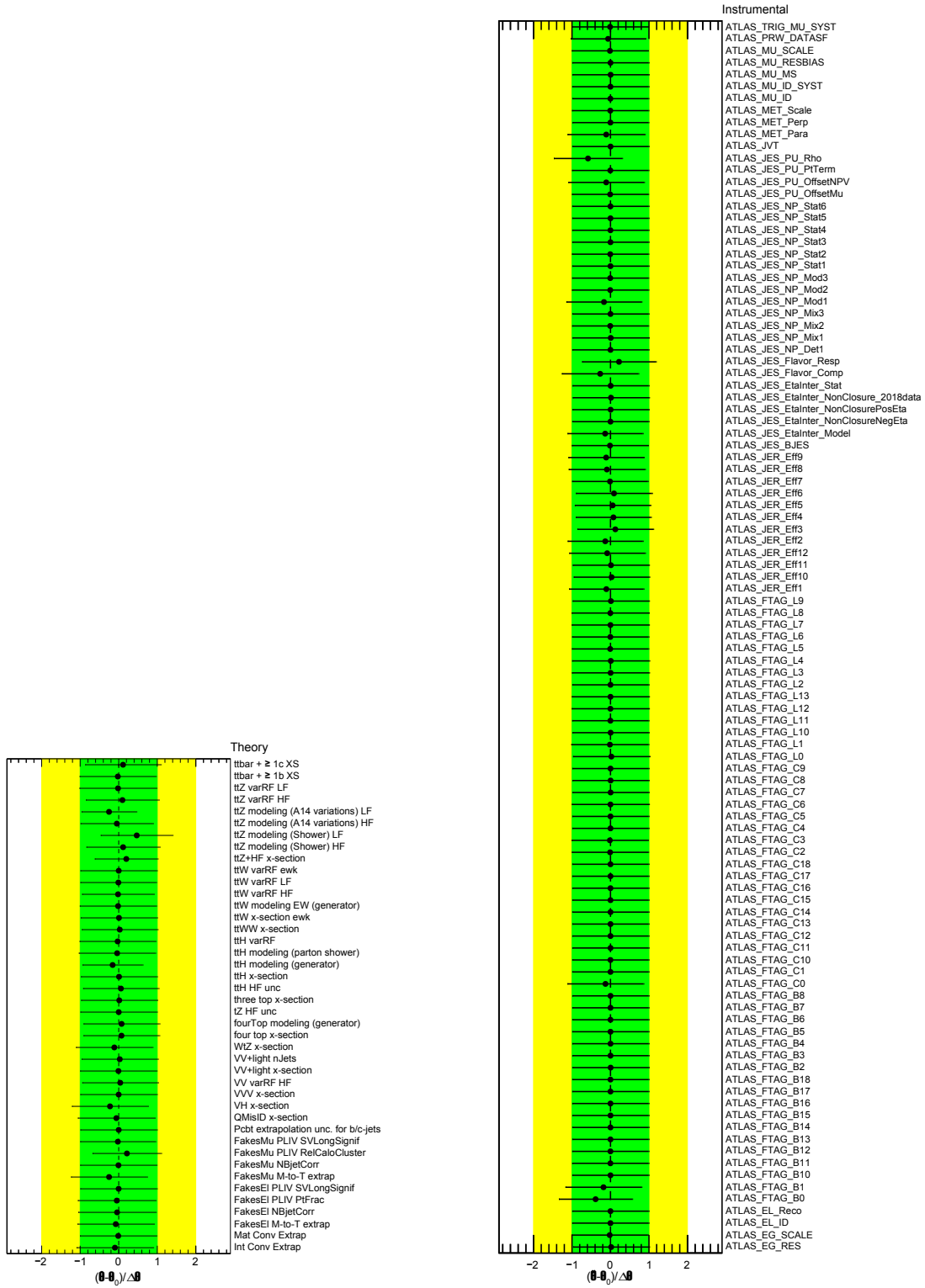
Figure 5.22: Pulls and constraints on the theory nuisance parameters (left) and on the instrumental nuisance parameters (right) resulting from a background-only fit performed over the 10 CRs and the unblinded bins of the SRs.
