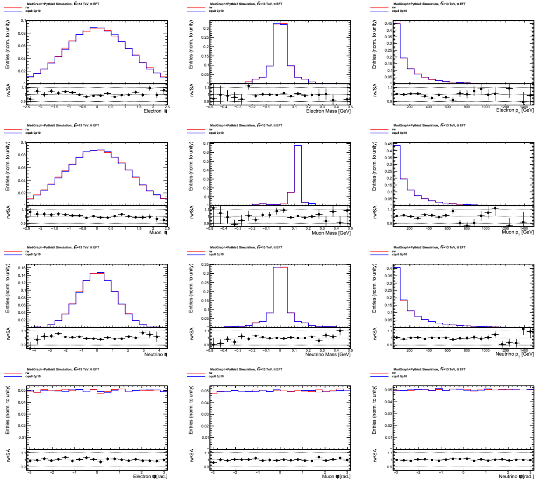
Figure C.5: Truth-level reweighting validation related to the additional tt sample generated with c_{LR}^{(8)} = 0.1 , c_{RR} = c_{LR}^{(1)} = 0 . The red and blue lines show the distribution resulting from the nominal and the reweighted samples respectively. All distributions are normalized to unity. The bottom panels show the ratio between the nominal and reweighted sample entries.
