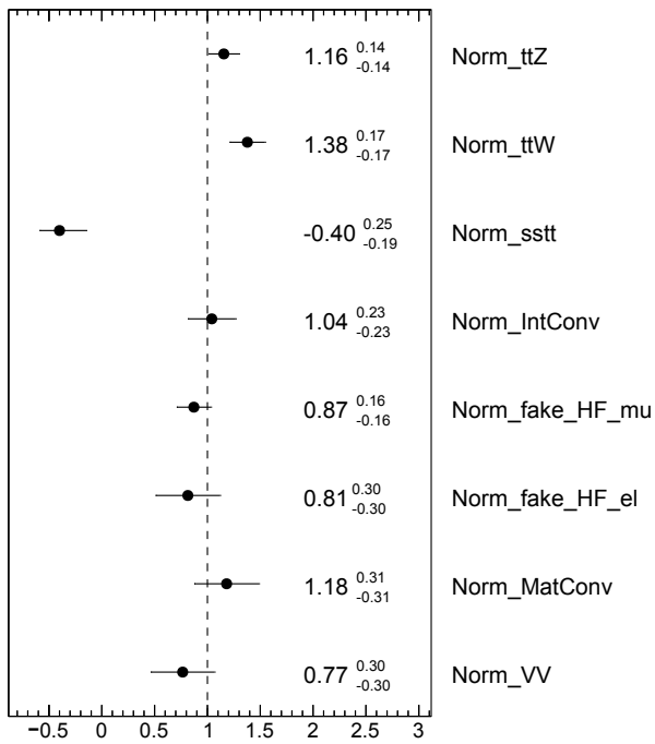
Figure 5.29: Normalization factors resulting from the S+B fit to Run 2 collision data performed over all analysis regions including statistical and systematic uncertainties. The normalization factors are related to the signal and to non-prompt leptons, diboson, t\bar{t}Z and t\bar{t}W backgrounds. All NFs are left free-floating in the fit.
