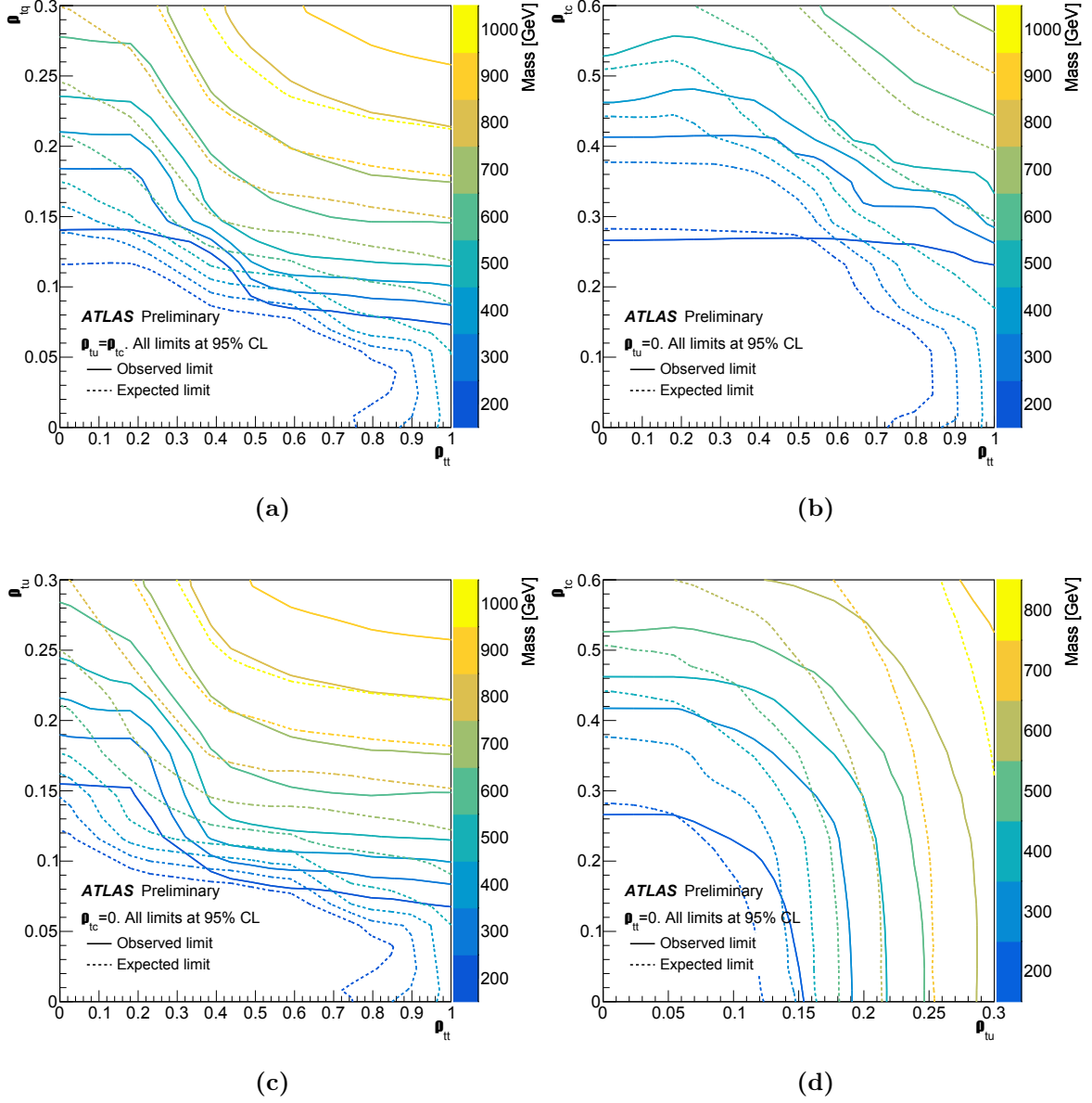
Figure A.4: Observed (solid line) and expected (dashed line) exclusion limits at 95% CL on the heavy Higgs boson mass for the g2HDM as a function of the couplings under different signal benchmarks.
