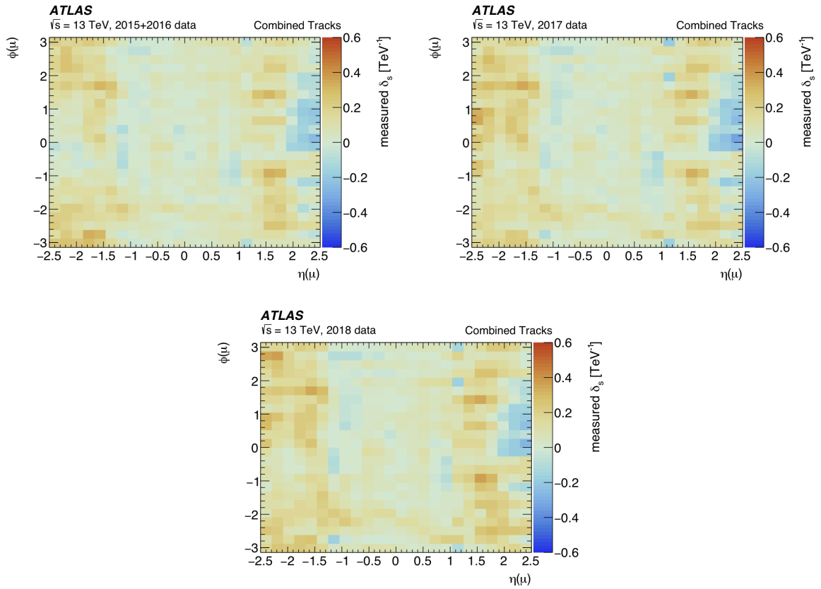
Figure B.5: Charge dependent bias on muon p_T evaluated for CB muons after applying the alignment procedures in Run 2 data for the different data taking years. The corrections have been derived using Z \rightarrow \mu\mu events.
