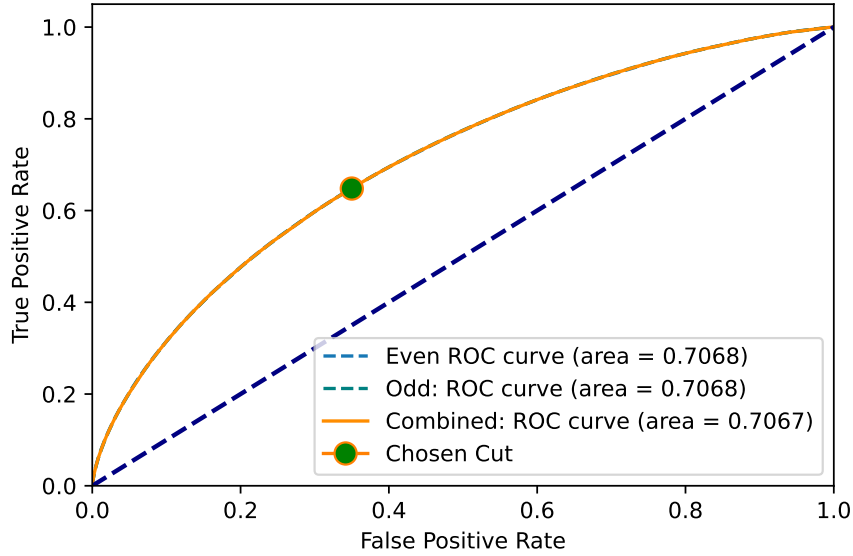
Figure 5.2: \text{NN}^{\text{SvsS}} ROC curve. It can be seen that the performance of the NN is comparable for the even and odd trainings, as expected. The green dot corresponds to the \text{NN}^{\text{SvsS}} output cut chosen to define SR_{RR} and SR_{LR} .
