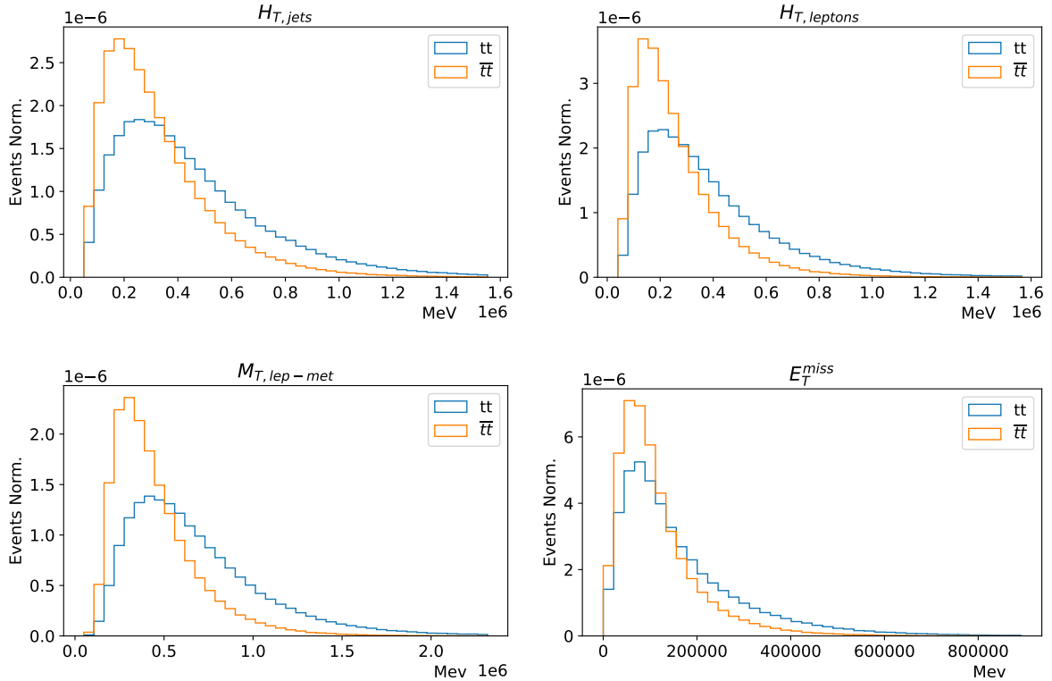
Figure 5.4: The kinematic distributions associated to tt and \bar{t}\bar{t} events are shown as blue and orange lines respectively. From top left to bottom right: H_{T,jets} , H_{T,leptons} , M_{T,lep-met} and E_T^{miss} .
