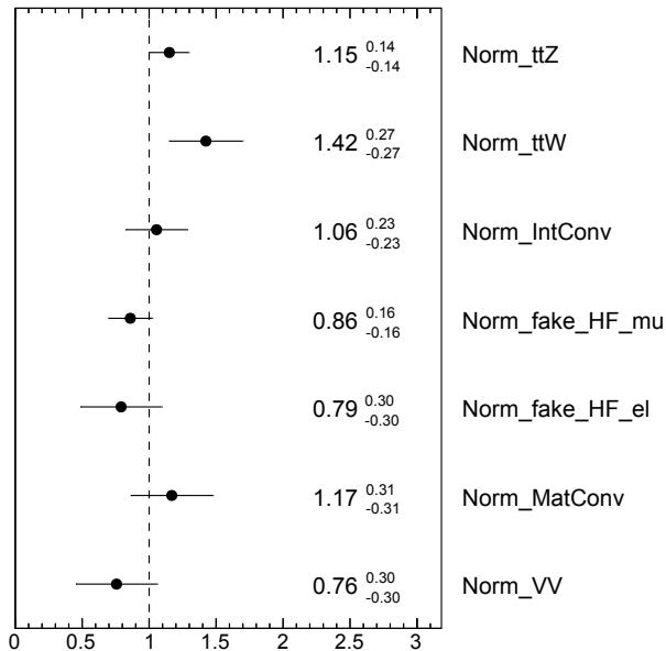
Figure 5.15: Normalization factors resulting from the background-only fit to CRs and to the unblinded bins of the SRs with statistical and systematic uncertainties. The normalization factors are related to the non-prompt leptons, diboson, t\bar{t}Z and t\bar{t}W backgrounds and are left free-floating in the fit.
