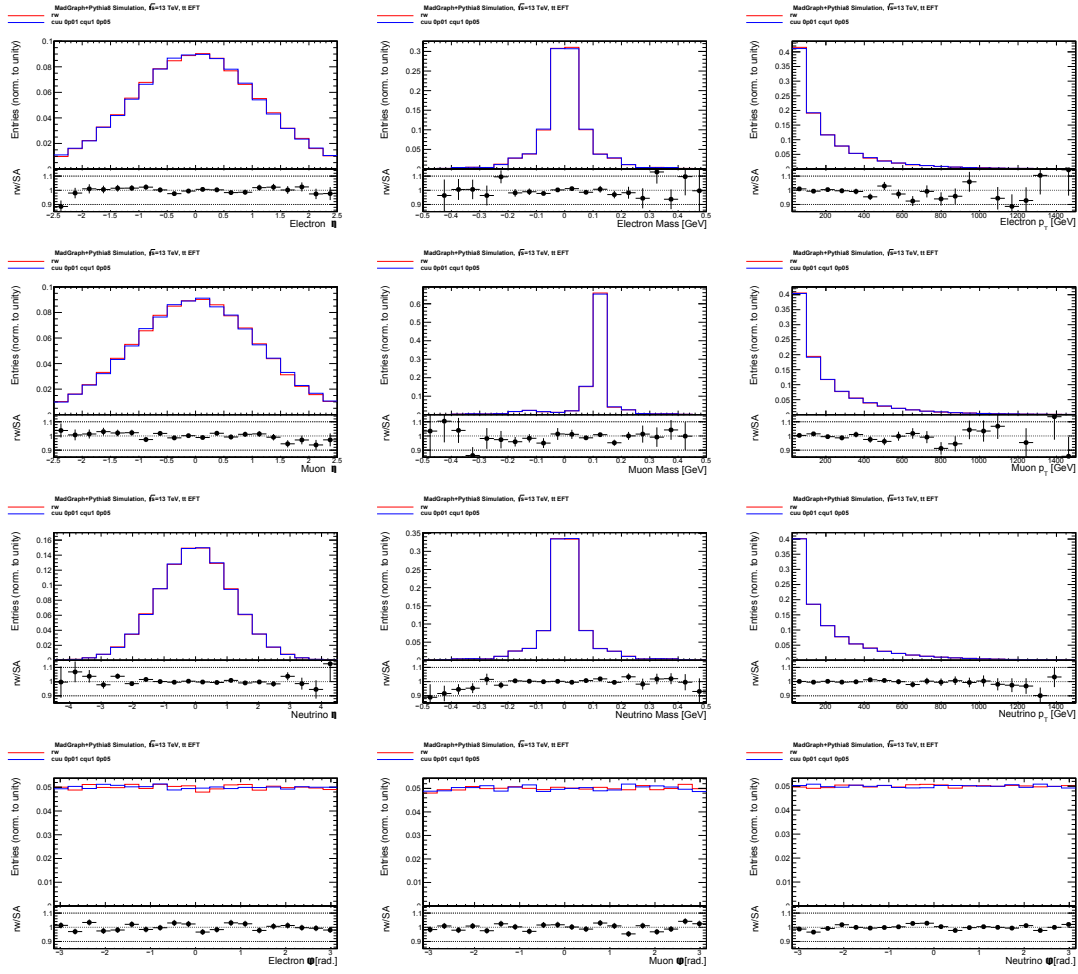
Figure C.9: Truth-level reweighting validation related to the additional tt sample generated with c_{RR} = 0.01 , c_{LR}^{(1)} = 0.05 , c_{LR}^{(8)} = 0 . The red and blue lines show the distribution resulting from the nominal and the reweighted samples respectively. All distributions are normalized to unity. The bottom panels show the ratio between the nominal and reweighted sample entries.
