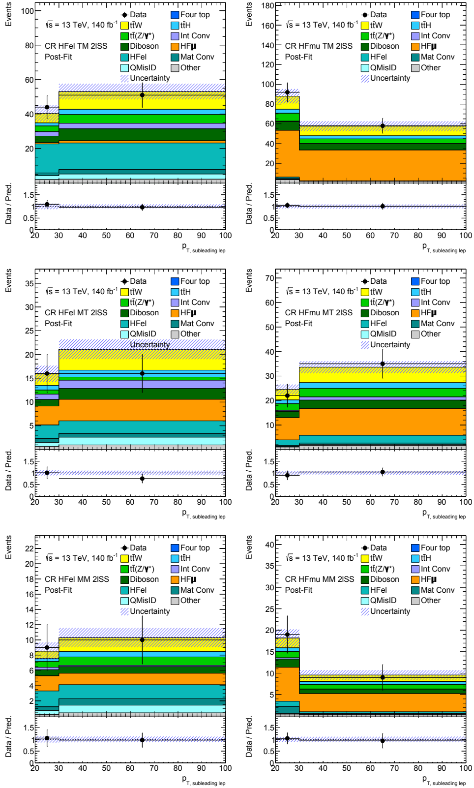
Figure 5.17: Post-fit distributions in the HF -CRs of the variables used in the background-only fit performed over the CRs and the unblinded bins of the SRs. The blue hashed band includes both statistical and systematic uncertainties. The bottom panels display the ratio between observed and expected event yields, used to assess the post-fit data/MC agreement.
