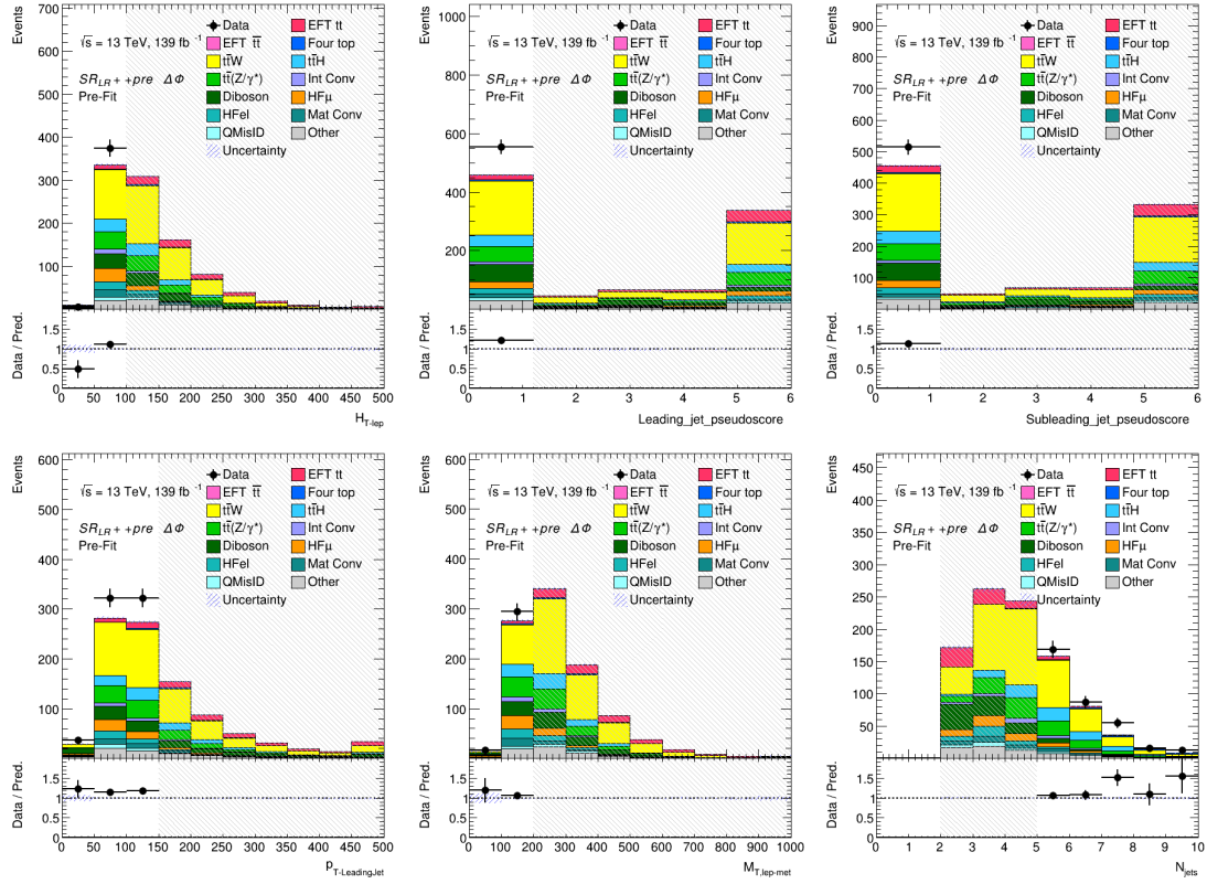
Figure E.16: Kinematic distributions for data and MC events in the \Delta\Phi < 2.5 region related to the 6 input variables of \text{NN}^{\text{SvsB}} for events in SR_{LR}^{++} . From top left to bottom right: H_{T,leptons} , b-tagging score of the leading jet, b-tagging score of the subleading jet, p_{T,LeadingJet} , M_{T,lep-met} and n_{Jets} . The bottom panels display the ratio between data and MC yields. Data events are not shown in bins where S/B \geq 5\% .
