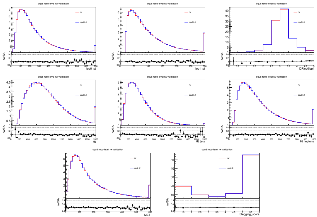
Figure C.17: Reco-level reweighting validation related to the additional tt sample generated with c_{LR}^{(8)} = 0.1 , c_{RR} = c_{LR}^{(1)} = 0
