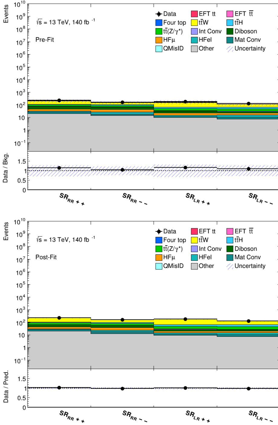
Figure 5.38: Summary of the pre-fit and post-fit data and MC yields in the analysis SRs. The post-fit yields are related to the fit performed on Run 2 data. The blue hashed bands include both statistical and systematic uncertainties. The bottom panels display the ratio between data and MC yields.
