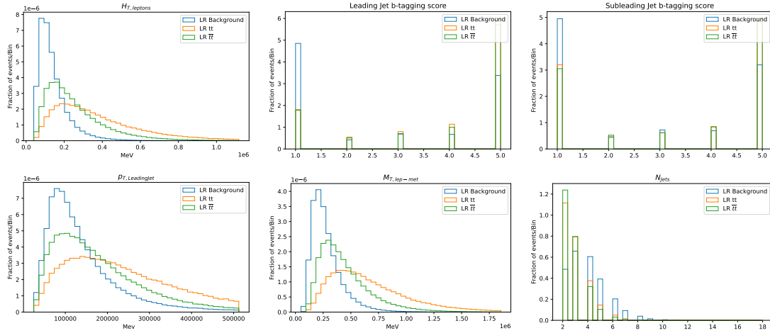
Figure E.11: Kinematic distributions related to the 6 input variables of NN^{SvsB} for events in SR_{LR} . From top left to bottom right: H_{T,leptons} , b-tagging score of the leading jet, b-tagging score of the subleading jet, p_{T,LeadingJet} , M_{T,lep-met} and n_{Jets} . The distributions related to tt , t\bar{t} and background events are reported in orange, green and blue respectively. All distribution are normalized to unity.
