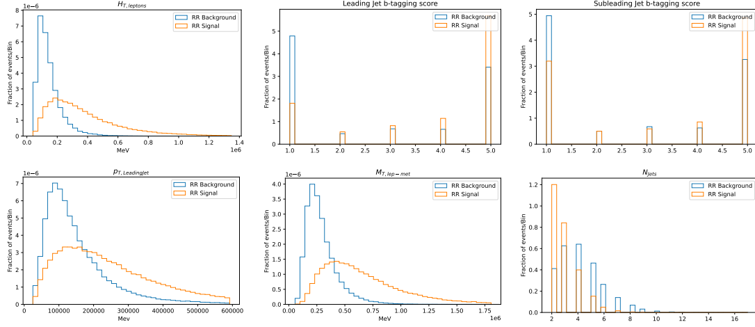
Figure E.5: Kinematic distributions related to the 6 input variables of NN^{SvsB} for events in SR_{RR} . From top left to bottom right: H_{T,leptons} , b-tagging score of the leading jet, b-tagging score of the subleading jet, p_{T,LeadingJet} , M_{T,lep-met} and n_{Jets} . Signal and background distributions are reported in orange and blue respectively. All distribution are normalized to unity.
