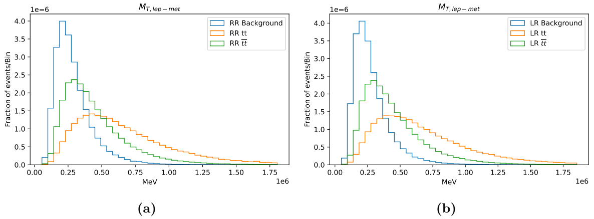
Figure 5.5: Normalized distribution of the NN^{\text{SvsS}} input variable M_{T,lep-met} for SR_{RR} (a) and SR_{LR} (b). The distributions related to tt , t\bar{t} and background events are reported in orange, green and blue respectively.
