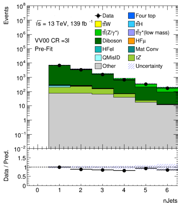
Figure F.1: Jet multiplicity distribution of data and simulated events in the defined VV00 CR without the b -jet selection requirement. It can be noticed that the t\bar{t}Z contribution is not negligible at high multiplicity.
