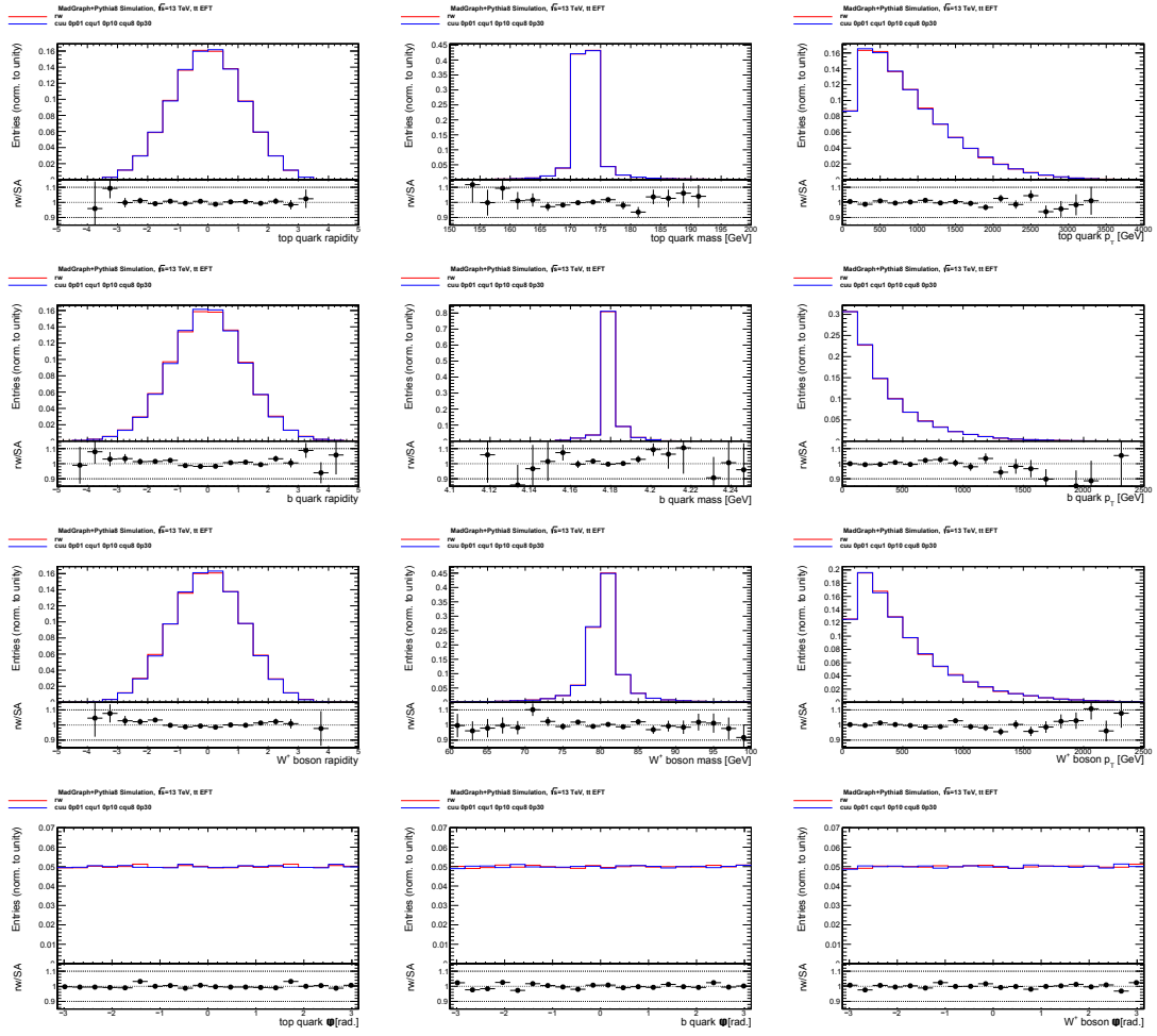
Figure C.12: Truth-level reweighting validation related to the additional tt sample generated with c_{RR} = 0.01 , c_{LR}^{(1)} = 0.1 , c_{LR}^{(8)} = 0.3 . The red and blue lines show the distribution resulting from the nominal and the reweighted samples respectively. All distributions are normalized to unity. The bottom panels show the ratio between the nominal and reweighted sample entries.
